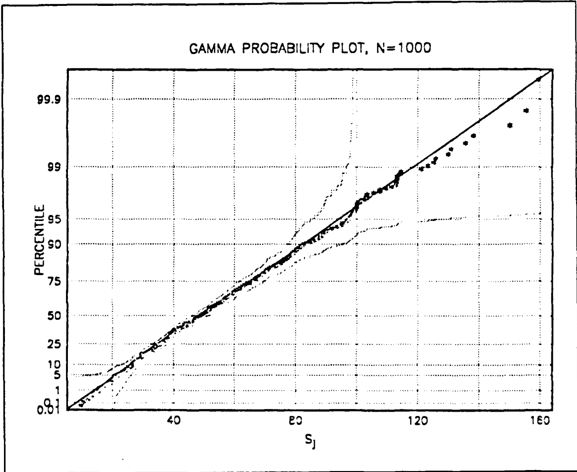
Figure C1. Probability Plot
