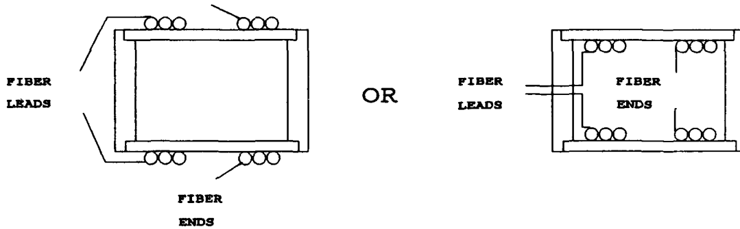
Figure 2.4b Two fiber coil push-pull accelerometer using two disks.
