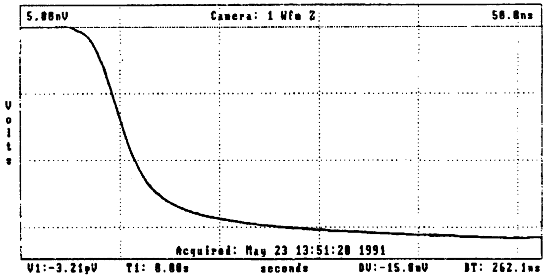
Figure 3.5. Integrated laser pulse of Figure 3.4.
