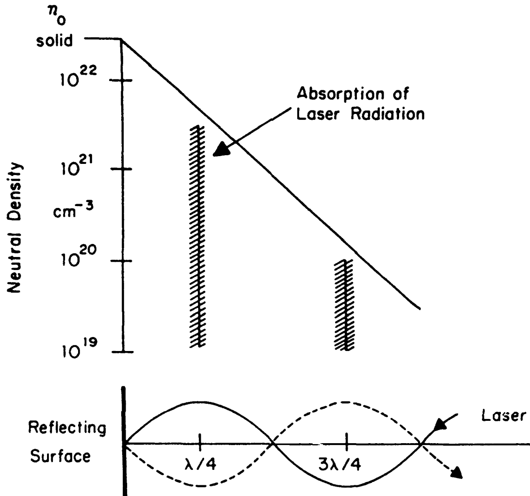
Figure 2.1. Absorption of laser radiation near a reflecting surface. The neutral density gradient in front of the surface is caused by blow-off of surface material. [Ref. 9]
