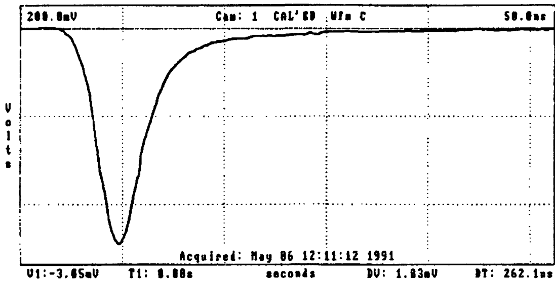
Figure 3.4. A typical laser pulse captured by DCS.
