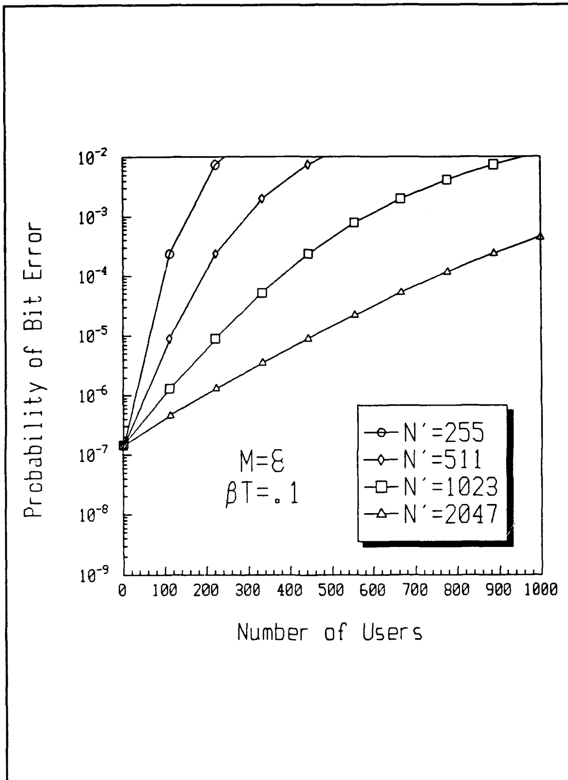
Figure 19 Performance of Coherent Optically Heterodyned MFSK-CDMA, M = 8 and \beta T = .1
