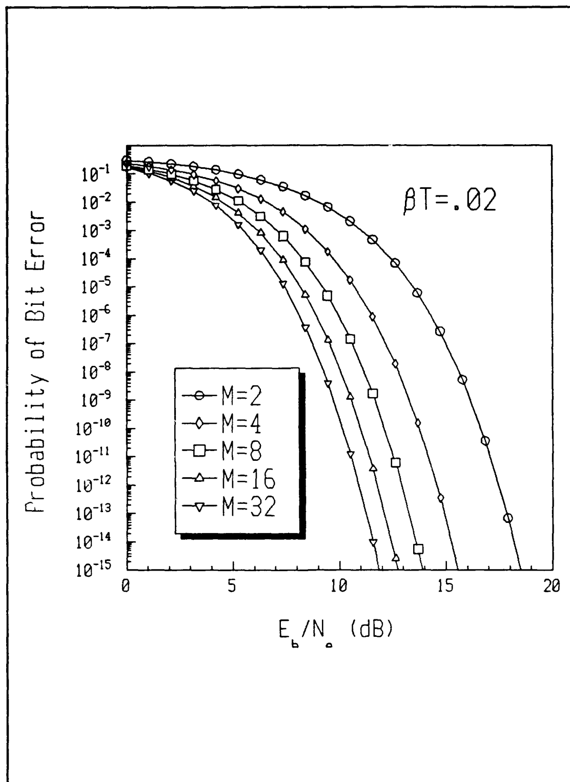
Figure 15 Performance of Coherent Optically Heterodyned MFSK, \beta T = .02
