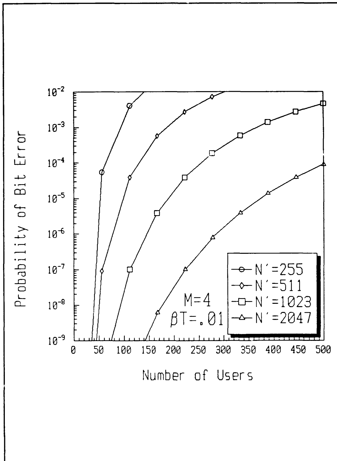
Figure 23 Performance of Coherent Optically Heterodyned MFSK-CDMA, M = 4 and \beta T = .01
