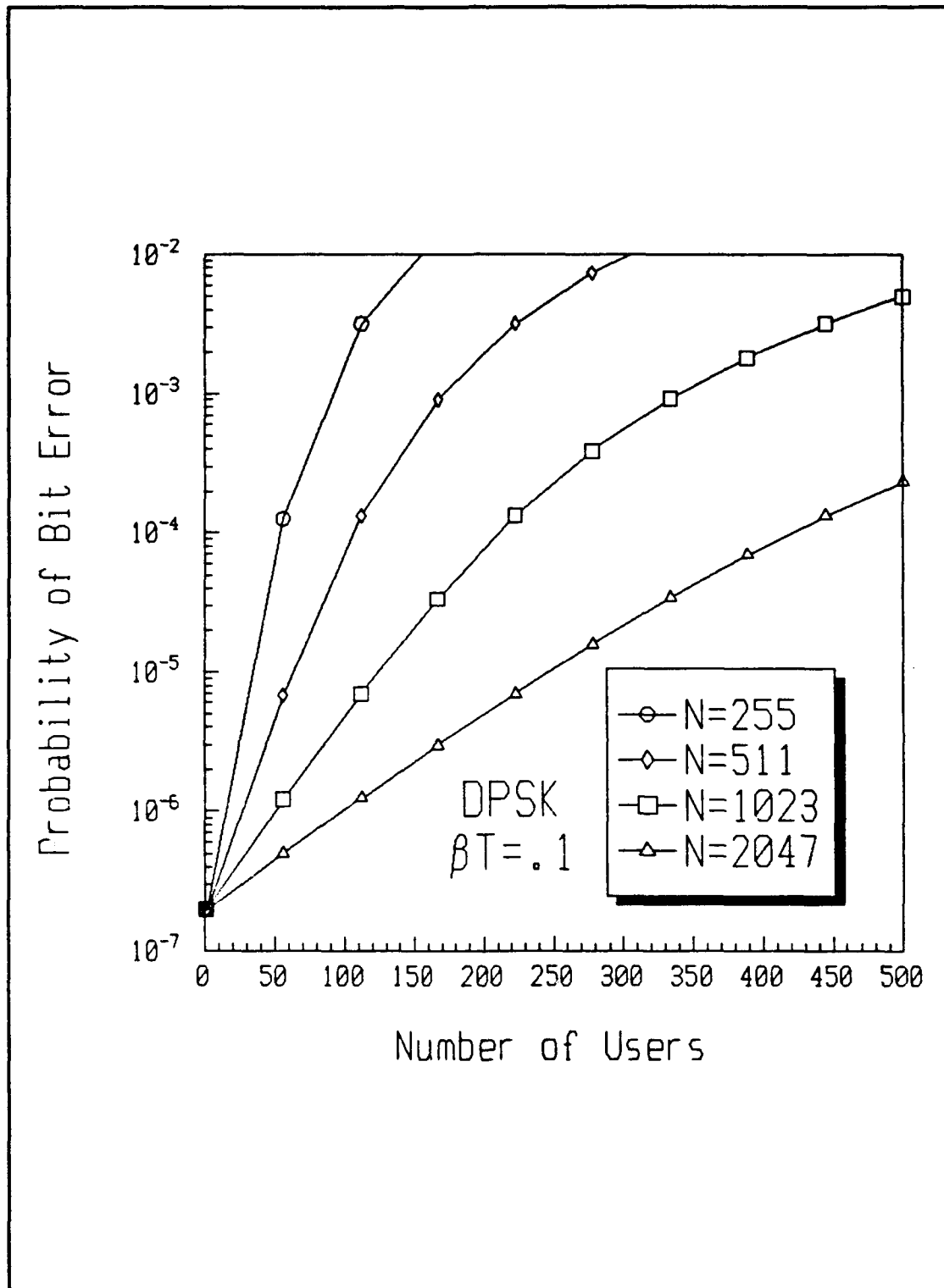
Figure 33 Performance of Coherent Optically Heterodyned DPSK, \beta T = .1
