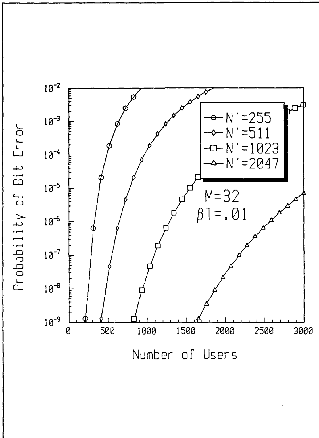
Figure 26 Performance of Coherent Optically Heterodyned MFSK-CDMA, M = 32 and \beta T = .01
