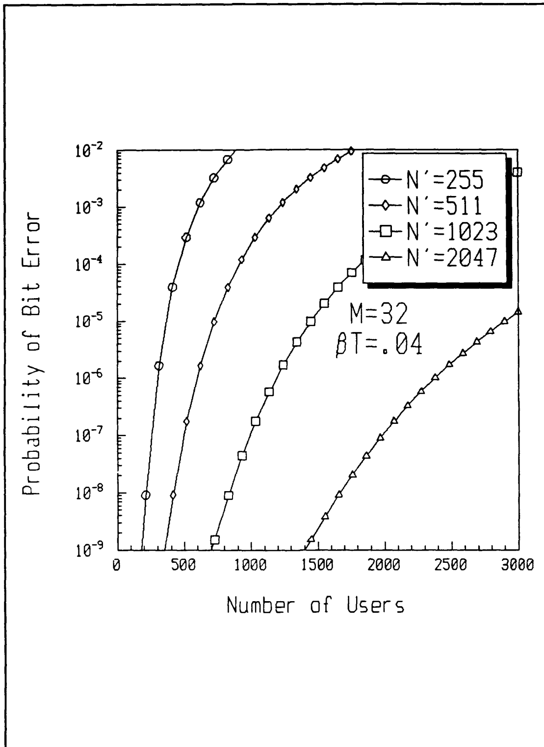
Figure 31 Performance of Coherent Optically Heterodyned MFSK-CDMA, M = 32 and \beta T = .04
