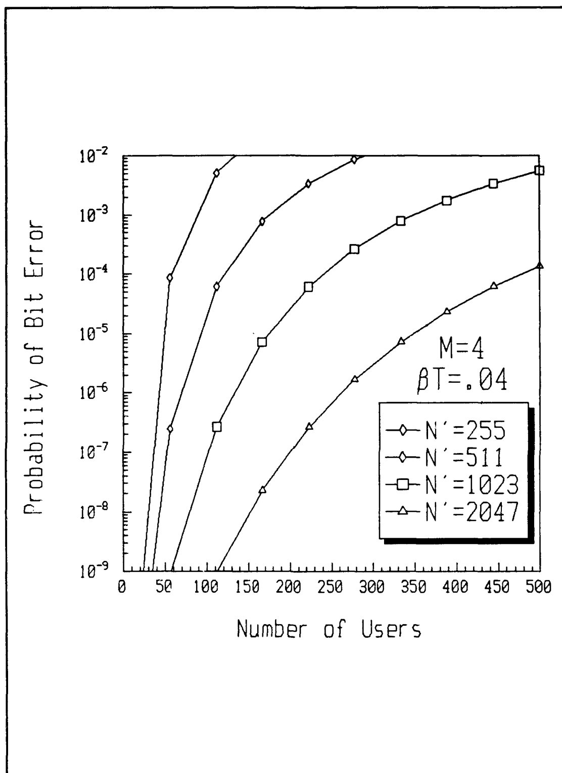
Figure 28 Performance of Coherent Optically Heterodyned MFSK-CDMA, M = 4 and \beta T = .04
