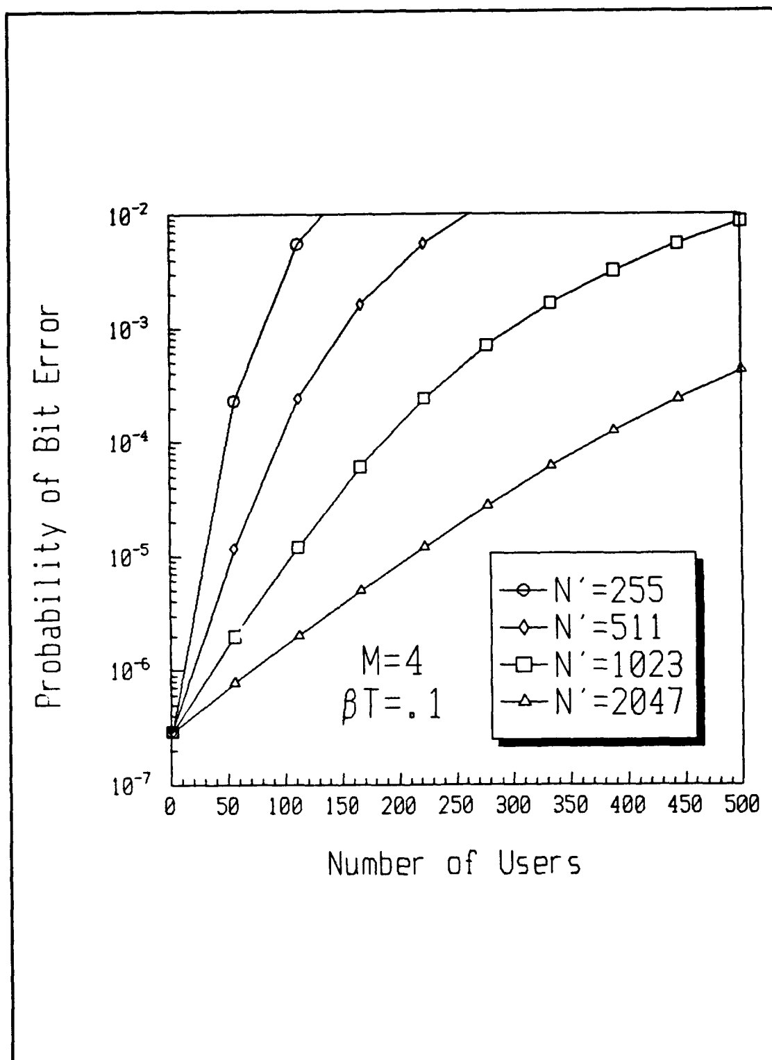
Figure 18 Performance of Coherent Optically Heterodyned MFSK-CDMA, M=4 and \beta T = .1
