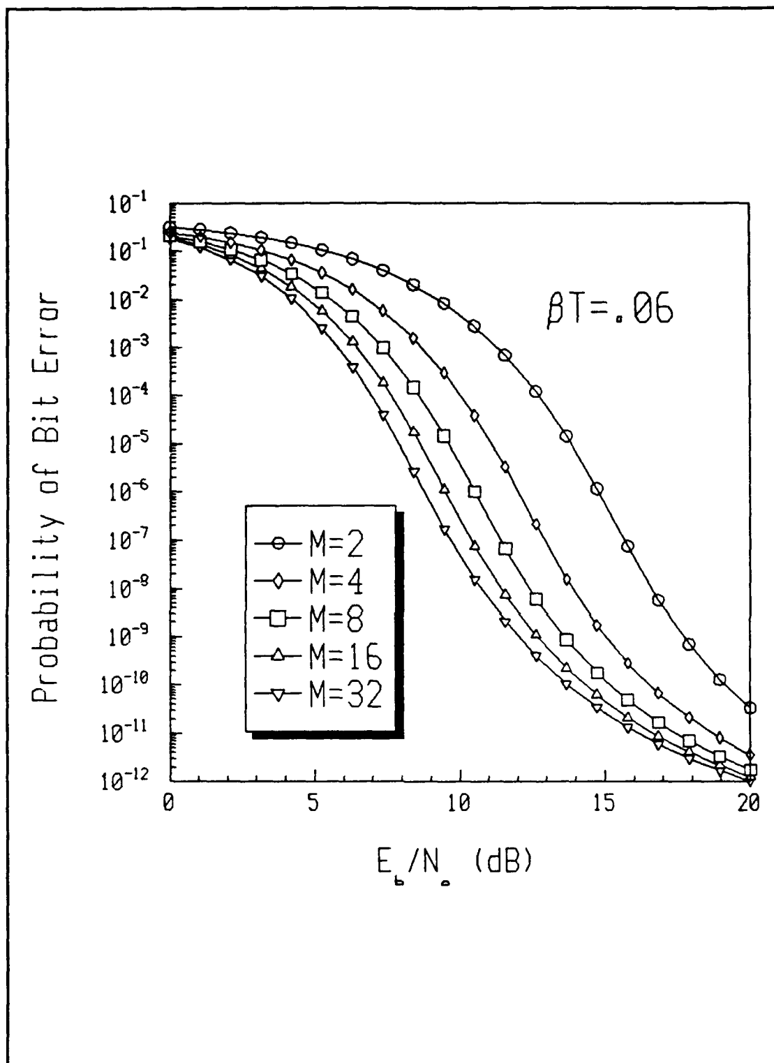
Figure 13 Performance of Coherent Optically Heterodyned MFSK, \beta T = .06
