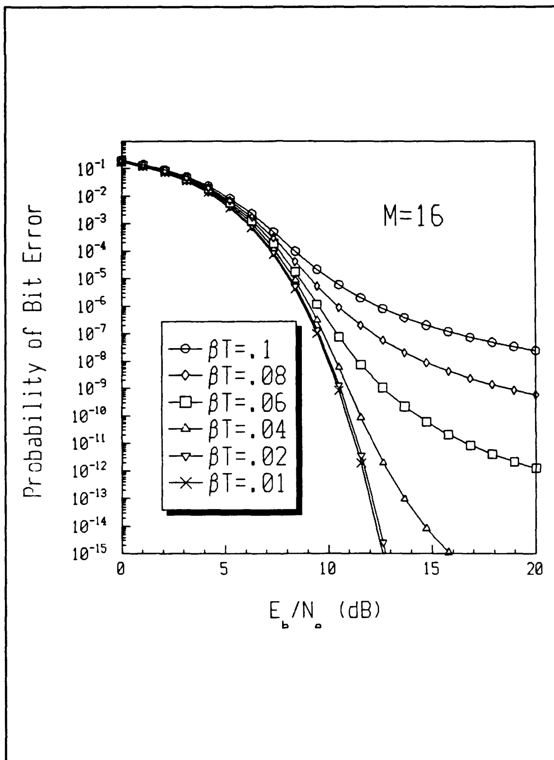
Figure 9 Performance of Coherent Optically Heterodyned MFSK, M = 16
