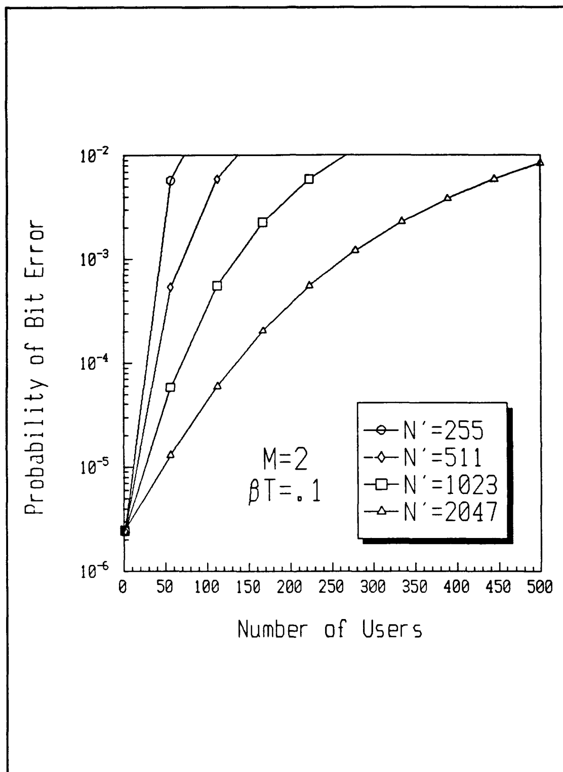
Figure 17 Performance of Coherent Optically Heterodyned MFSK-CDMA, M=2 and \beta T = .1
