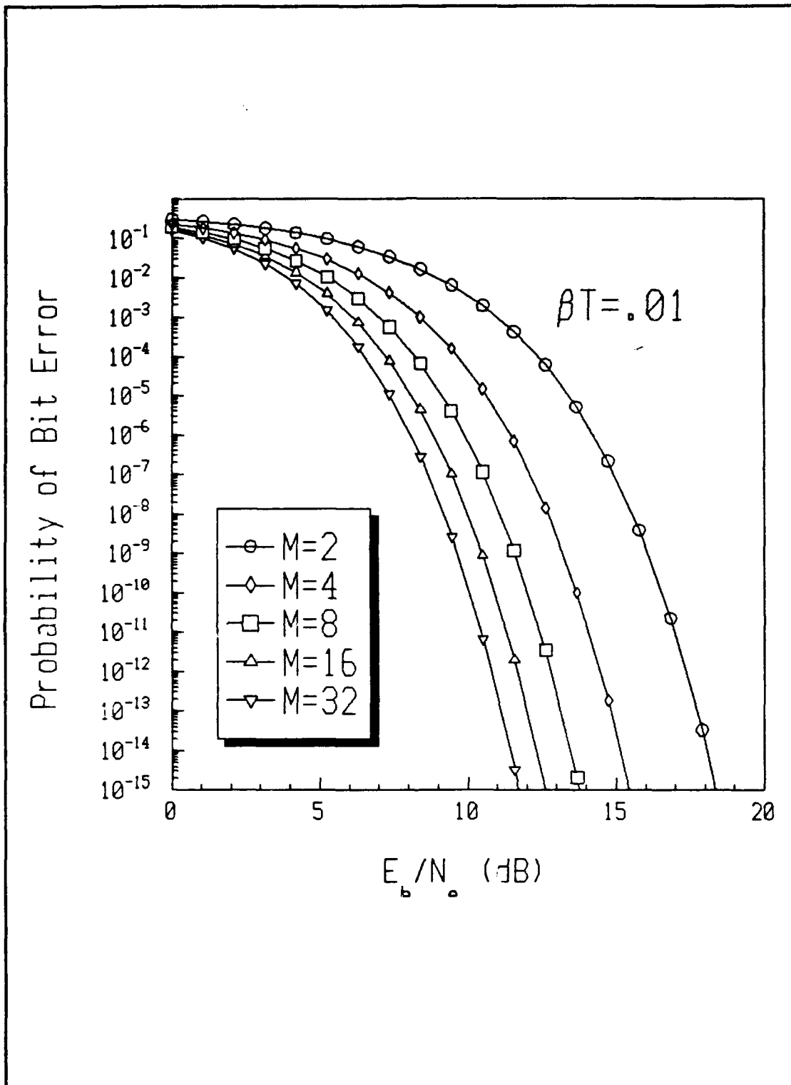
Figure 16 Performance of Coherent Optically Heterodyned MFSK, \beta T = .01
