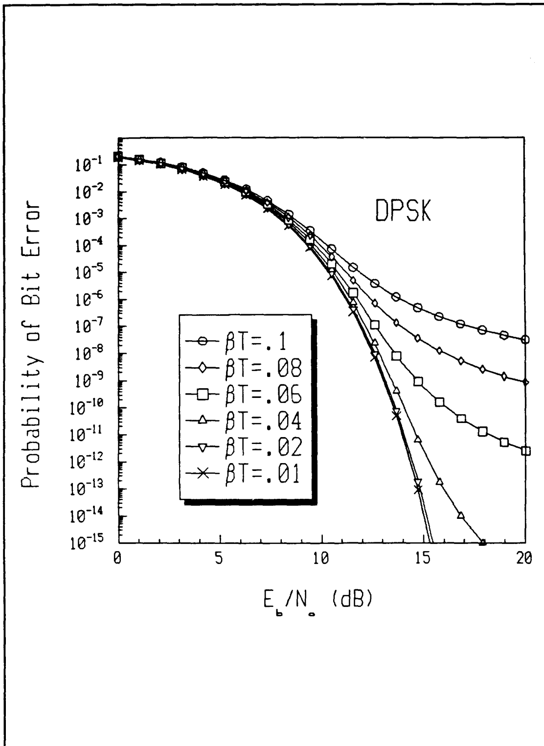
Figure 32 Coherent Optically Heterodyned DPSK Performance
