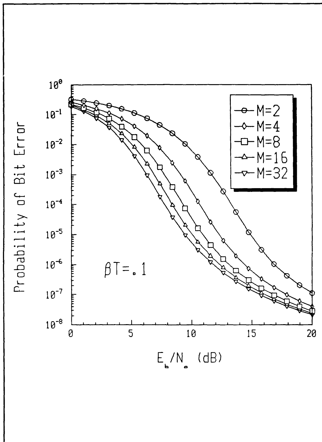
Figure 11 Performance of Coherent Optically Heterodyned MFSK, \beta T = .1
