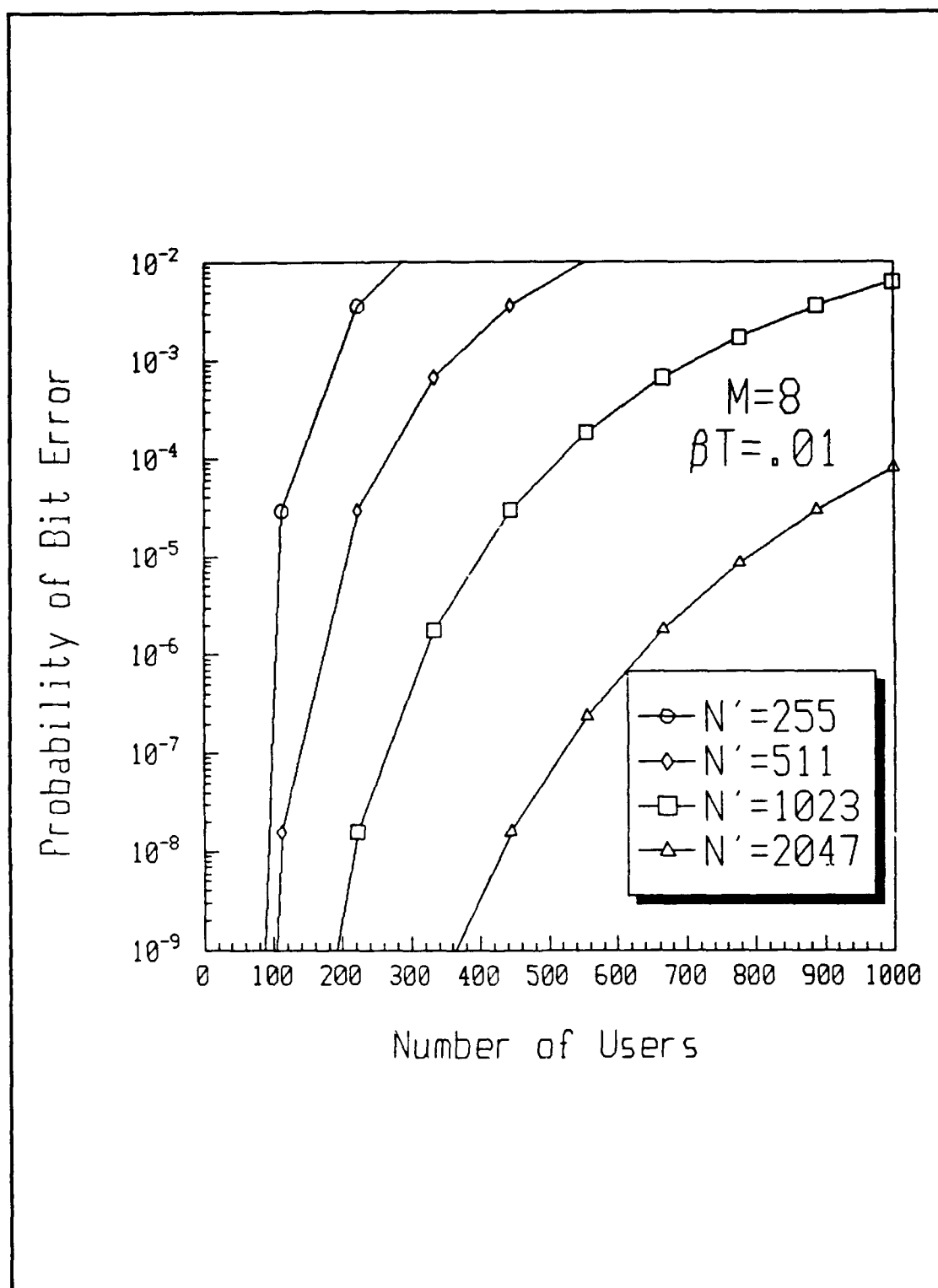
Figure 24 Performance of Coherent Optically Heterodyned MFSK-CDMA, M = 8 and \beta T = .01
