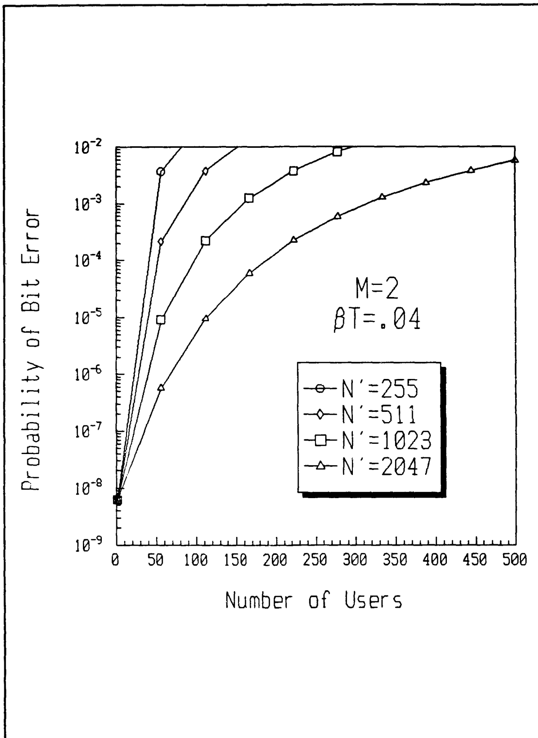
Figure 27 Performance of Coherent Optically Heterodyned MFSK-CDMA, M = 2 and \beta T = .04
