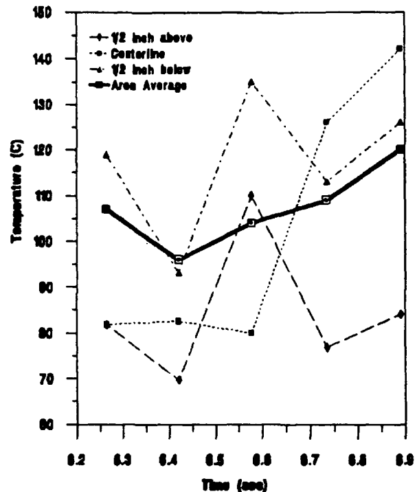
FIGURE A-9: TEST-12: Plume Temperature At 16.7 Nozzle Diameters From The Nozzle Exit (Based On An Emissivity=1)
