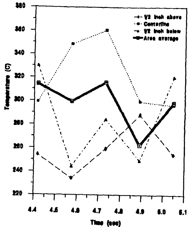
FIGURE A-22: TEST-20: Plume Temperature At 16.7 Nozzle Diameters From The Nozzle Exit (Based On An Emissivity=1)
