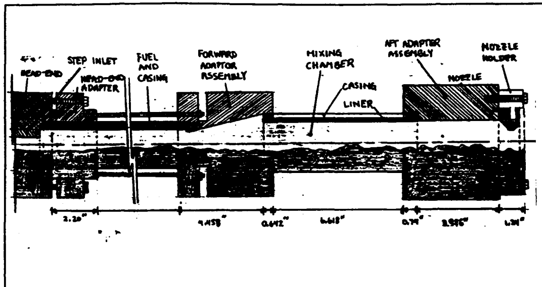
FIGURE 10: Ramjet Configuration
