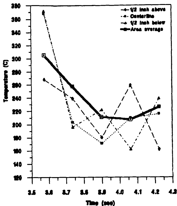
FIGURE A-28: TEST-23: Plume Temperature At 16.7 Nozzle Diameters From The Nozzle Exit (Based On An Emissivity=1)
