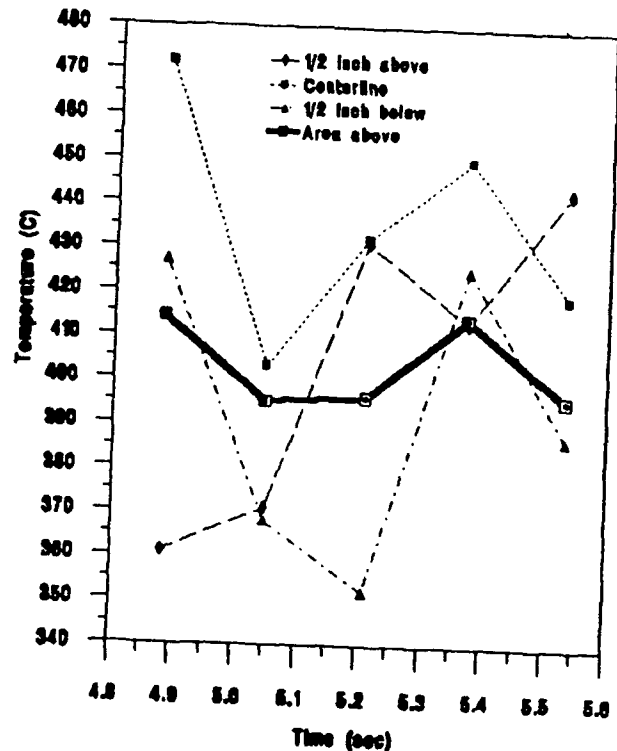
FIGURE A-20: TEST-19: Plume Temperature At 10.7 Nozzle Diameters From The Nozzle Exit (Based On An Emissivity=1)
