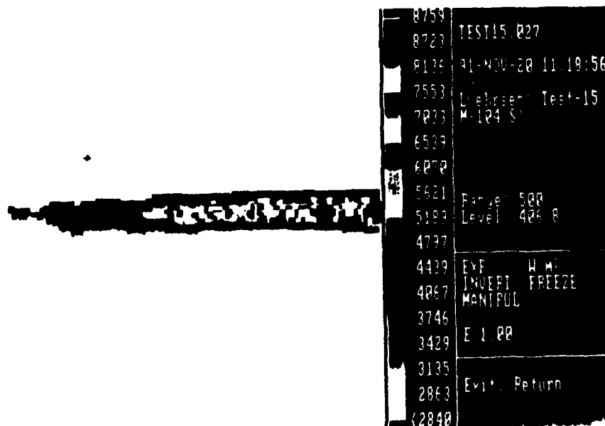
FIGURE A-13: TEST-15: IR Plume Representation
