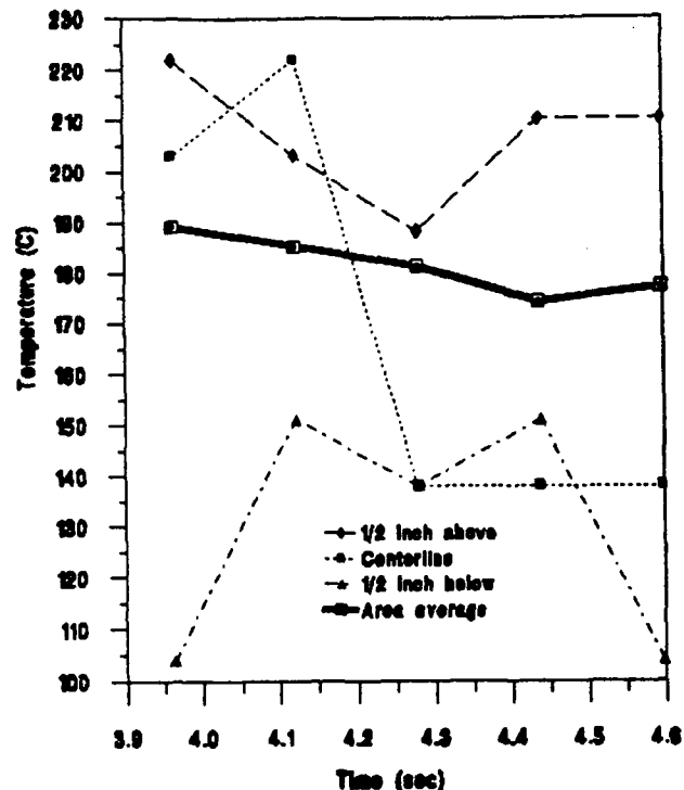
FIGURE A-26: TEST-22: Plume Temperature At 18.7 Nozzle Diameters From The Nozzle Exit (Based On An Emissivity=1)
