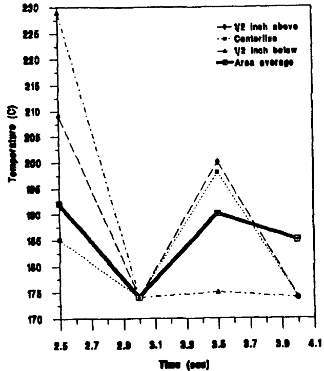
FIGURE A-14: TEST-16: Plume Temperature At 10.7 Nozzle Diameters From The Nozzle Exr (Based On An Emissivity=1)
