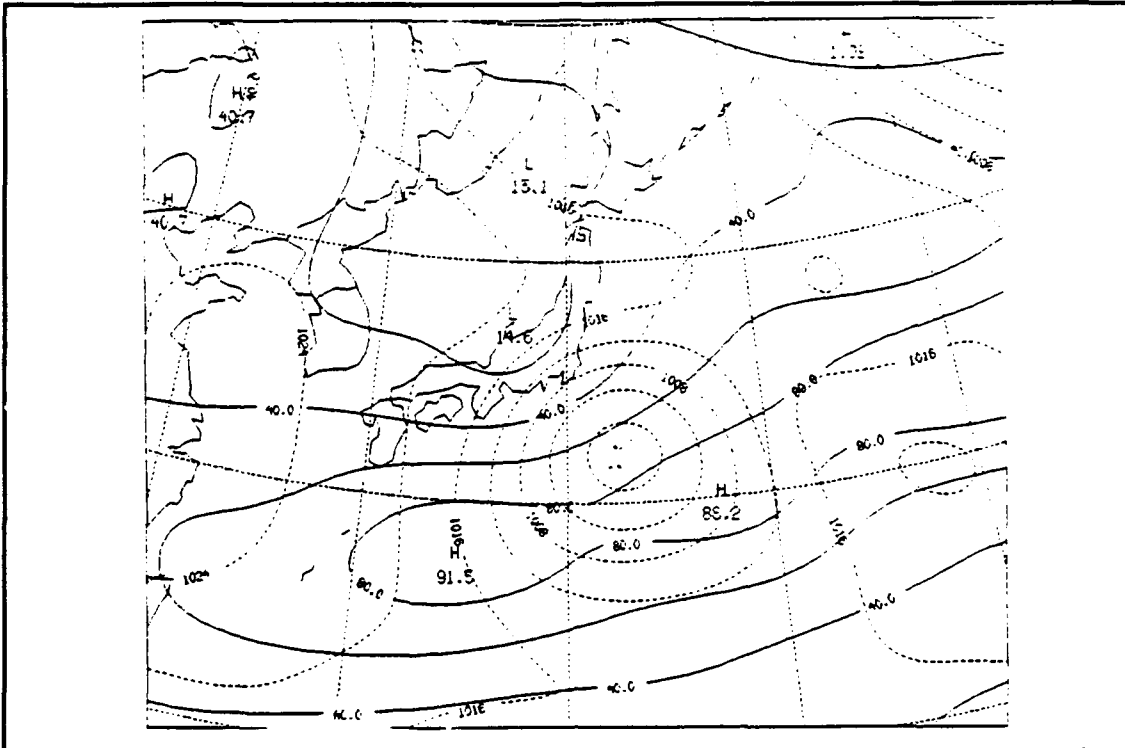
Figure 18. 1200Z UTC 11 February 1986 Upper-Level Analysis: Same as Fig. 4.
