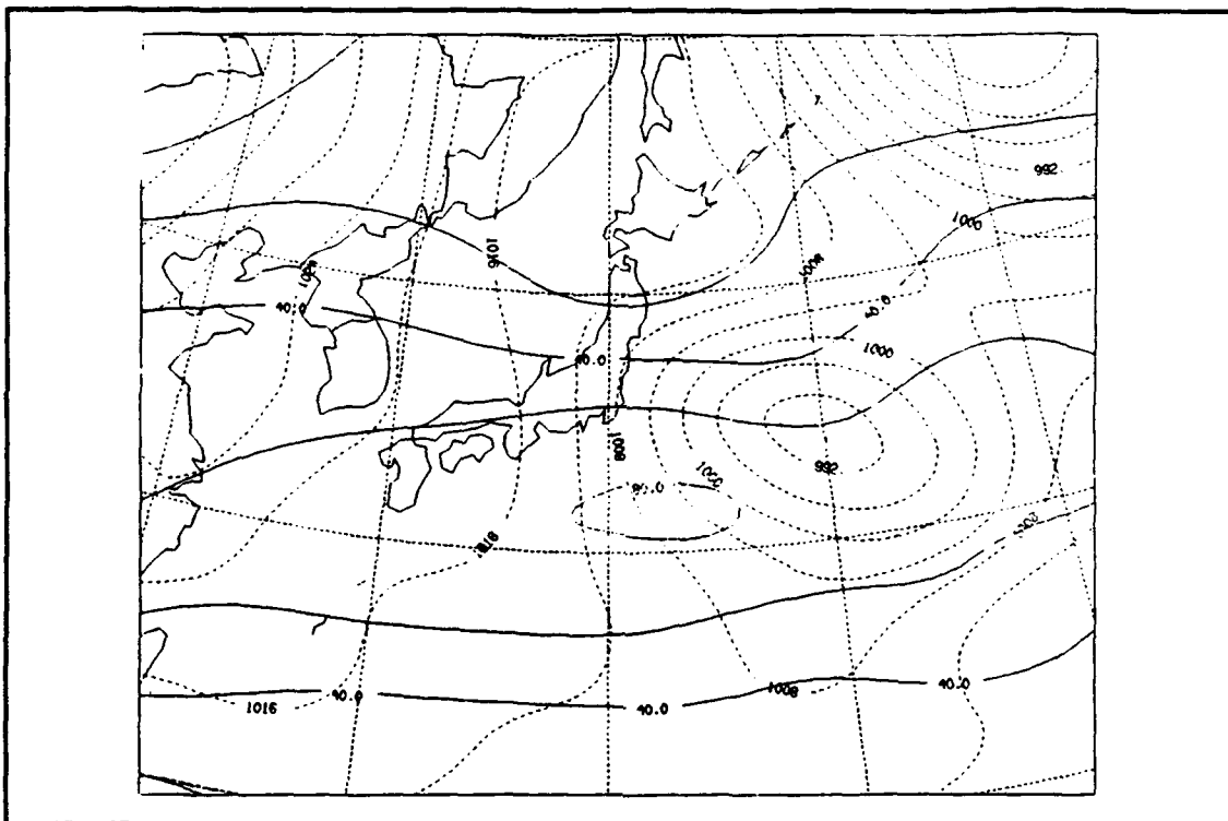
Figure 12. 1200Z UTC 19 February 1986 Upper-Level Analysis: Same as Fig. 4.
