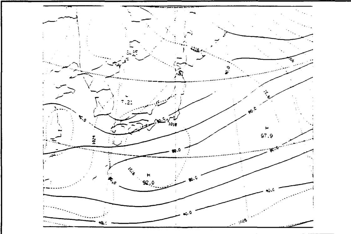
Figure 15. 0000Z UTC 11 February 1986 Upper-Level Analysis: Same as Fig. 4.
