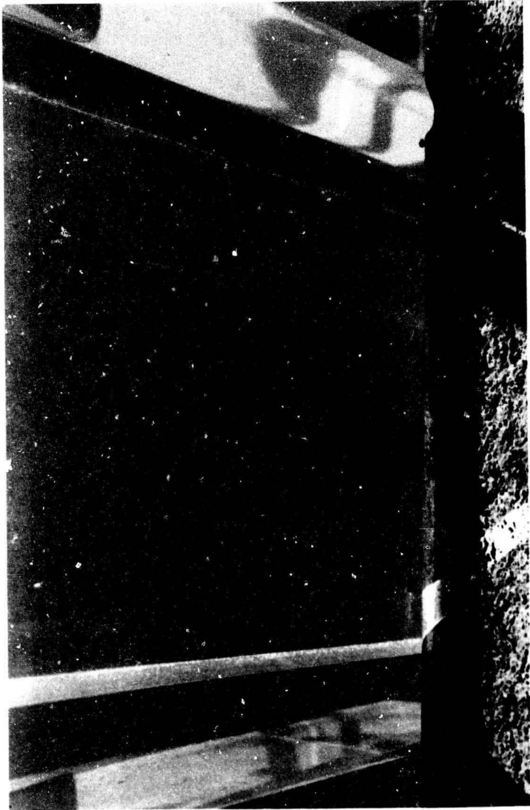
Figure 17. Note the absence of crazing on test beam No. 4 after 5 years of sustained flexure loading as a cantilever beam; the flexure stress above the fulcrum is 1200 psi. The beam was photographed from below.
