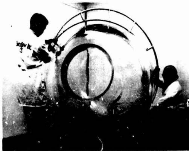
Figure 10. Checking the dimensions of a finished 66 inch diameter NEMO hull.
