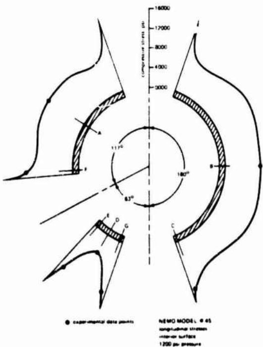
Fig. 15 Distribution of longitudinal stresses on the interior surface of model scale NEMO sphere #45 under 1200 psi external hydrostatic loading. Note that the highest stresses are at the edges of penetrations
