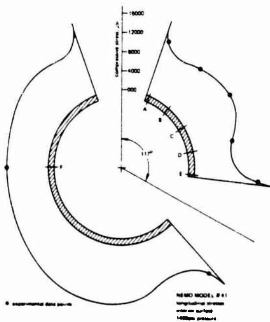
Fig. 12 Distribution of longitudinal stresses on the exterior surface of model scale NEMO sphere # 41. Note that the highest stresses are at the edges of penetrations. Magnitude of hydrostatic loading was 1400 psi
