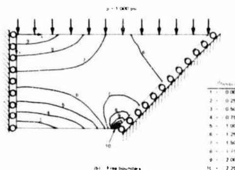
Fig. 18 Plot of \sigma_{hoop} stress contours in a U/D_1 = 0.46 plane disk with single conical bearing surface
