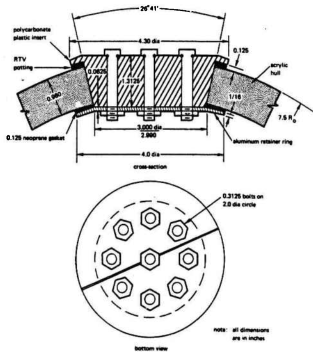
Fig. 3 15 \times 13-inch NEMO Model #36, imploded at 4350 psi under short term pressurization with tap water at 75°F
