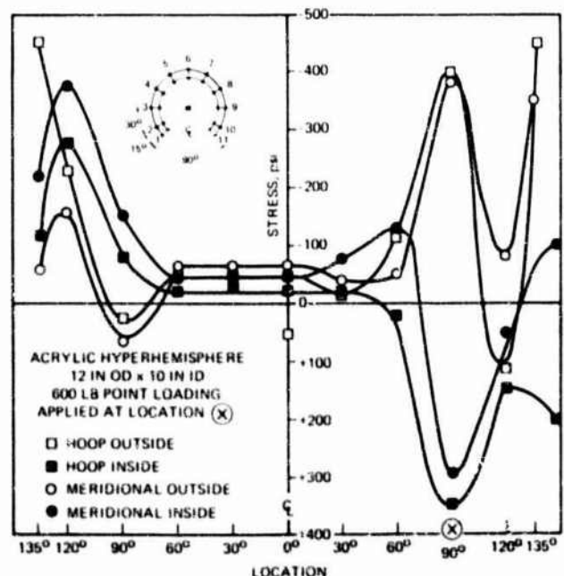
Fig. 9 Stresses in acrylic window under point loading applied to its equator
