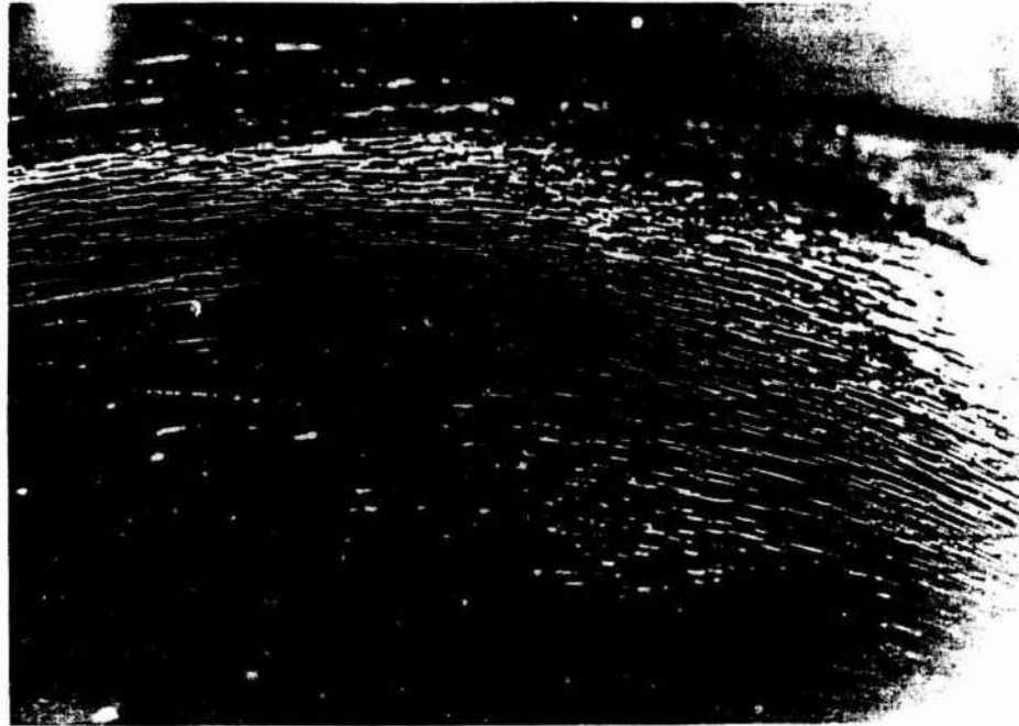
Fig. 6 Crazing, typical of the weathered surface on the 10-year-old NEMO Model #37
