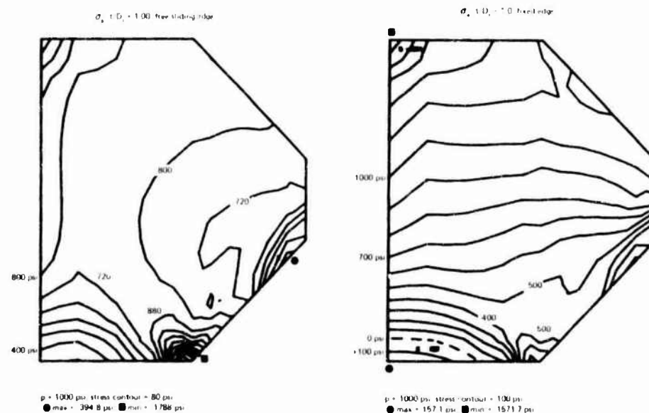
Fig. 25 Plot of \sigma_x stress contours in a t/D_i = 1.0 plane disk with twin conical bearing surfaces
