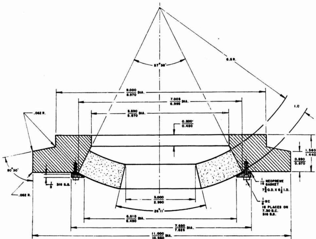
Fig. 5 Dimensions of the spherical sector test fixture shown in Fig. 4
