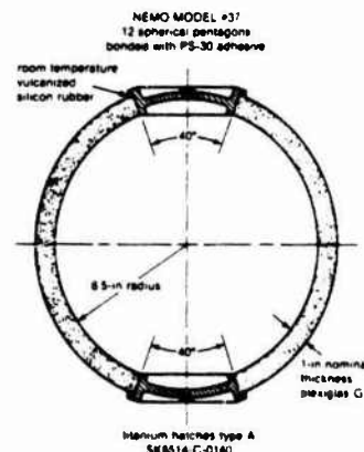
Fig. 5 NEMO Model #37 assembly, imploded at 4200 psi under short-term loading
