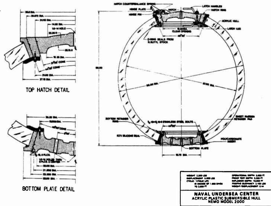
Fig. 1 Design characteristics of Navy's NEMO Model 2000 for 3000 ft operational depth (For further details see references [5] and [16])
