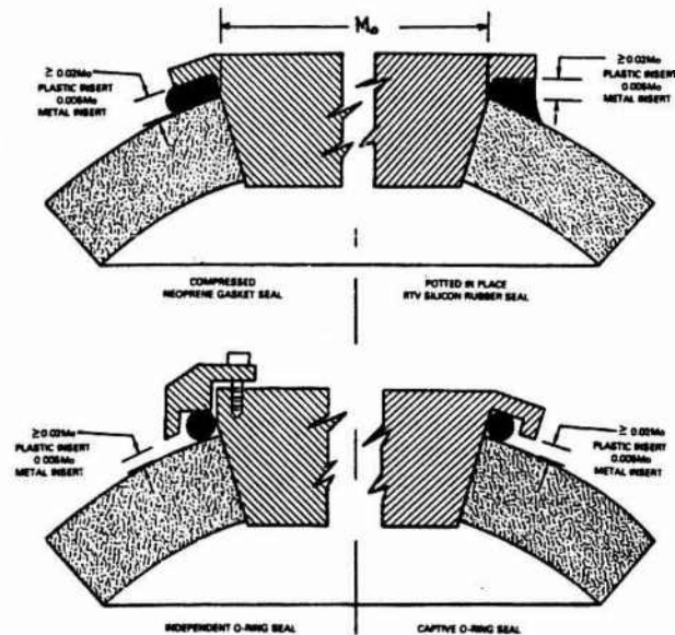
Fig. 10 Typical sealing arrangements for inserts
