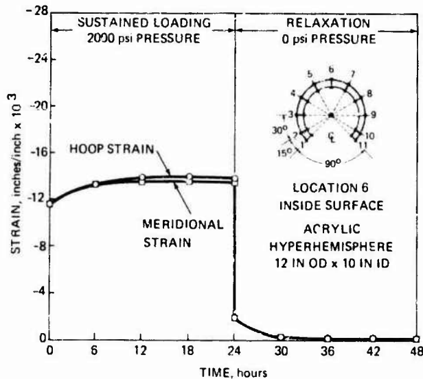
Fig. 15 Membrane strain at the apex of the acrylic hyperhemisphere under long term hydrostatic loading. Note that there is very little creep at this location, and that it is of the same magnitude in both meridional and hoop directions.
