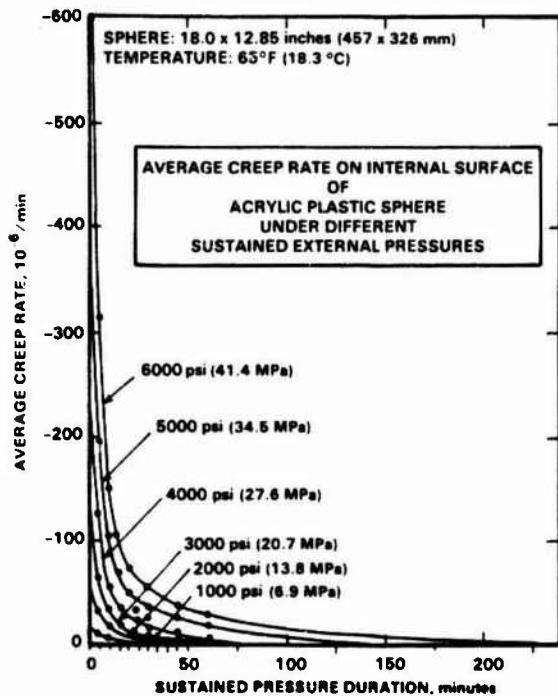
Fig. 6 Creep (time-dependent strain rate) on the concave surface of Model AA under sustained pressure loading
