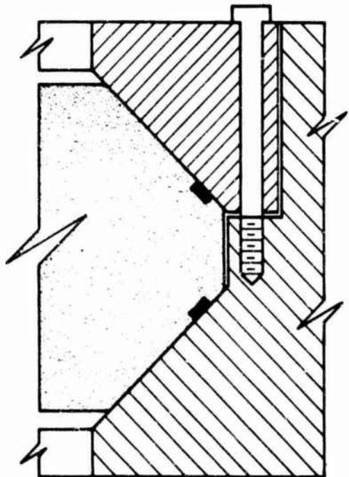
Fig. 2 Sealing arrangement for twin bevel disks utilizing axially compressed O-rings located in the bearing surfaces of the window. It is not a recommended design as the O-ring grooves in the bearing surfaces decrease significantly the fatigue life of the window
