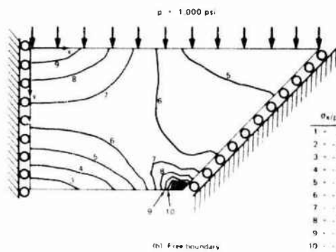
Fig. 16 Plot of \sigma_r stress contours in a U/D_1 = 0.46 plane disk with single conical bearing surface
