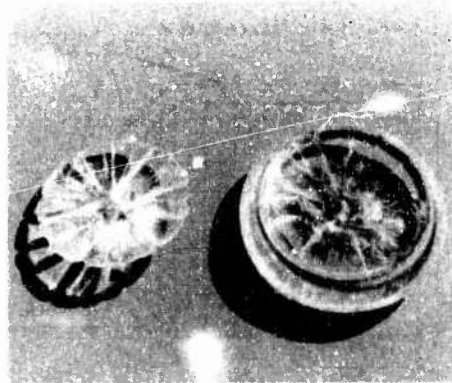
Fig. 11 Fracture surface on a twin bevel plane disk after short term hydrostatic loading to fracture initiation; t/D_1 = 0.32 , D_0 = 4 in., test pressure = 9300 psi, \alpha = 90 deg
