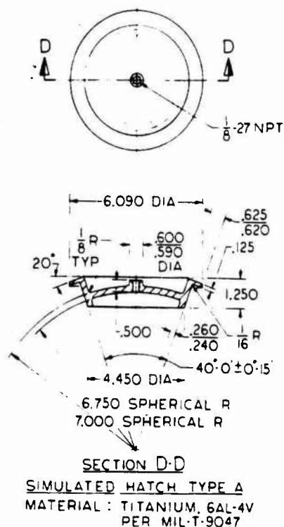
Fig. 4 Titanium hatches for NEMO Model #37
