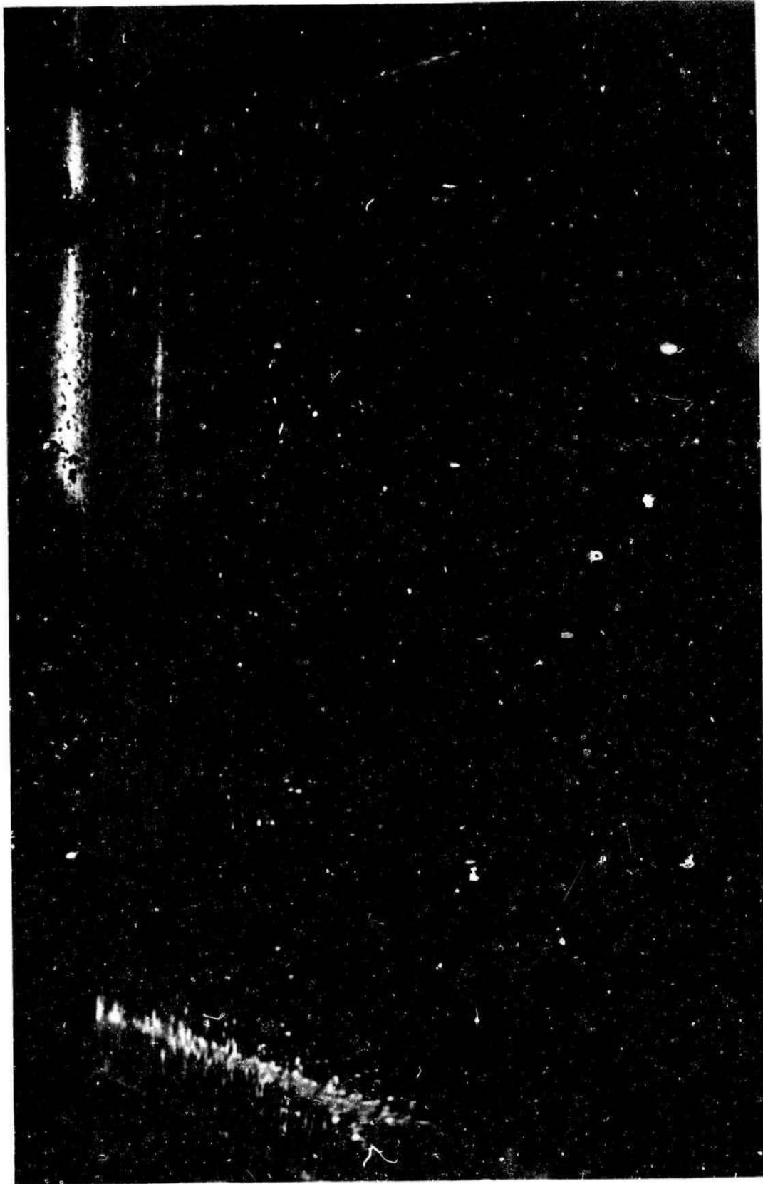
Figure 15. Crazing on the upper surface of the 4- by 48- by 2-inch-thick test beam No. 2 after 5 years of sustained flexure loading as a cantilever beam; the crazing was photographed from below the beam.
