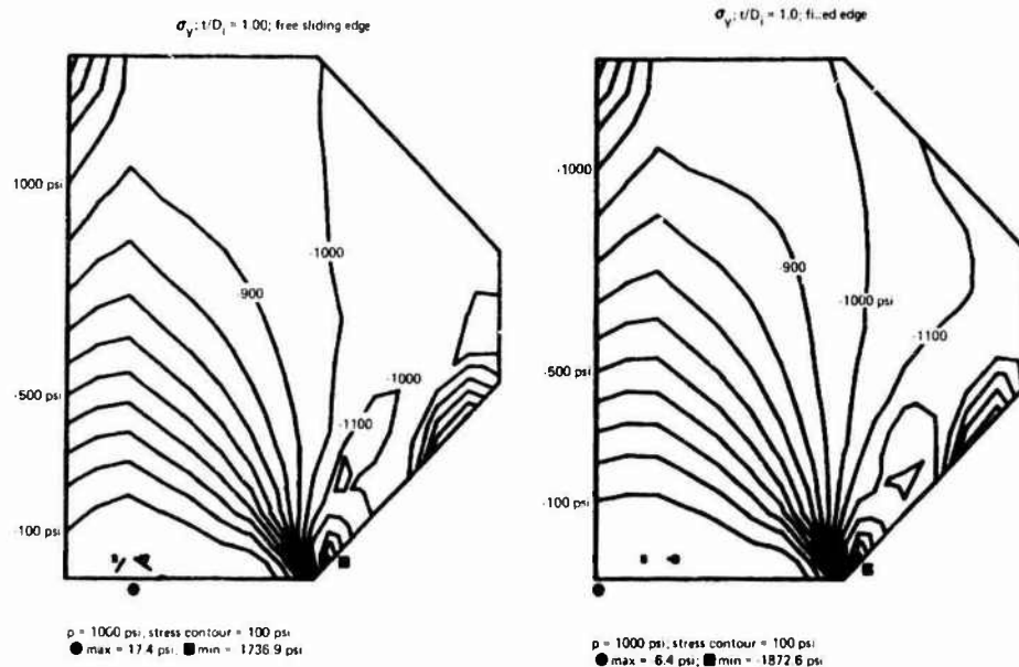
Fig. 26 Plot of \sigma_r stress contours in a t/D_1 = 1.0 plane disk with twin conical bearing surfaces
