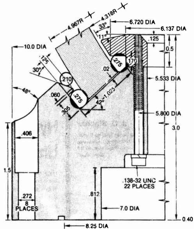
Fig. 3 Typical hyperhemispherical viewport assembly design for containment of electro-optical systems on submarines. The extent of O-ring deformation after tightening of holddown screws is shown by dark areas on the O-ring cross-sections.
