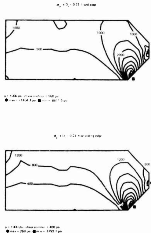
Fig. 23 Plot of \sigma_t stress contours in a l/D_1 = 0.23 plane disk with twin conical bearing surfaces
