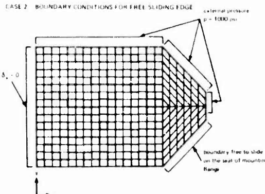
Fig. 15 Boundary conditions used in the finite element stress analysis of plane disks with twin conical bearing surfaces
