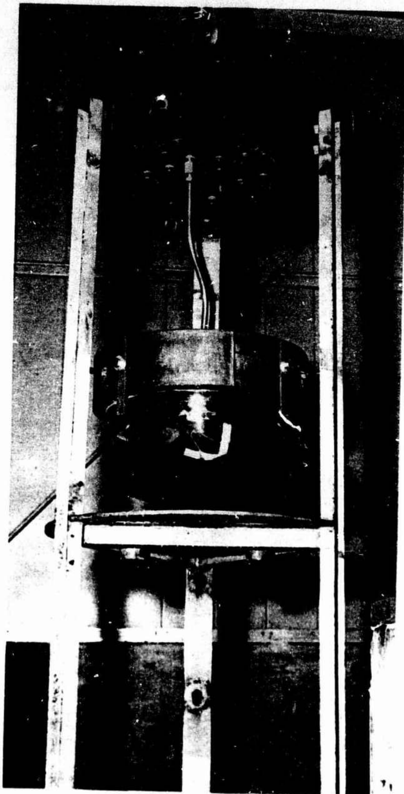
Figure 11. Test arrangement for long-term and cyclic-pressure testing of cast spherical windows. Note tube used for venting interior of hemisphere to ambient atmosphere outside the pressure vessel.
