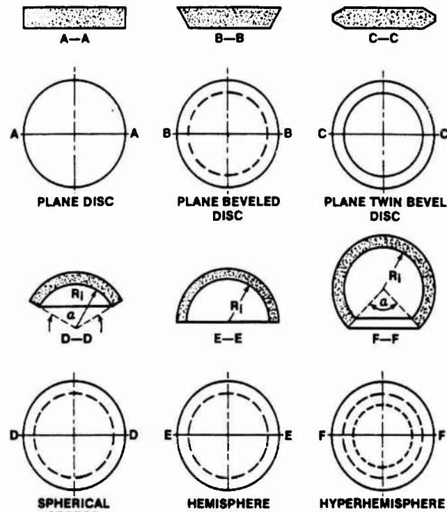
Fig. 2 Typical shapes of windows for pressure-resistant viewports
