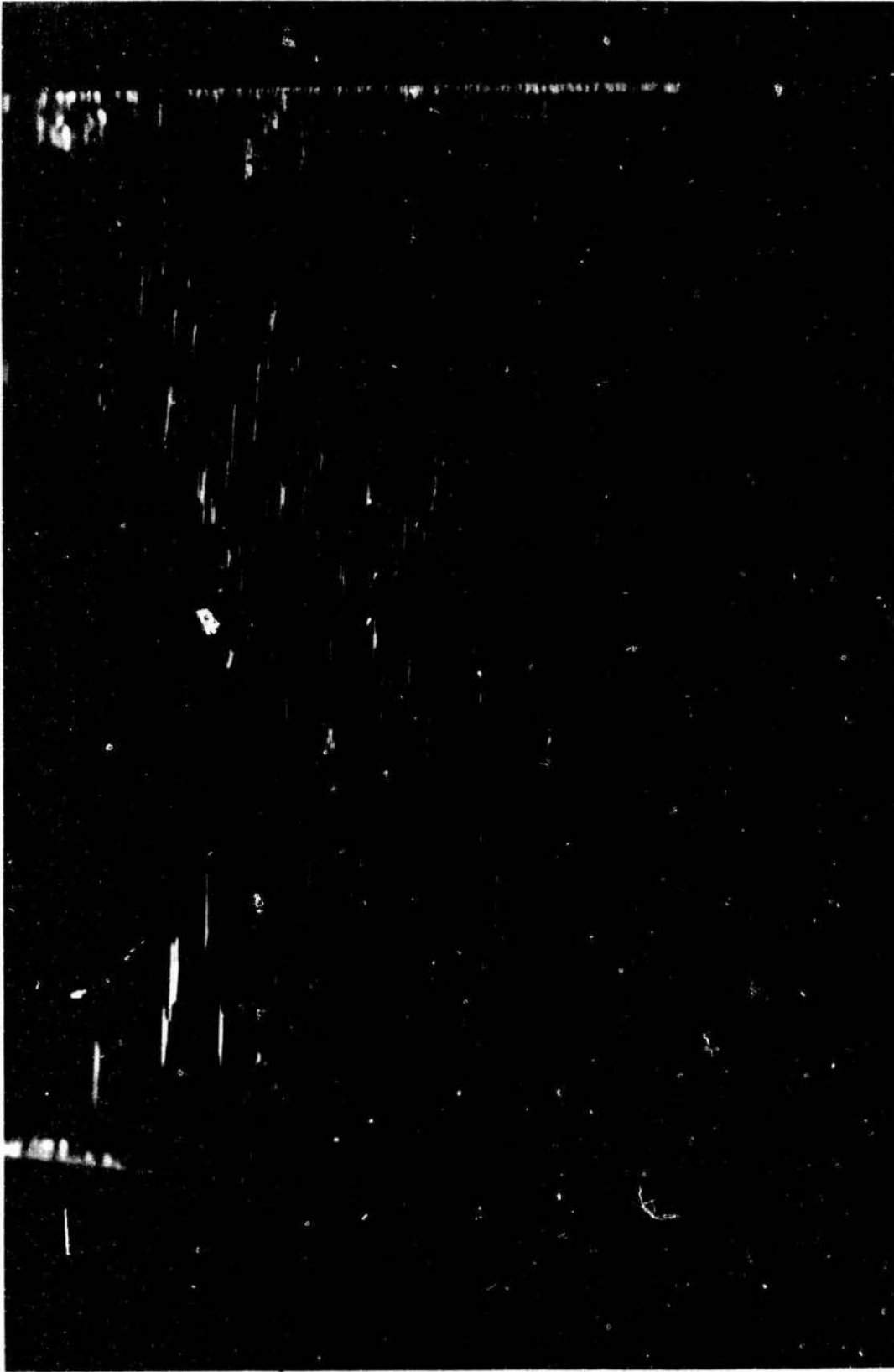
Figure 10. Crazing of the upper surface on the 2- by 22- by 0.25-inch-thick flexure specimen after 20 minutes of sustained 2000-psi flexure stress and continuous wetting by ethyl alcohol. Note that the crazing is oriented at right angles to the direction of principal flexure stress.
