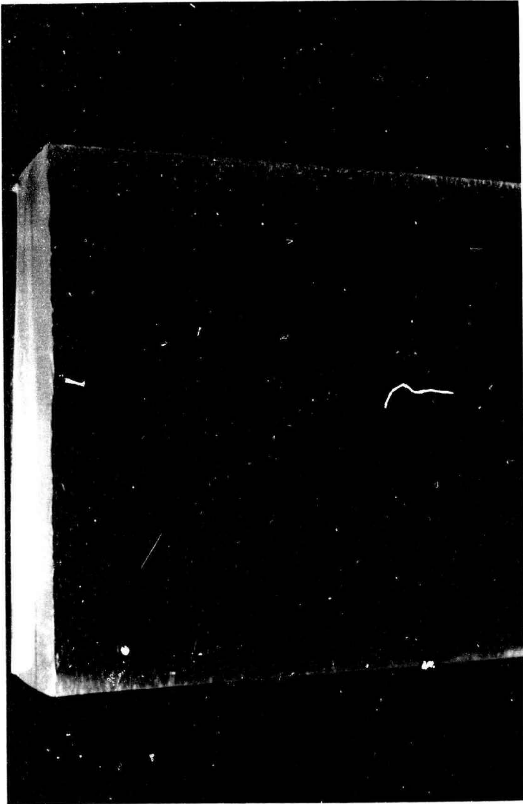
Figure 19. Crazeing on test beam No. 1 after 9 years of sustained flexure loading as a cantilever beam. The stress above the fulcrum was 2240 psi.
