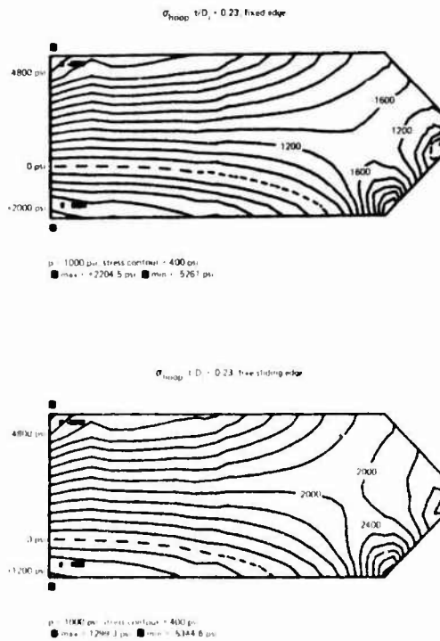
Fig. 24 Plot of \sigma_{hoop} stress contours in a t/D_i = 0.23 plane disk with twin conical bearing surfaces
