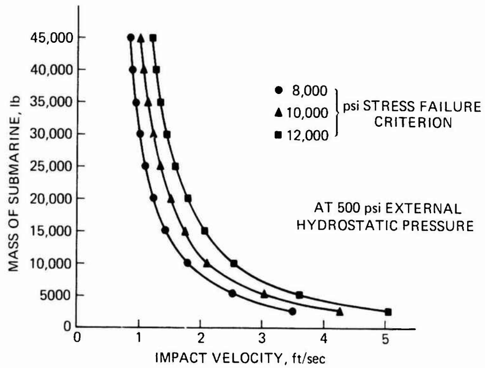
Figure 57. Critical impact velocities for 2.25-inch thick windows mounted on submersibles of different mass operating in 500 psi ambient pressure environment.
