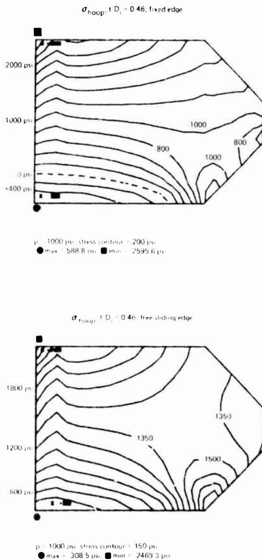
Fig. 21 Plot of \sigma_{hoop} stress contours in a l/D_1 = 0.46 plane disk with twin conical bearing surfaces
