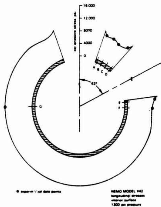
Fig. 13 Distribution of longitudinal stresses on the interior surface of model scale NEMO sphere # 42 under 1200 psi external hydrostatic loading. Note that the highest stresses are at the edges of penetrations
