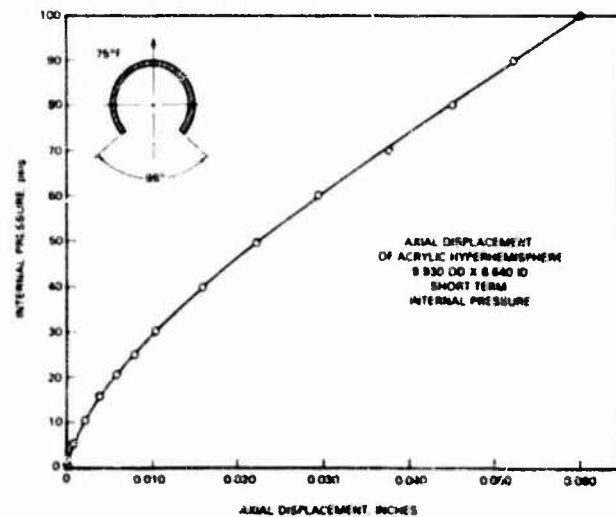
Fig. 11 Axial displacement of acrylic window under internal pressure
