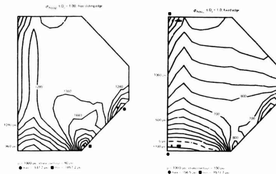
Fig. 27 Plot of \sigma_{hoop} stress contours in a t/D_1 = 1.0 plane disk with twin conical bearing surfaces
