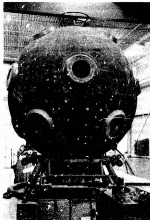
Fig. 7 Typical diving bell with twin bevel plane disk windows fabricated by Southwest Research Institute for the Suh Sea International. Note the small bulk of mountings for 8-in. dia. viewports
