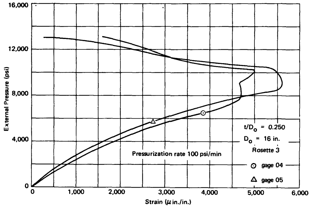
Figure A-27. Strains on the interior of sphere No. 33 under external pressure; rosette 3.
