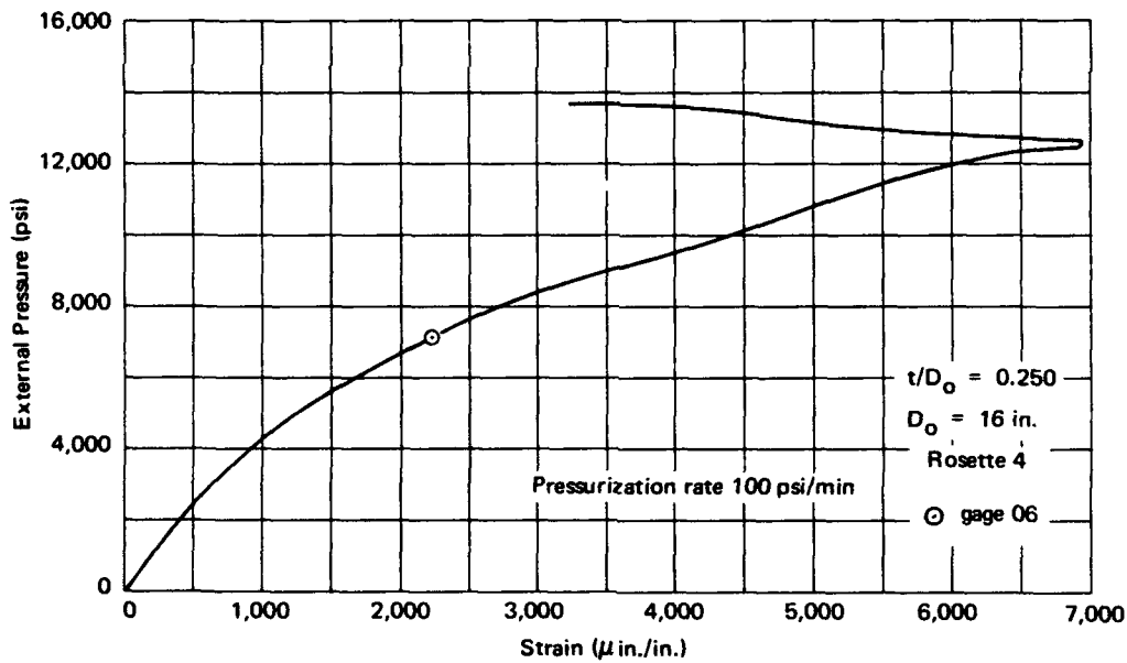
Figure A-28. Strains on the exterior of sphere No. 33 under external pressure; rosette 4.
