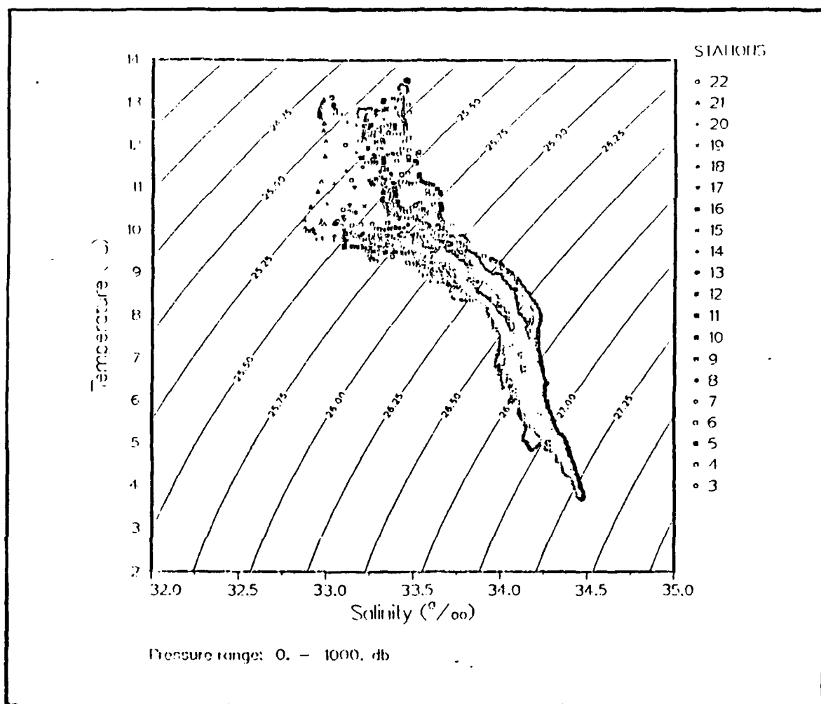
Figure 5. Temperature and salinity characteristics. Station locations are shown in Figure 1.
