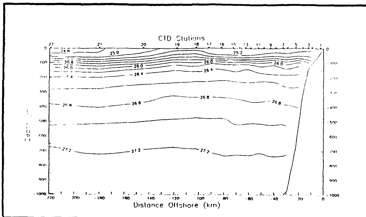
Figure 4. Density anomaly transection. Isopycnal spacing is every 0.2 \text{ kg/m}^3 . Station locations are shown in Figure 1. Distance offshore is measured from Pt. Sur, Ca.
