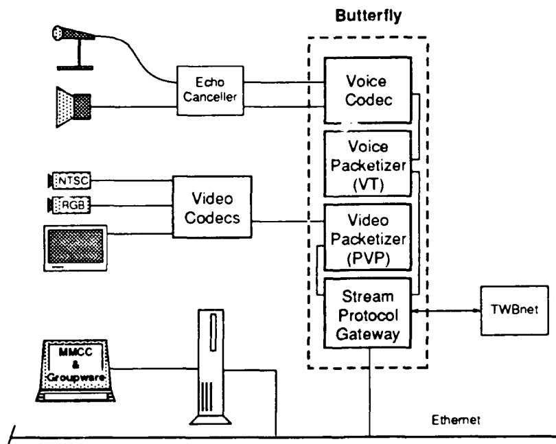
Figure 2. System Components
