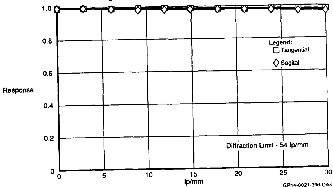
Figure 5.1-41. Modulation Transfer Function Material - ZnS/ZnSe Wavelength - 7.5 - 12 Microns Sample Size - 12 x 12 In. 5-33
