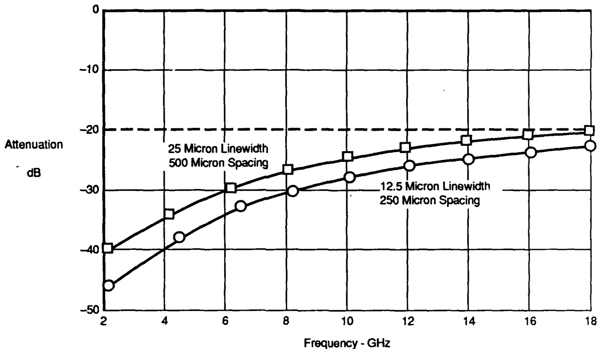
Figure 5.2-15. Microwave Attenuation in dB Through Inductive Grids
