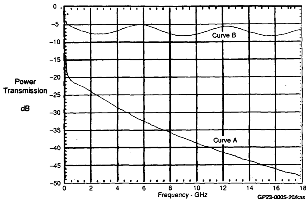
Figure 5.2-8. RF Transmission Sample Type: GaAs (Gold Coated/Silver Edge Painted) Sample Size: 7mm Coaxial Test Type: Airline Coaxial
