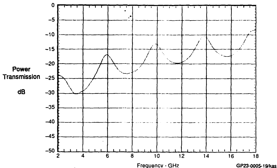
Figure 5.2-7. RF Transmission Sample Type: ZnS/ZnSe Sample Size: 12 x 12 Inch Test Type: Tunnel
