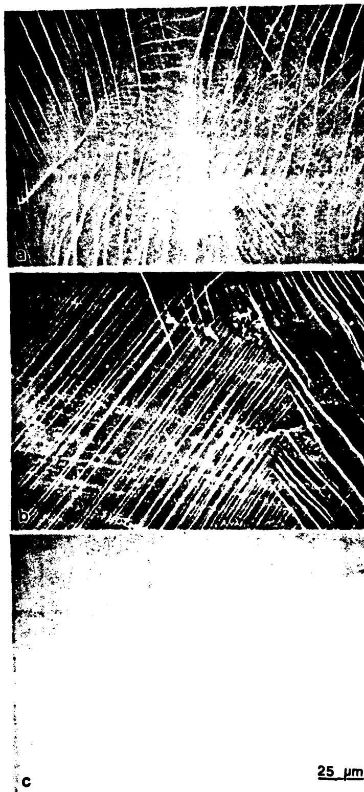
Figure 3. Optical micrographs showing slip lines on the surface of compression specimens after 0.03 strain and which have been solution-treated and aged for 6 hrs at (a) 375°C, (b) 575°C, (c) 675°C.
