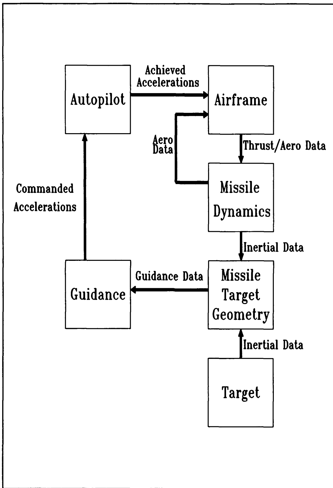
Figure 3.1 Missile Flight Simulation
