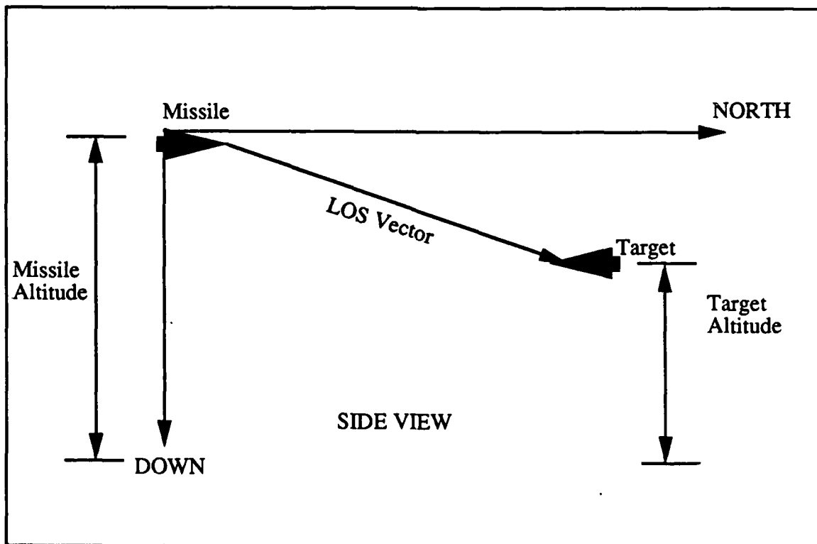
Figure 4.2 North-Down Planar View
