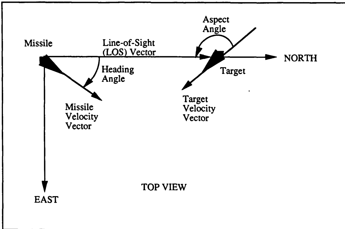
Figure 4.1 North-East Planar View
