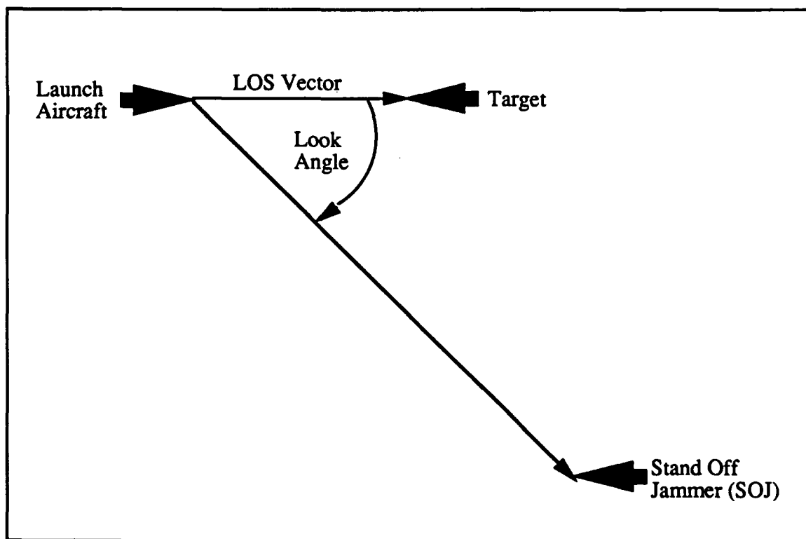
Figure 4.8 SOJ Look Angle
