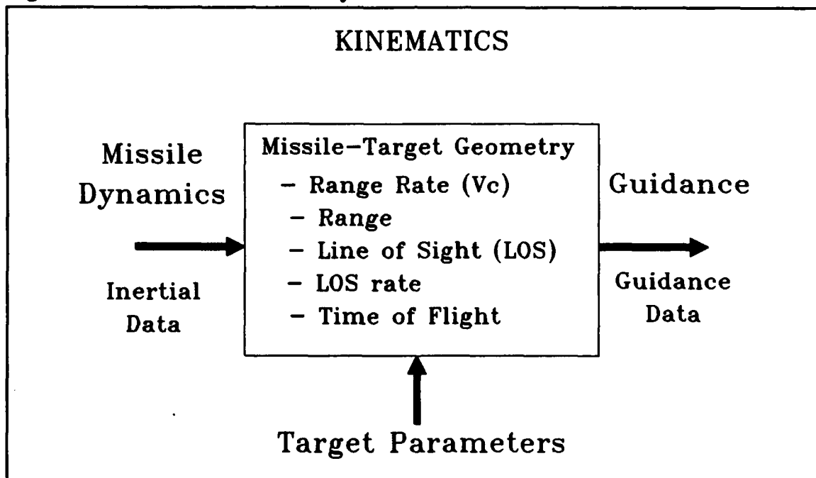
Figure 3.5 Kinematics: Missile-Target Geometry
