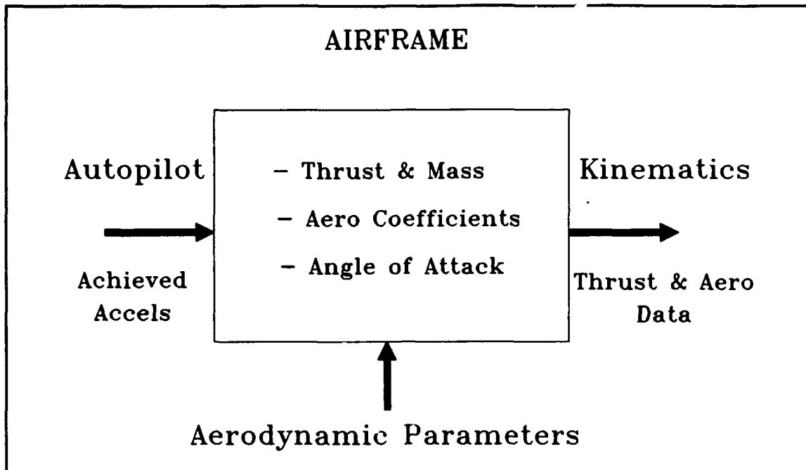
Figure 3.3 Airframe Model
