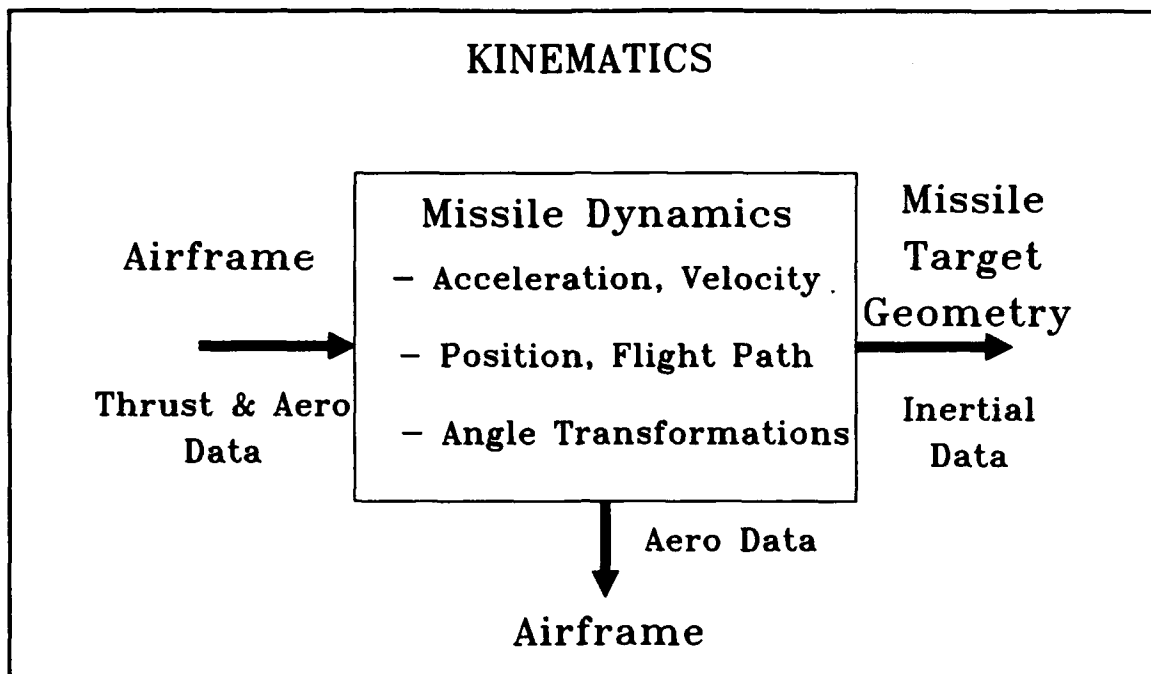
Figure 3.4 Kinematics: Missile Dynamics
