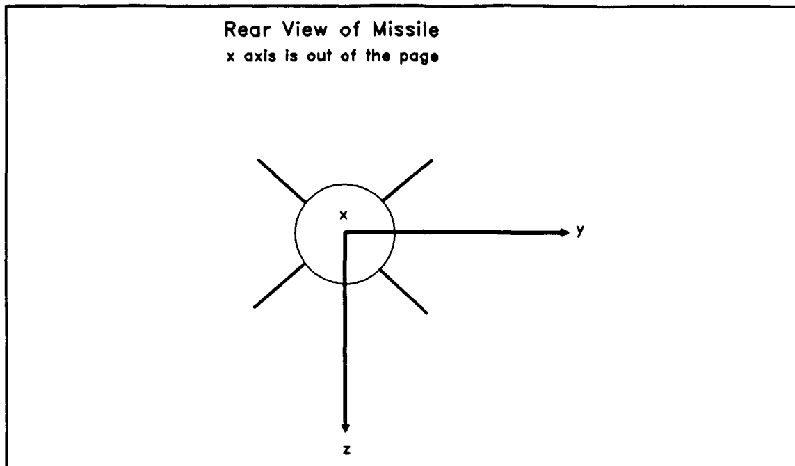
Figure 3.2 Missile Reference Axes
