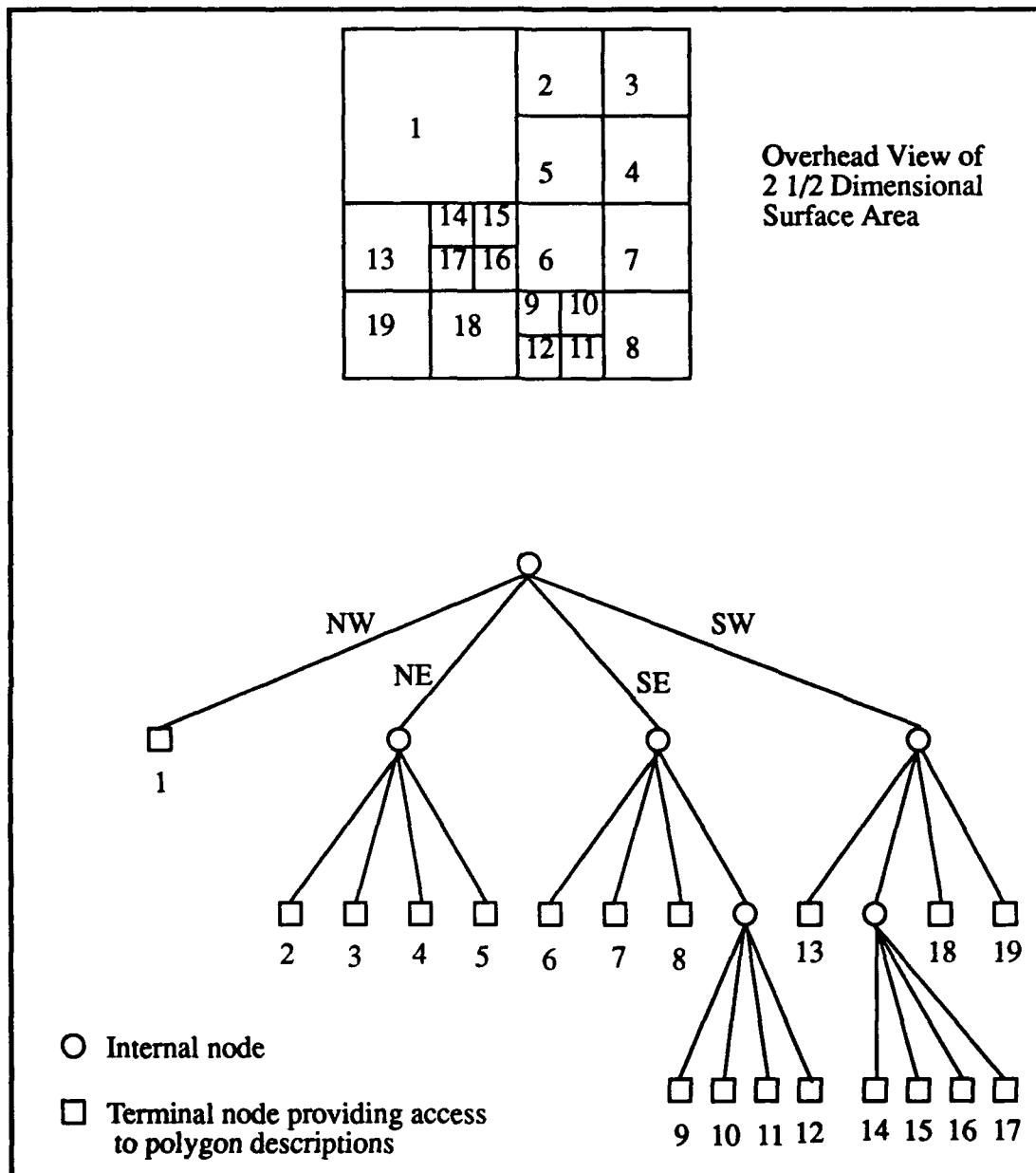
Figure 5.3 Quadtree Providing Spatial Index into 2 1/2 Dimensional Area
