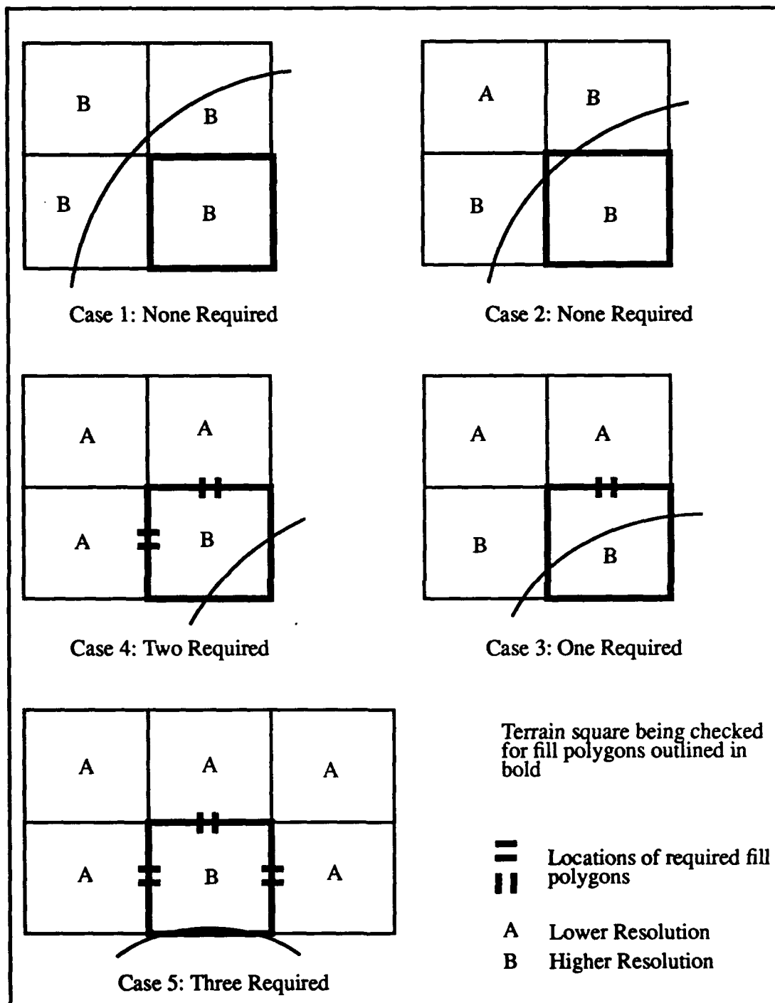
Figure 7.7. Circle-Rectangle Intersection and Required Fill Polygons
