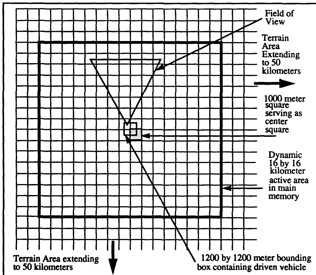
Figure 4.1. Active Area of Terrain in NPSNET
