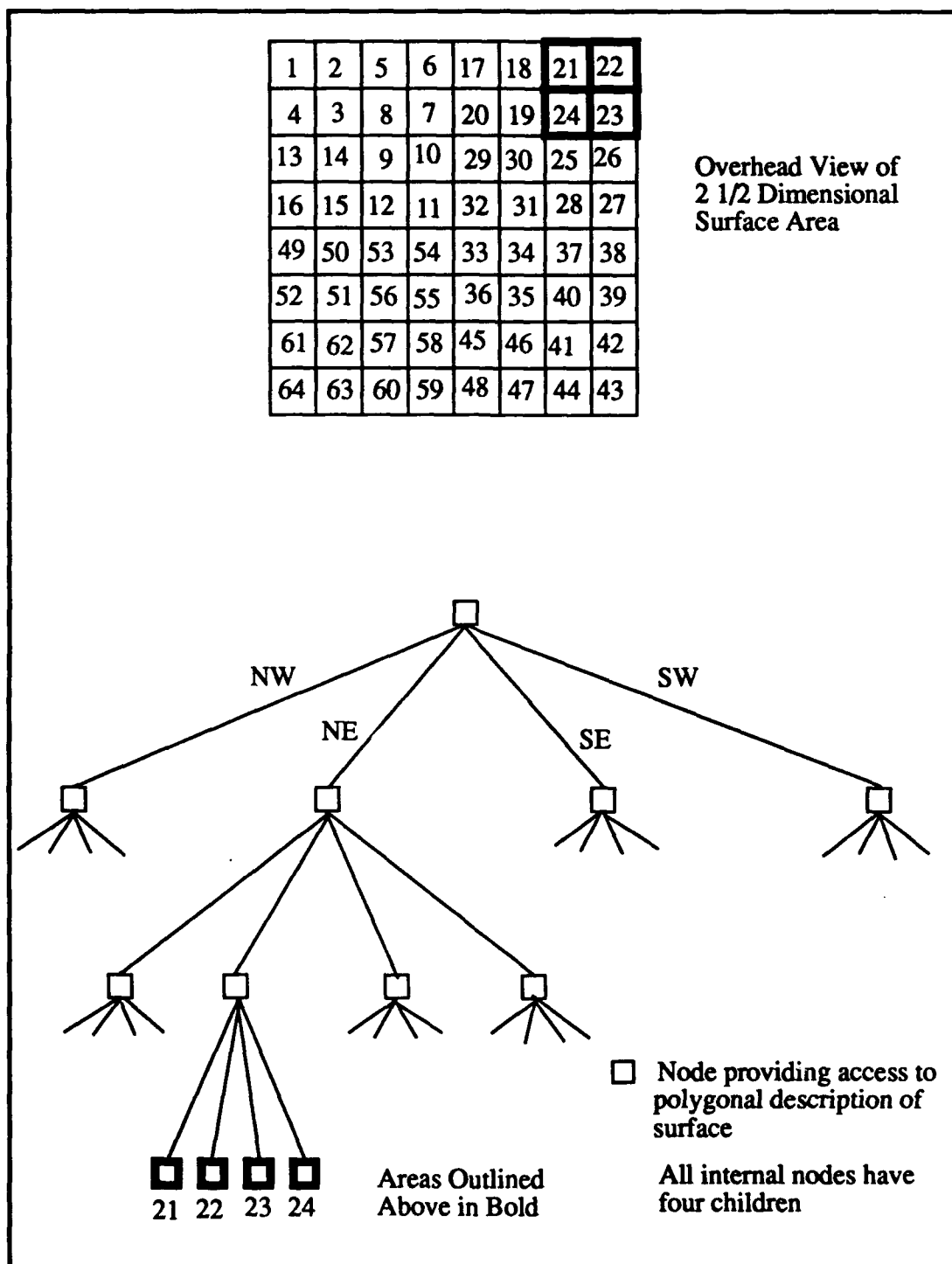
Figure 5.5. Full Quadtree Providing Spatial Index to Multiple Resolution Description of a 2 1/2 Dimensional Surface
