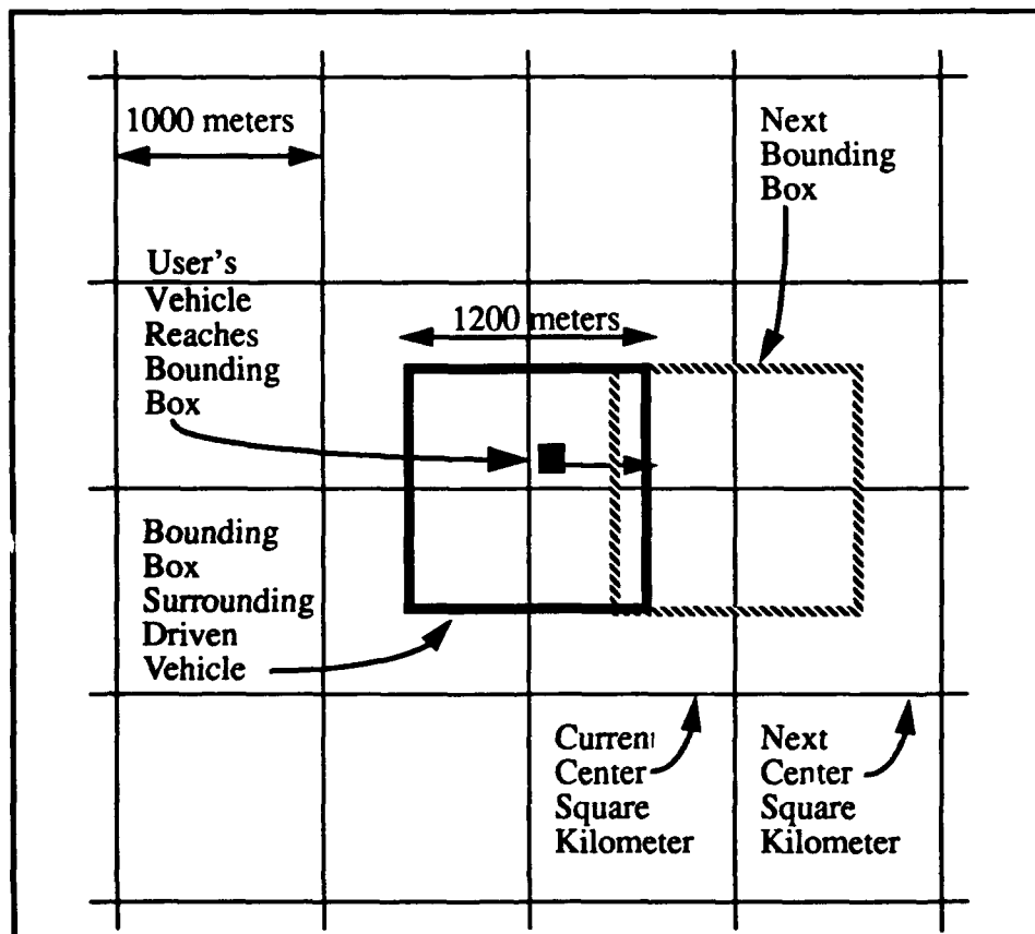
Figure 4.2. Boundaries for Terrain Paging in NPSNET
