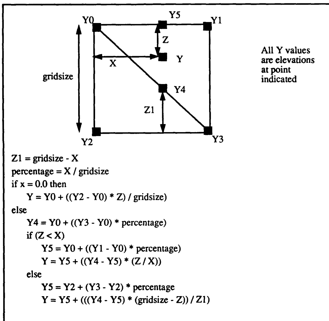
Figure 7.9. Algorithm for Determining Elevation Within Square of Terrain
