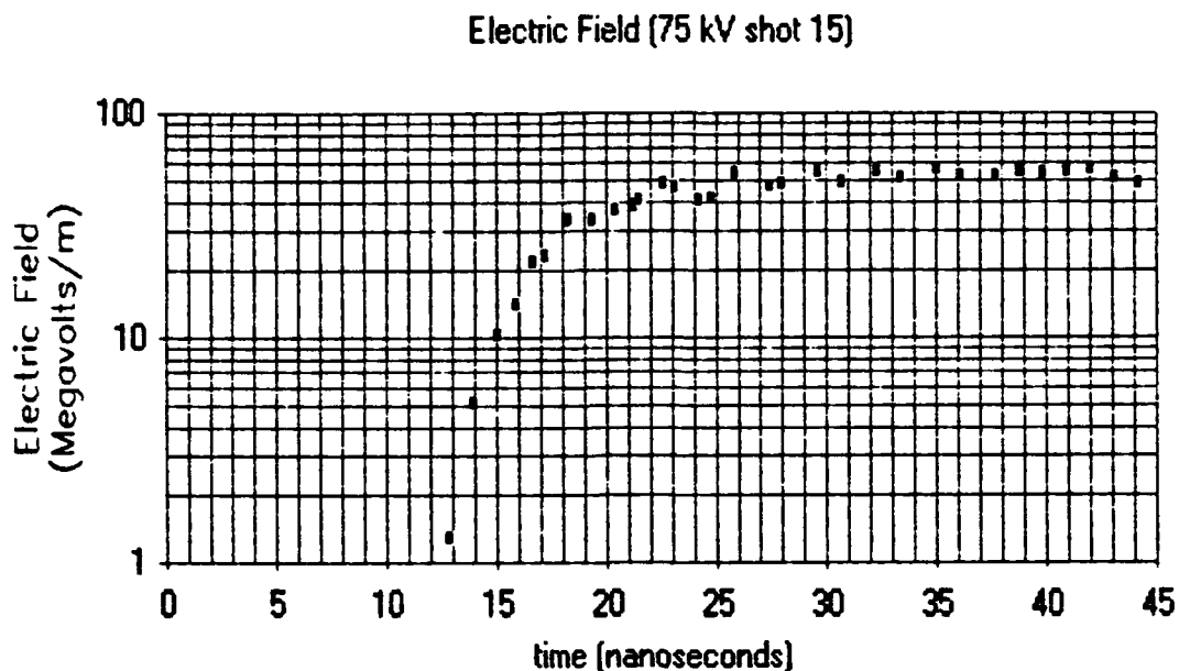
Figure 5.38 Electric Field vs. time for a 75 kV shot. The field crosses the 10 MV/m value at approximately 15 ns.
