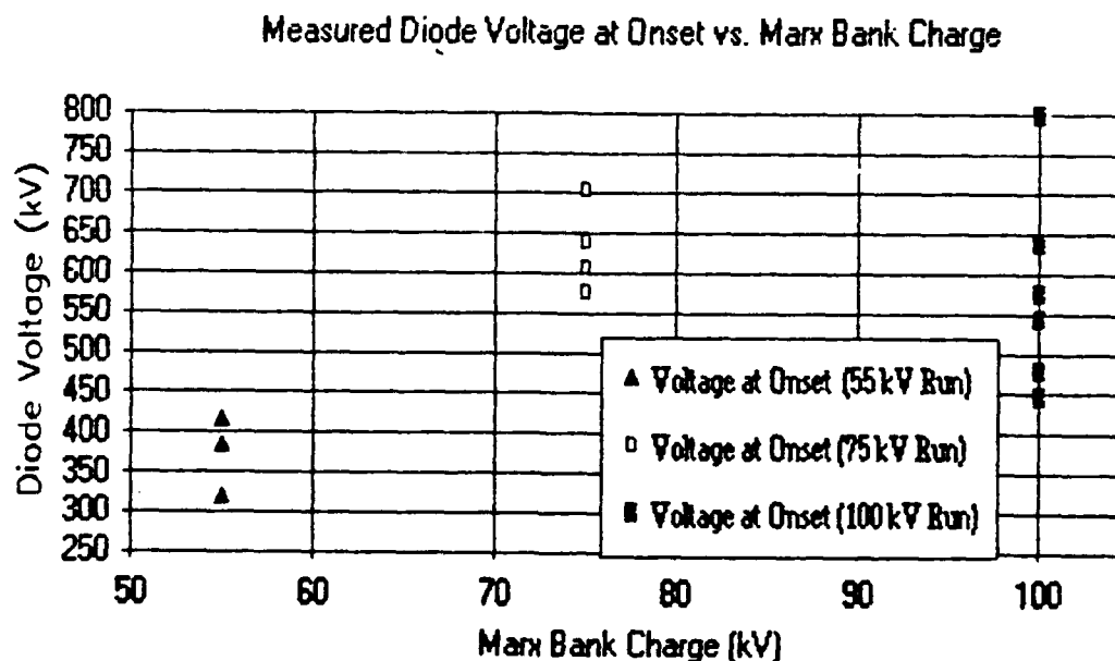
Figure F.2 Diode Voltage at Plasma Onset vs. Marx Bank Charge for the 55 kV, 75 kV, and 100 kV Data Runs.
