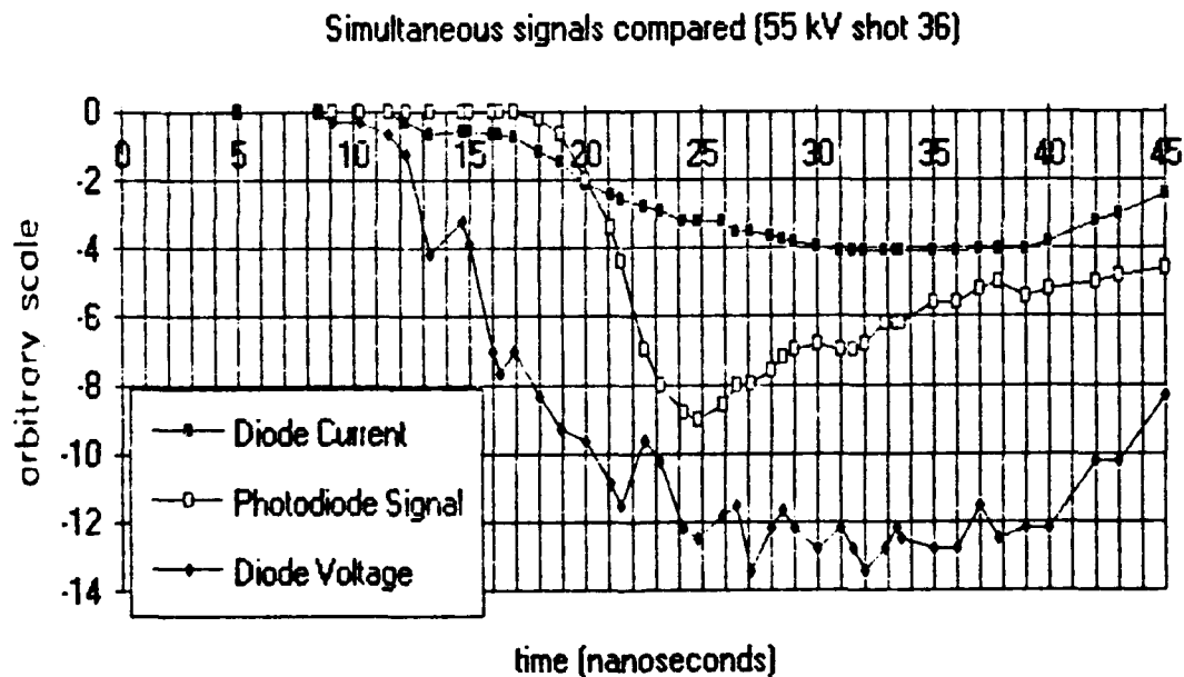
Figure 5.25 Diode Voltage, Diode Current, and Photodiode waveforms for a 55 kV shot plotted on an arbitrary vertical scale.
