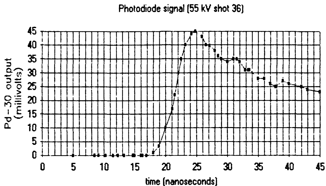
Figure 5.24 Photodiode waveform for a 55 kV shot. Same arbitrary zero time as Figure 5.22.
