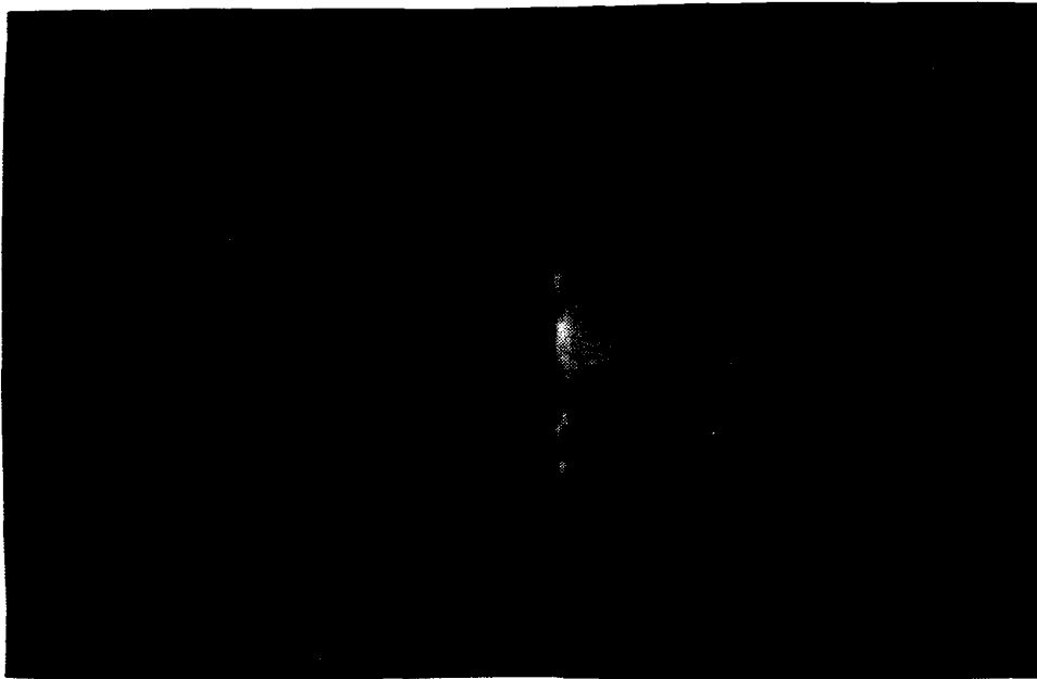
Figure 5.8 Time lapsed photograph of a 100 kV shot using a 2.5% neutral density filter. Notice multiple cathode spots.
