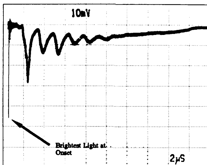
Figure 5.1 Scanned, computer enhanced, photograph of the long time ( 2 \mu\text{s}/\text{div} ) photodiode waveform for a 75 kV shot. The brightest light occurs at onset. Later peaks correlate to ringing of the diode voltage and current waveforms.
