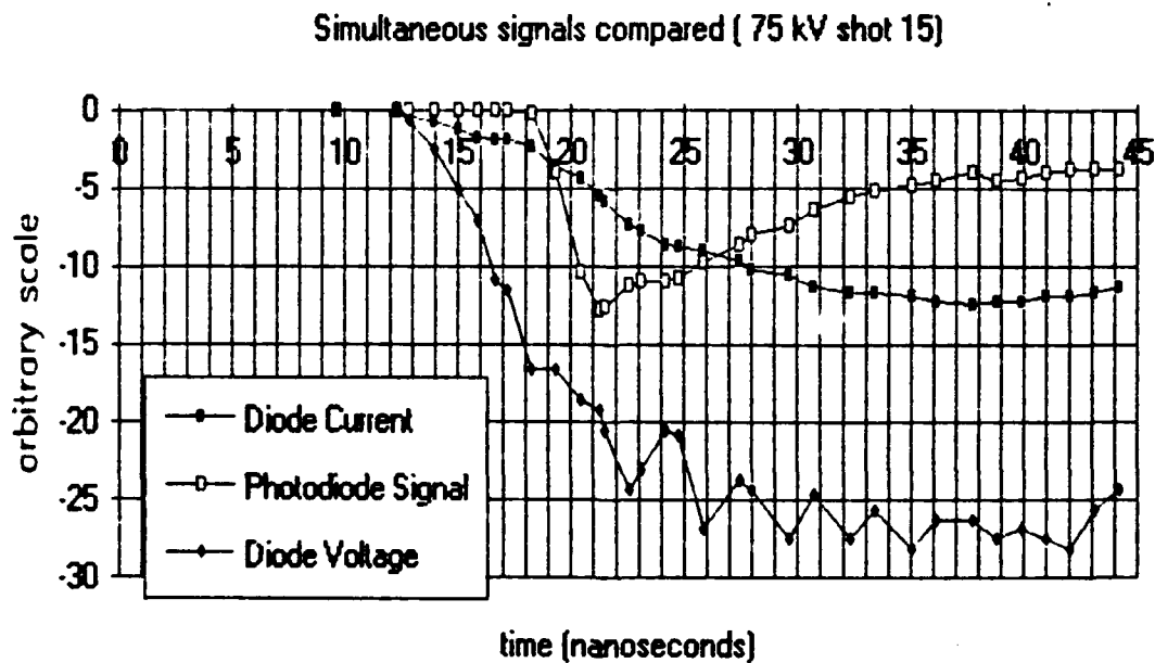
Figure 5.29 Diode Voltage, Diode Current, and Photodiode waveforms for a 75 kV shot plotted on an arbitrary vertical scale.
