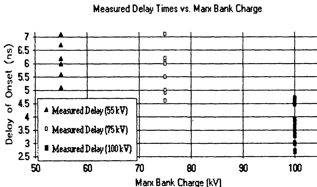
Figure F.1 Delay Time of Plasma Onset vs. Marx Bank Charge for the 55 kV, 75 kV and 100 kV Data Runs.
