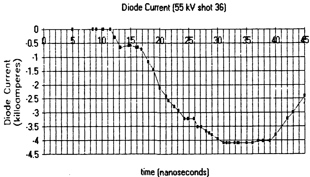
Figure 5.23 Diode Current waveform for a 55 kV shot. Same arbitrary zero time as Figure 5.22.
