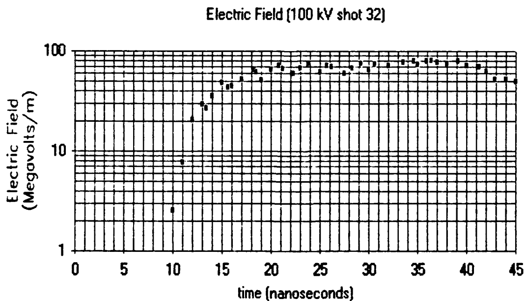
Figure 5.39 Electric Field vs. time for a 100 kV shot. The field crosses the 10 MV/m value at approximately 11 ns.
