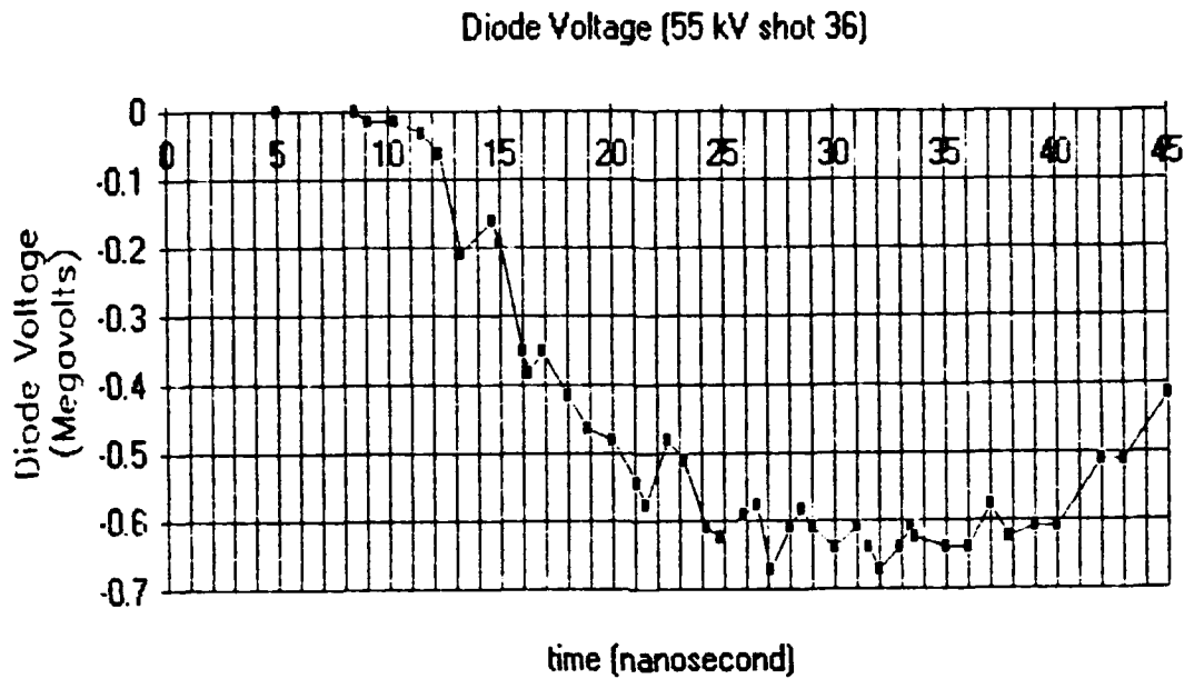
Figure 5.22 Diode Voltage waveform for a 55 kV shot. The zero of time is arbitrarily chosen.
