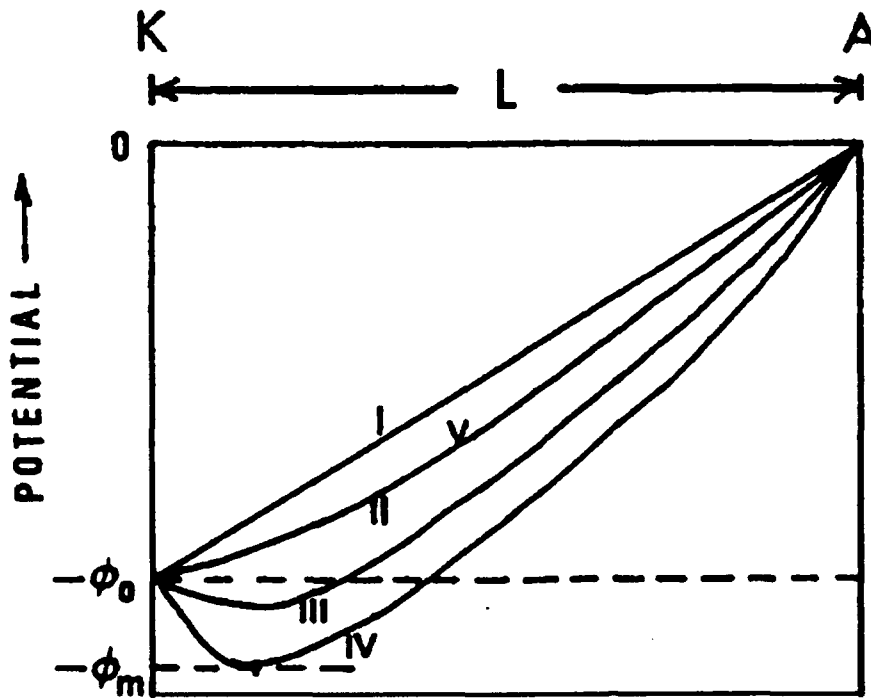
Figure 2.2 Electrostatic potential in diode including electron space charge. A time dependent potential minimum forms near cathode(K) surface. I through V are sequential in time. Anode(A) is distance L from K. [Ref. 4]
