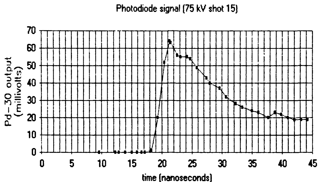
Figure 5.28 Photodiode waveform for a 75 kV shot. Same arbitrary zero time as Figure 5.26.
