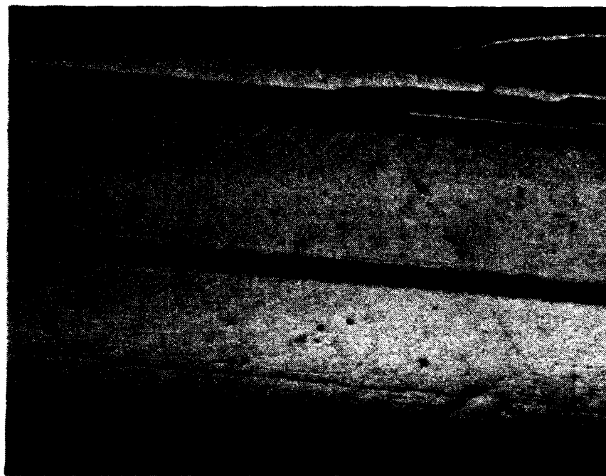
Fig. 3 W/Zr laminate with cracking delamination, 50X
