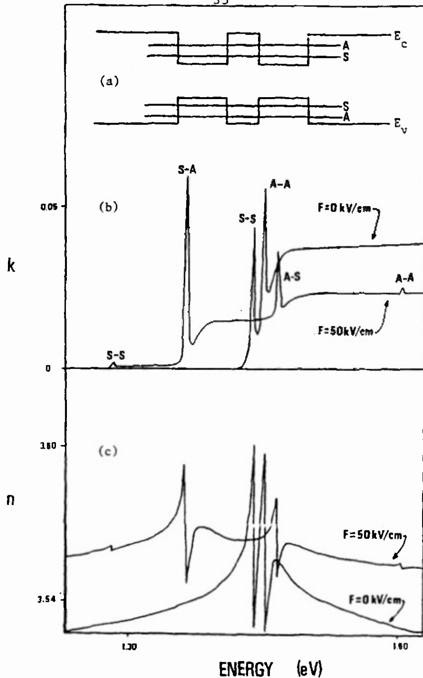
Fig.12 (a) Shows schematic band diagram of CDQW under flat band conditions with the symmetric (S) and antisymmetric (A) confined electron and hole energy levels. (b) Shows absorption coefficient k as a function of transition energy for 0 and 50 kV/cm total field based on phenomenological model. (c) Shows index of refraction n as a function of transition energy for 0 and 50 kV/cm total field based on a phenomenological model.
