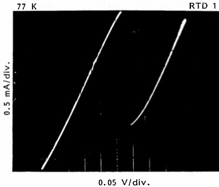
Figure 6b I-V curve of RTD 1 having 30% Al barriers measured at 77 K. The device dimension is 12 x 12 \mu m . This device shows a Peak to Valley Ratio of 3.3 with a peak current density of 3.5 kA/cm^2 . Note that origin of I-V curve is shifted to bottom of third quadrant.
