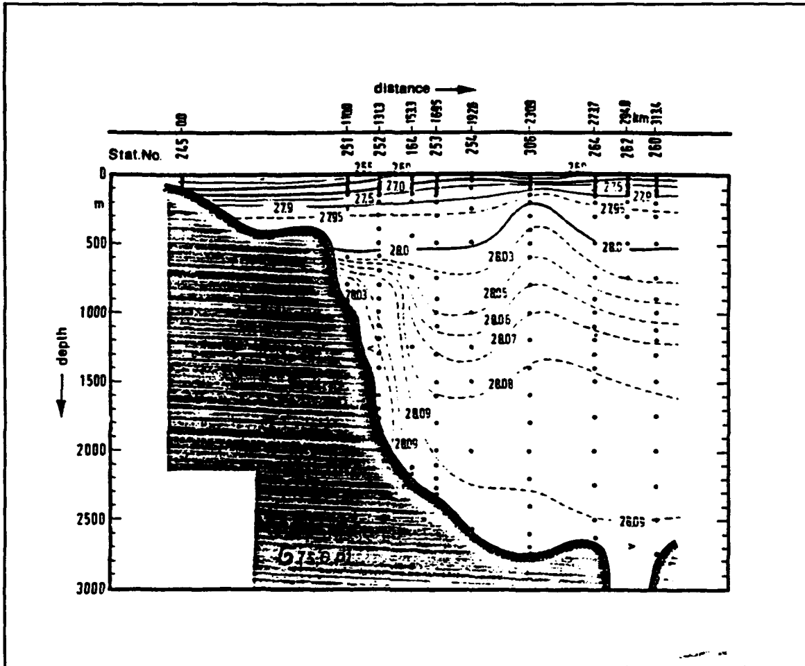
Figure 20. Cross section at 79°N showing the density structure associated with the southward flowing bottom boundary current against the continental slope (from Koltermann and Lüthje, 1989).
