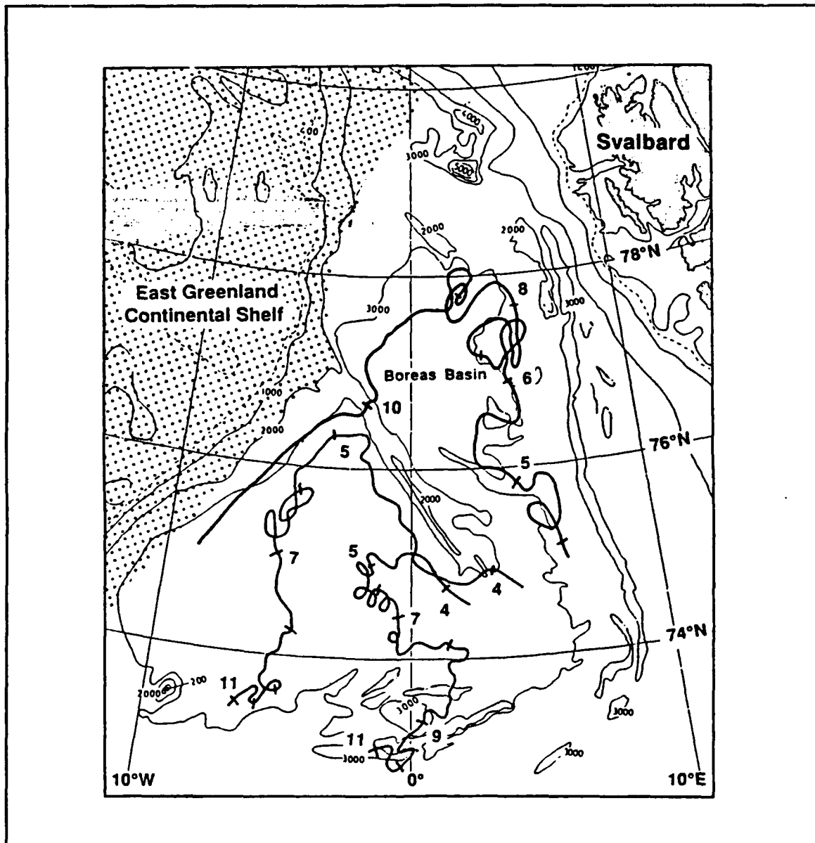
Figure 16. Trajectory of satellite tracked buoys (drogue at 30 m) from MIZEX '87 (numbers indicate date of position) (from GSP Group , 1989).
