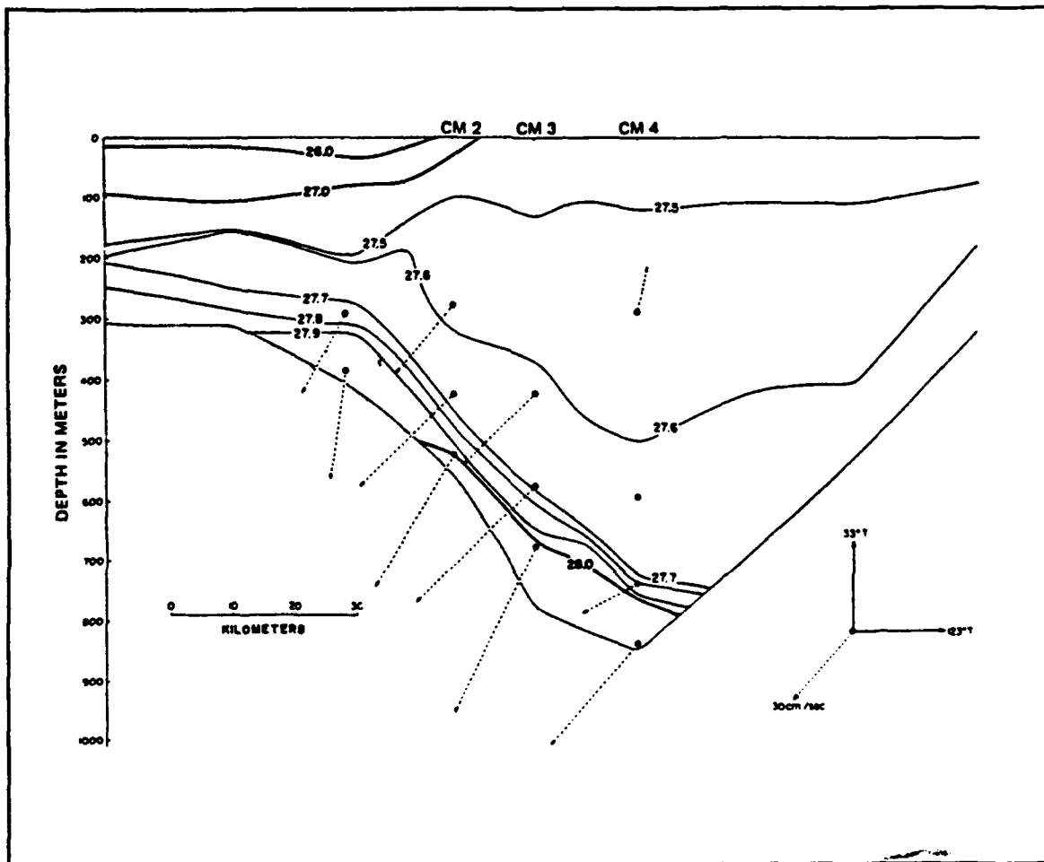
Figure 19. Vertical density ( \sigma_t ) cross section across the Denmark Strait (from Smith, 1976 ). Dotted arrows show that measured currents near bottom are directed to the southwest and that they are accelerated as the current is forced against the continental slope.
