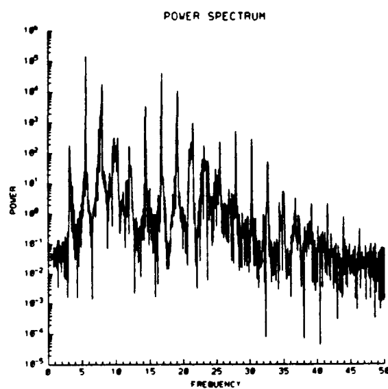
Figure 3.7 Fourier spectrum Duffing's equation.
