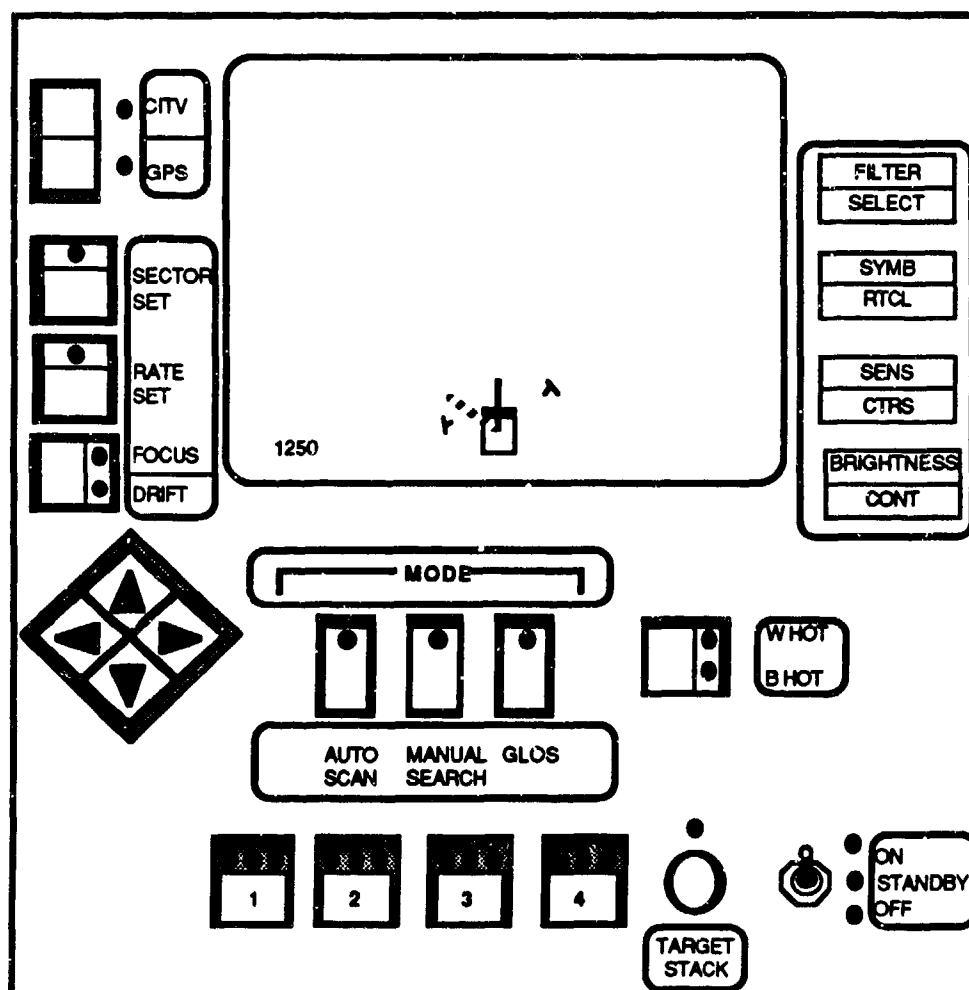
Figure 5. Commander's Independent Thermal Viewer (CITV)
