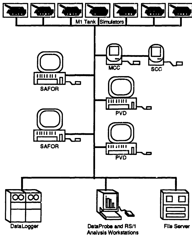
Figure 2. Simulation Networking (SIMNET) Architecture
