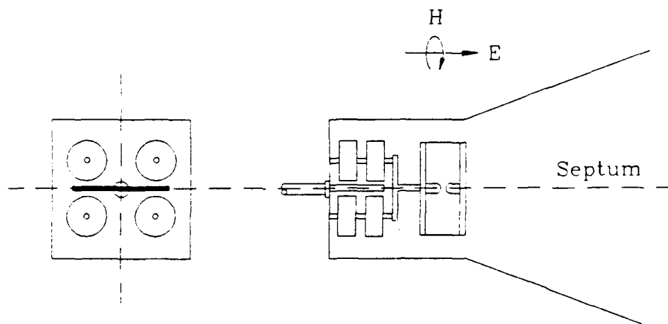
Figure 38b: Horizontal orientation of the capacitor unit.
