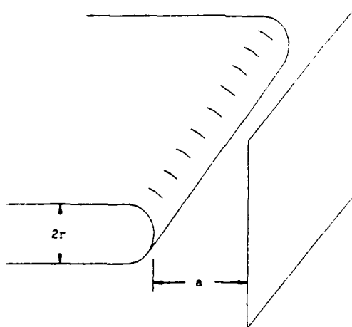
FIGURE 29 Field enhancement between a plate with rounded edges and a flat plate
