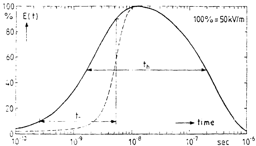
FIGURE 14 Model for exo-atmosphere EMP
