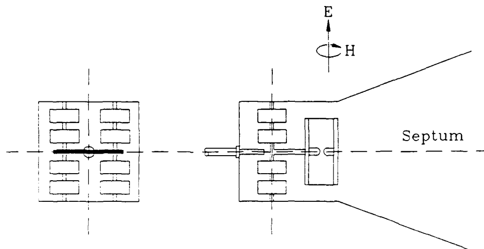
Figure 38a: Vertical orientation of the capacitor unit
