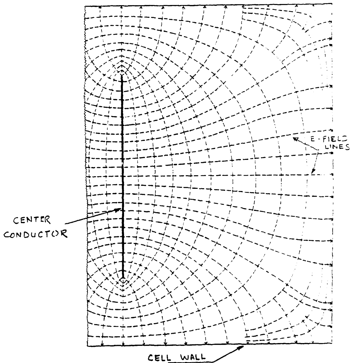
FIGURE 18 General field distribution in a TEM cell
