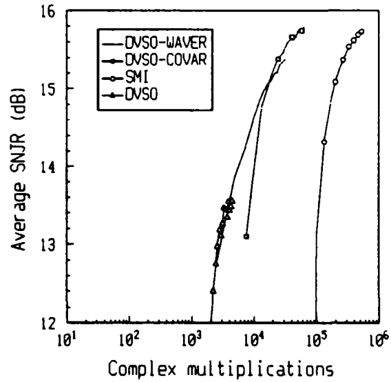
Fig. 48 Average SNJR versus complex multiplications for DVSO-WAVER, DVSO-COVAR, SMI and DVSO methods for K=40 and L=3 . Monte-Carlo simulations with 100 trials.
