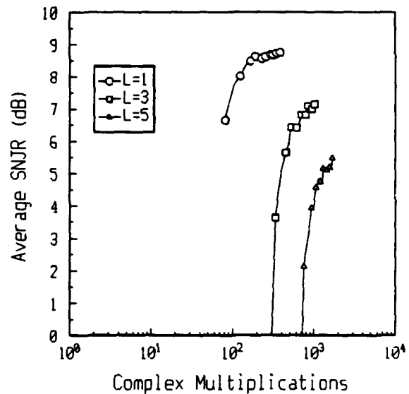
Fig. 12 Average SNJR versus complex multiplications for DVSO method for L=1, 3 and 5 . Monte-Carlo simulations with 100 trials.
