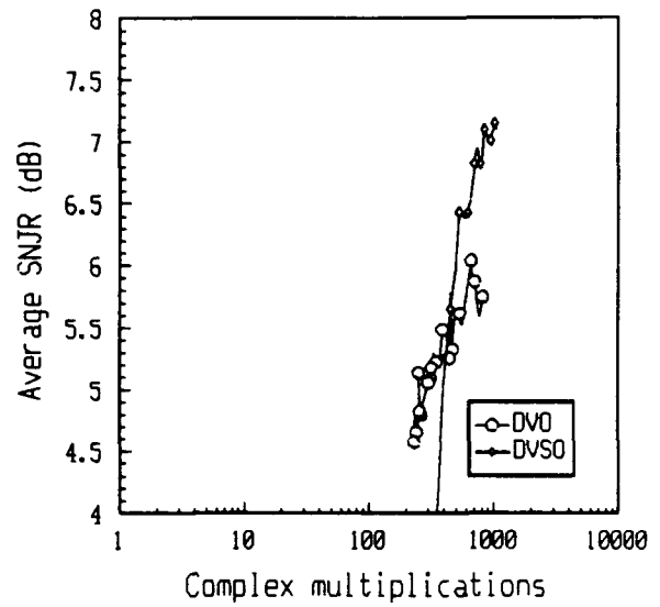
Fig 19 Average SNJR versus complex multiplications for the DVO and DVS0 methods with K=10 and L=3 . Monte-Carlo simulations with 100 trials.
