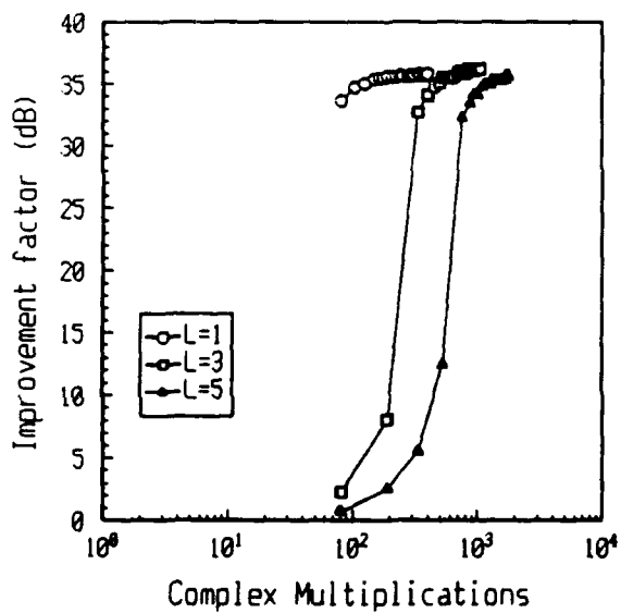
Fig. 13 Improvement factor versus complex multiplications for DVSO method for L=1, 3 and 5 . Monte-Carlo simulations with 100 trials.
