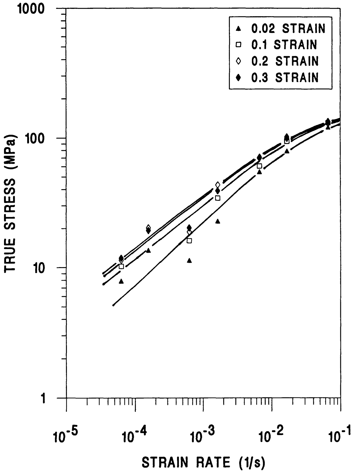
Figure 20. True Stress vs Strain Rate Curves for the Al-10Mg-0.5Mn Alloy at 300°C for True Strains Between 0.02 and 0.3.
