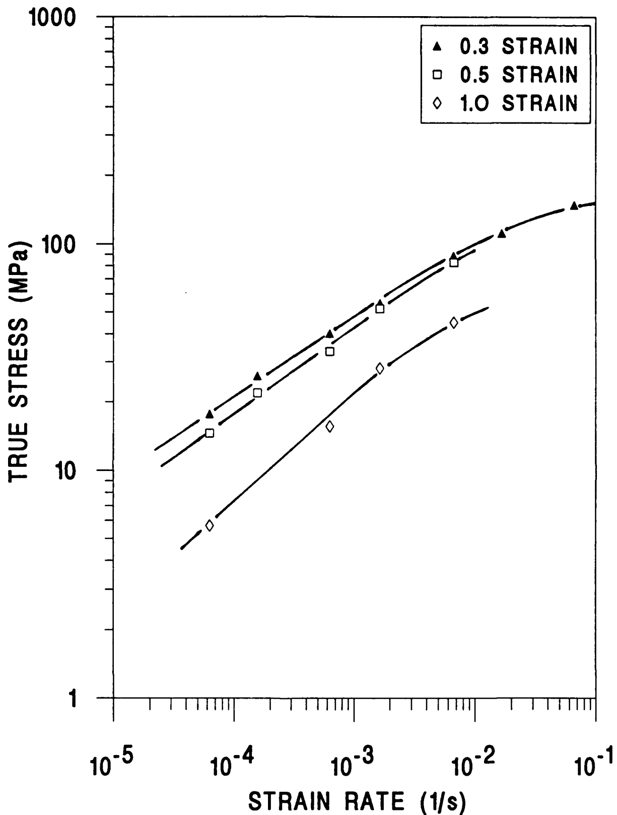
Figure 21. True Stress vs Strain Rate Curves for the Al-10Mg Alloy at 300°C for True Strains Greater than 0.3.
