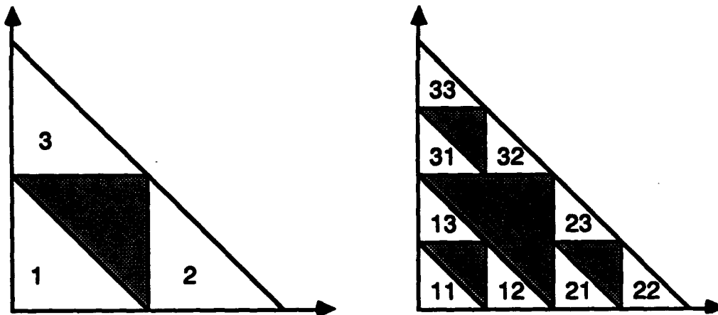
Figure 3.22 An addressing scheme for the Sierpinski triangle.
