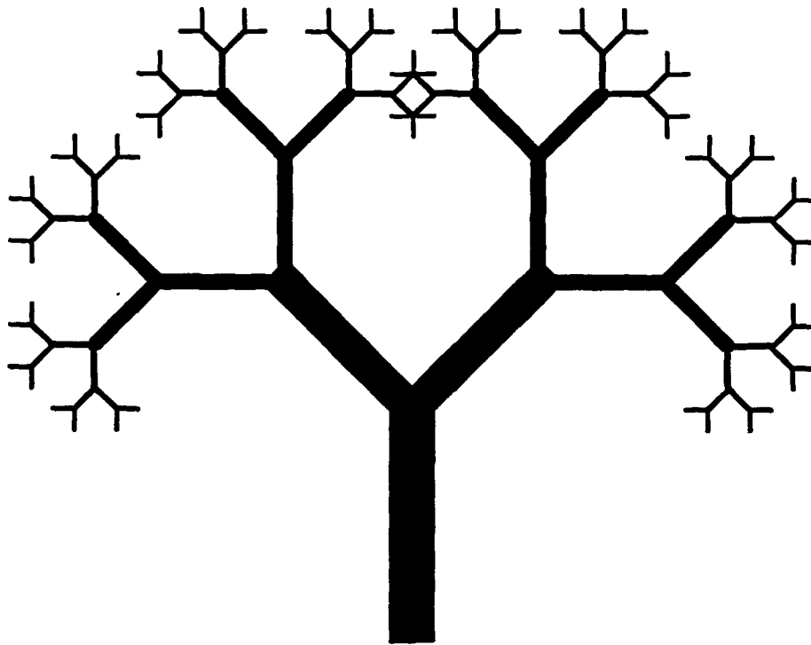
Figure 3.14 A fractal tree.
