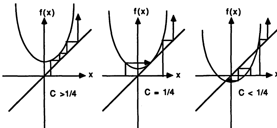
Figure 4.29 Graphs of f(x) = x^2 + c for c > 1/4 , c = 1/4 , and c < 1/4 .
