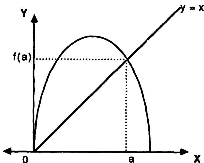
Figure 2.3 A fixed point a of f(x) : f(a) = a .
