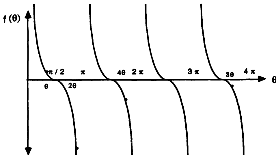
Figure 4.11 The cotangent map and a chaotic orbit.
