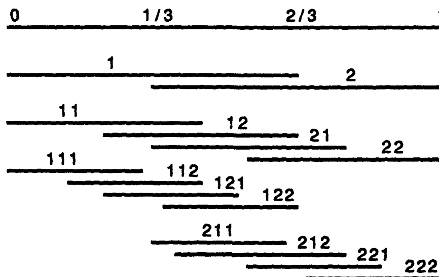
Figure 3.21 Addressing the attractor of an overlapping IFS.
