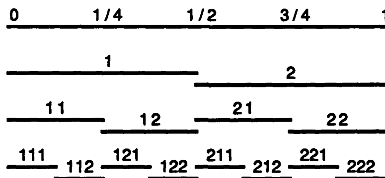
Figure 3.20 Addressing the attractor of a just-touching IFS.
