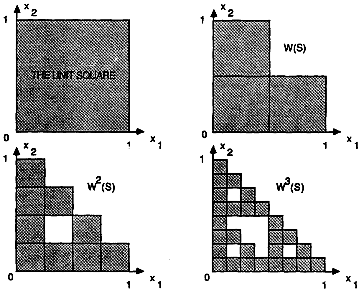
Figure 3.11 Creating the Sierpinski triangle by iterating the unit square.
