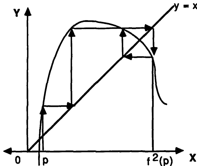
Figure 2.6 An eventually periodic point p of f(x) : f^2(p) is periodic.
