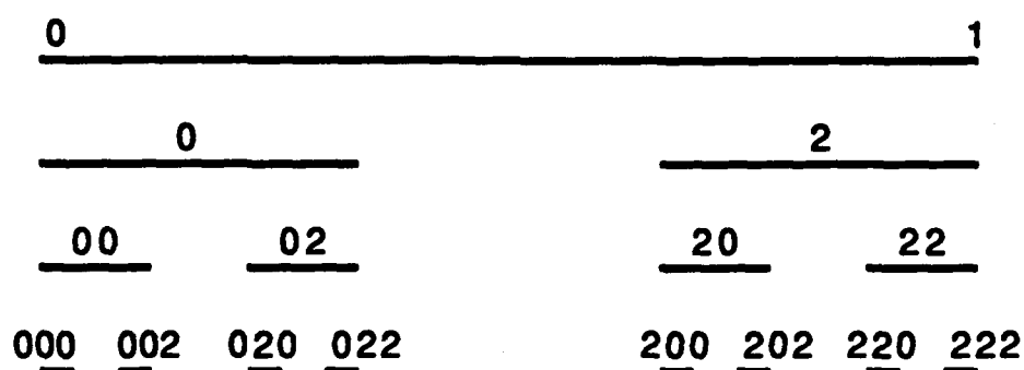
Figure 3.19 Addressing the attractor of an iterated function system.
