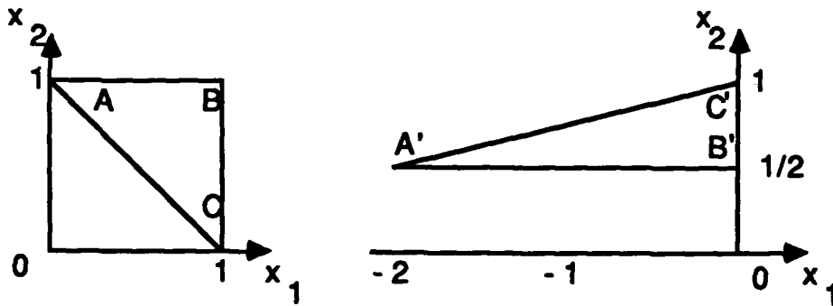
Figure 3.3 An affine transformation of a triangle.
