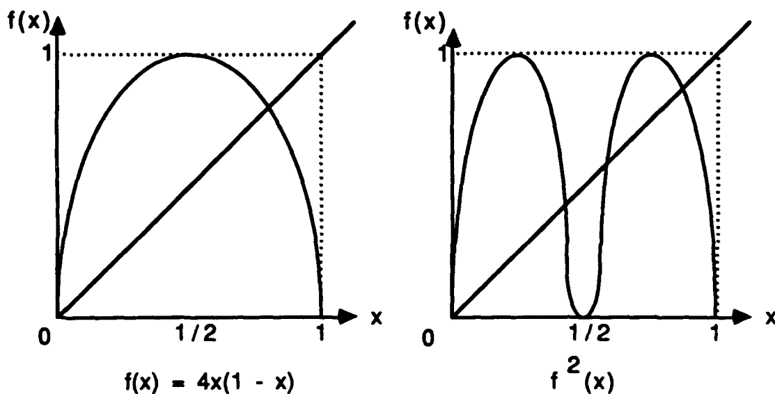
Figure 4.3 The first and second iterates of f(x) = 4x(1-x) .
