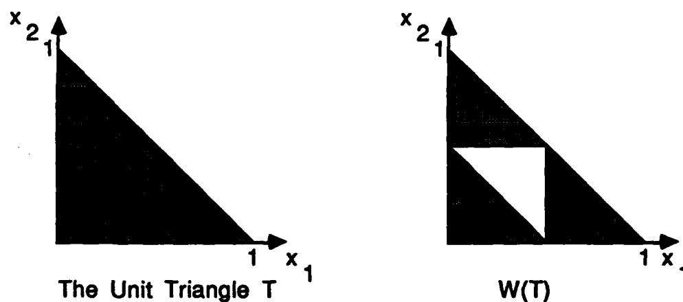
Figure 3.8 The effect of W on the unit triangle.
