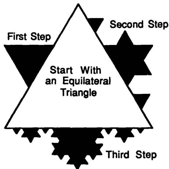
Figure 3.28 Constructing the Koch snowflake.
