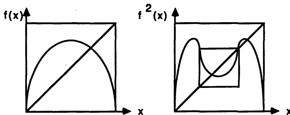
Figure 4.20 The first and second iterates of the logistic equation.
