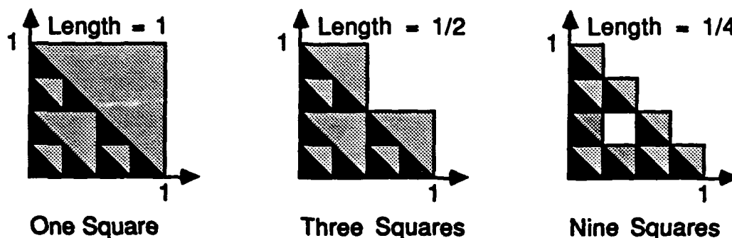
Figure 3.27 Covering the Sierpinski triangle with grids of size 1/2^n .
