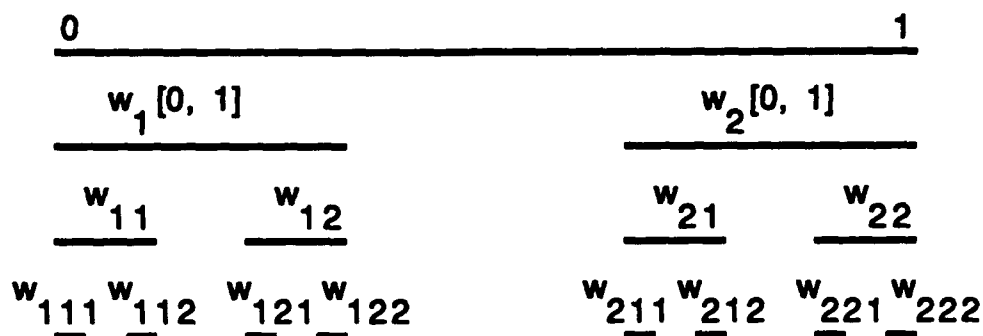
Figure 3.7 Creating the Cantor set through an iterated function system (IFS).
