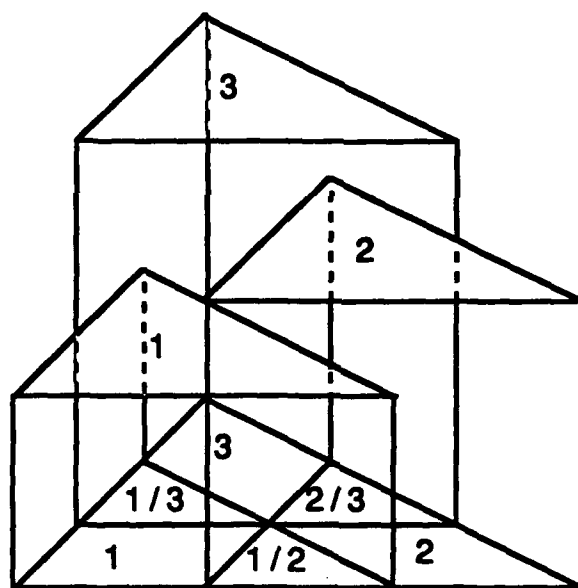
Figure 3.24 Lifting an attractor into the third dimension.
