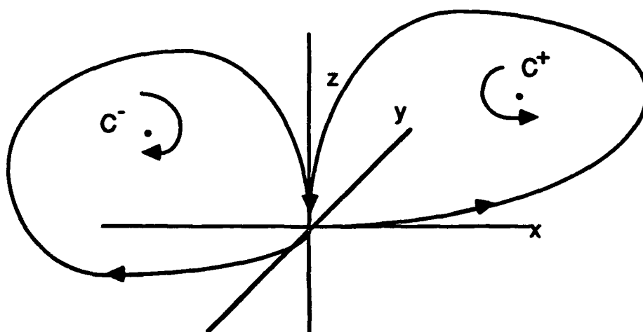
Figure 4.55 The homoclinic orbit of the Lorenz equations.
