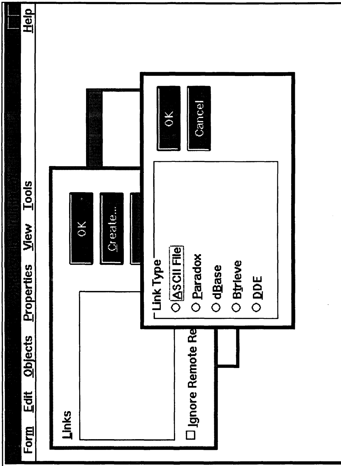
Figure 10a ObjectVision
