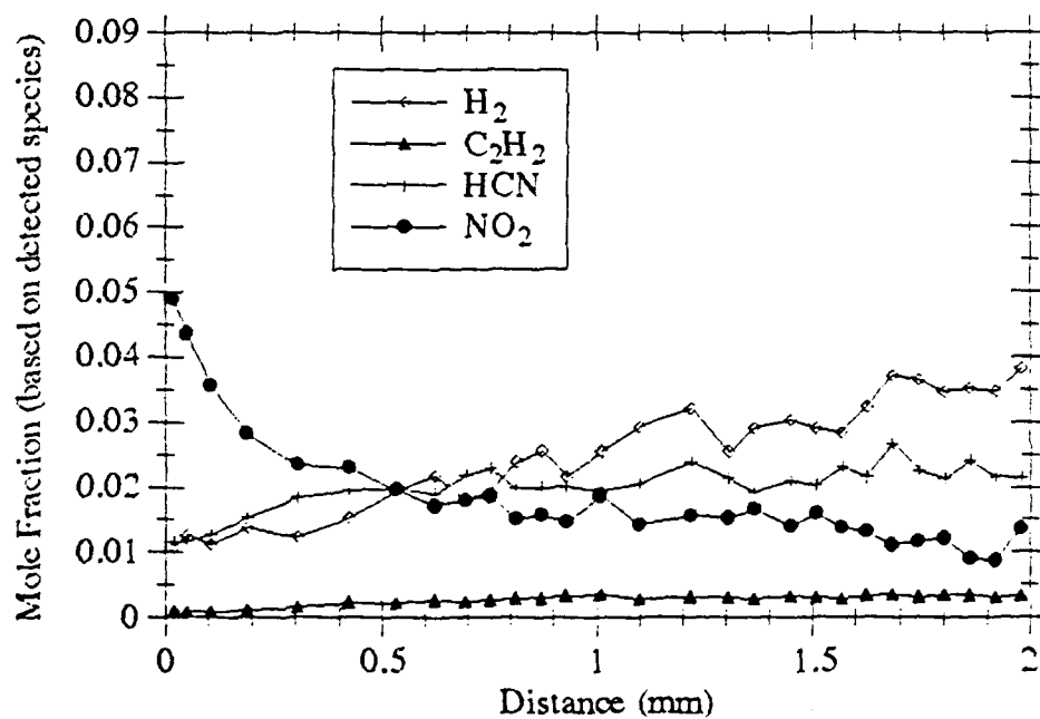
Figure 2. Species profiles for a double-base propellant, JA-2, in argon at one atmosphere with a heat flux of 100 W/cm 2 .
