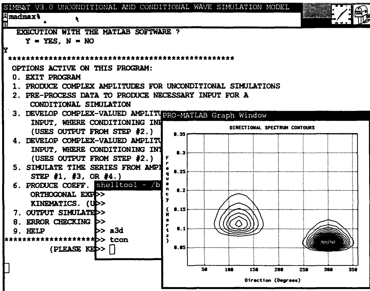
Figure A-11. Example of computer console executing SIMBAT interactively with MATLAB graphics in another window.
