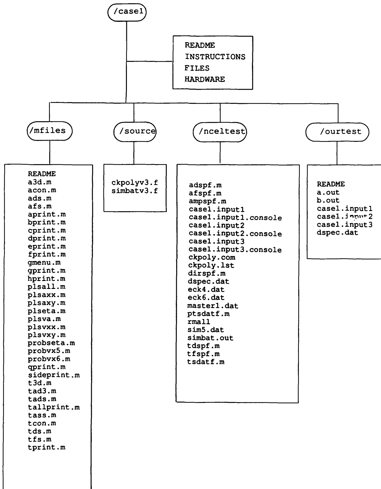
Figure A-1. Example No. 1 directory and file structure.
