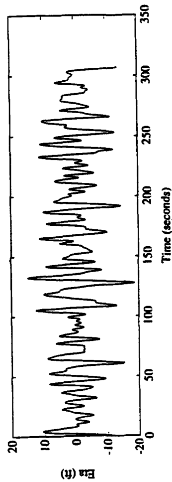
Simulated Wave Profile with Large Wave Embedded
