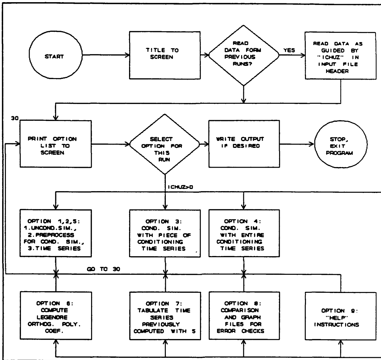
Figure 4. Flow of control in SIMBAT.
