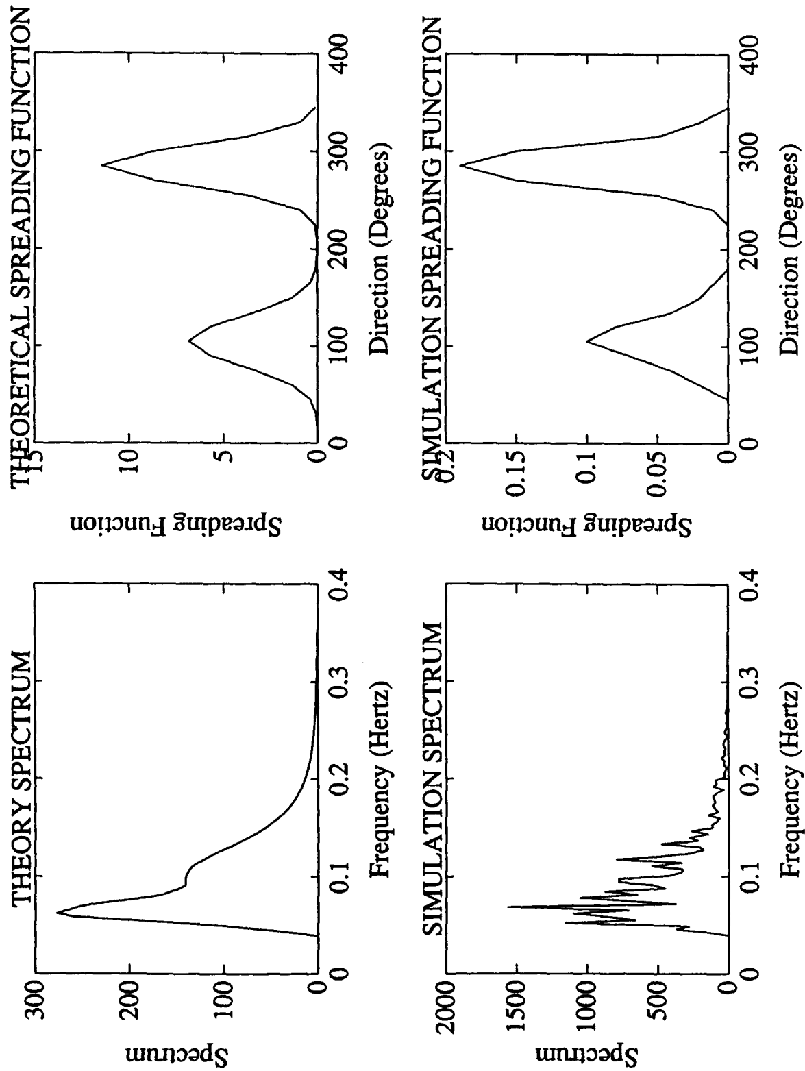
Figure B-19. Comparison of theoretical and simulated 2D spectra and spreading function.
