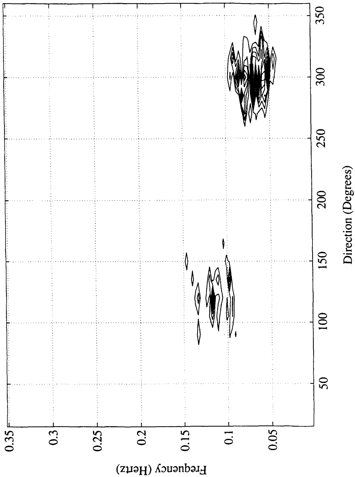
Figure A-17. Simulated contour plot of spectra.
