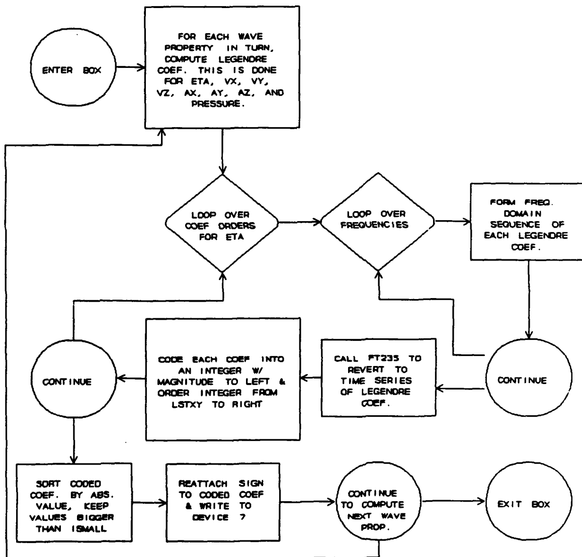
Figure 15. Details for Box A in Subroutine POLYEX.
