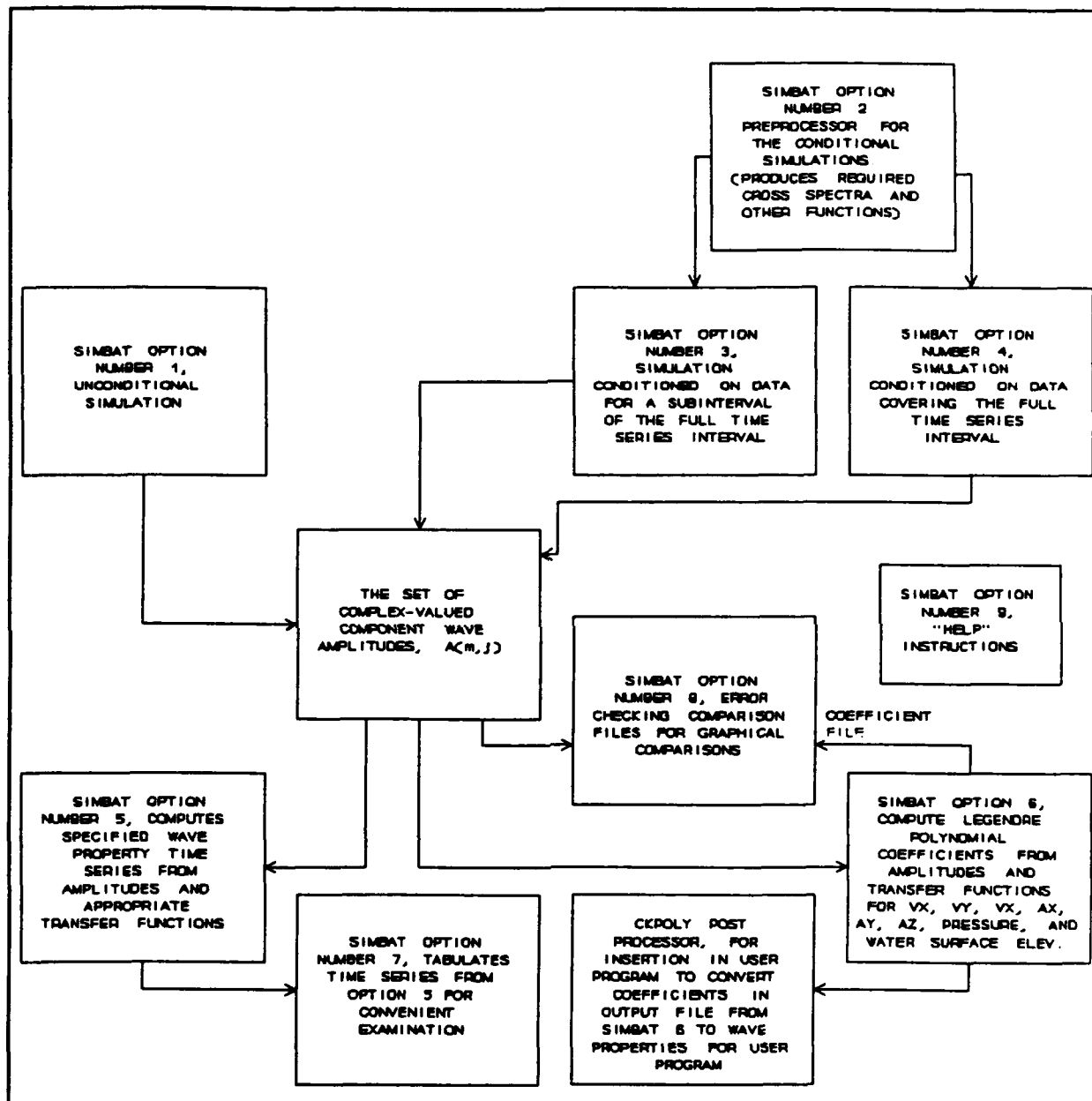
Figure 3. General program structure.
