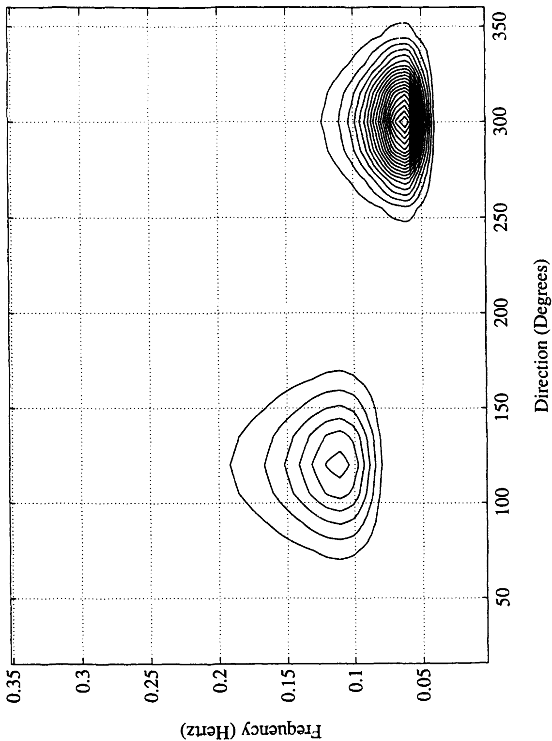
Figure B-10. Contour plot of same 3D spectra.
