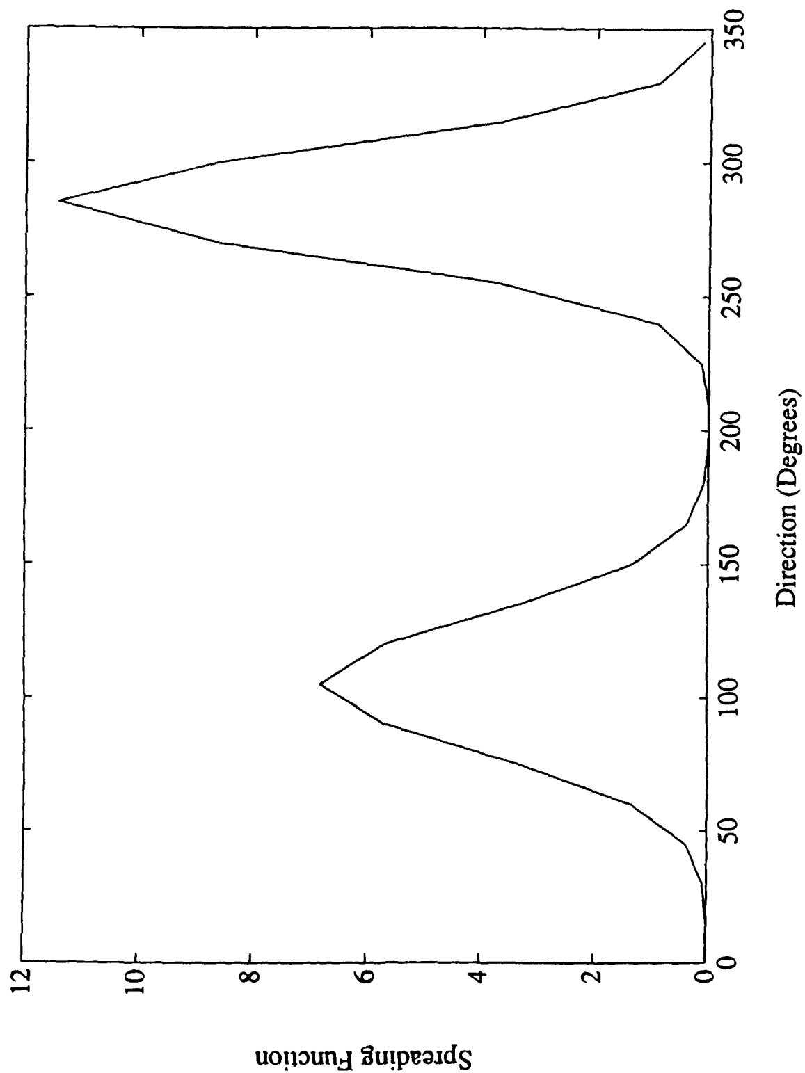
Figure C-13. Spreading function for spectra.
