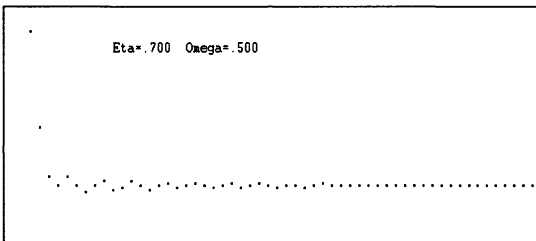
Figure III.D.3 Lower Cutoff Harmonic Ripple \omega=.5
