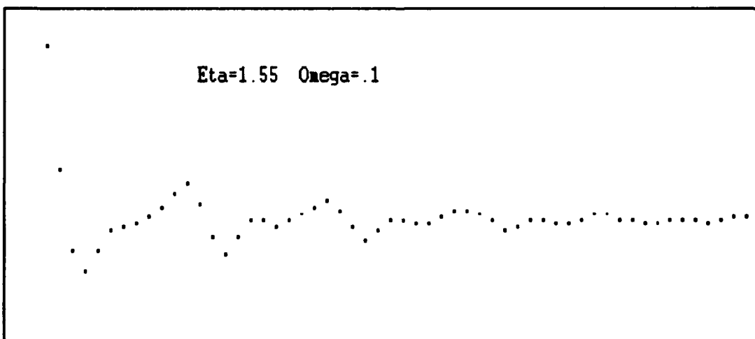
Figure III.D.8 Harmonic Ripples \omega=.1
