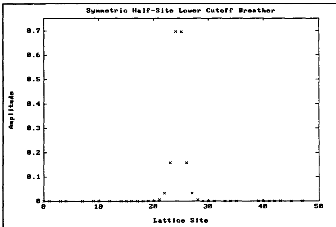
Figure III.B.5 Symmetric Half-Site Lower Cutoff Breather
