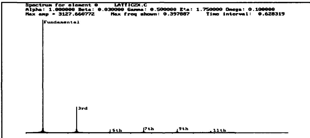
Figure III.D.7 Lower Cutoff FFT Spectrum \omega=.1
