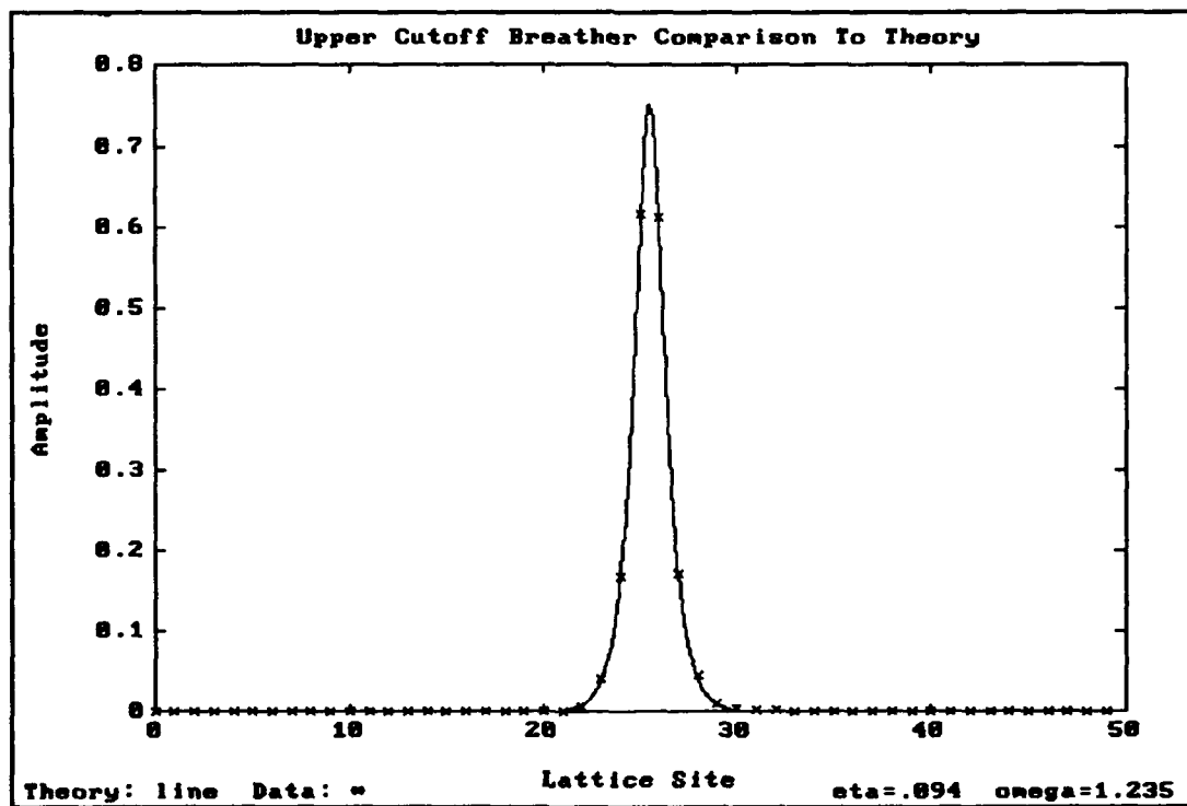
Figure III.C.8 Upper Cutoff Breather Theory Comparison
