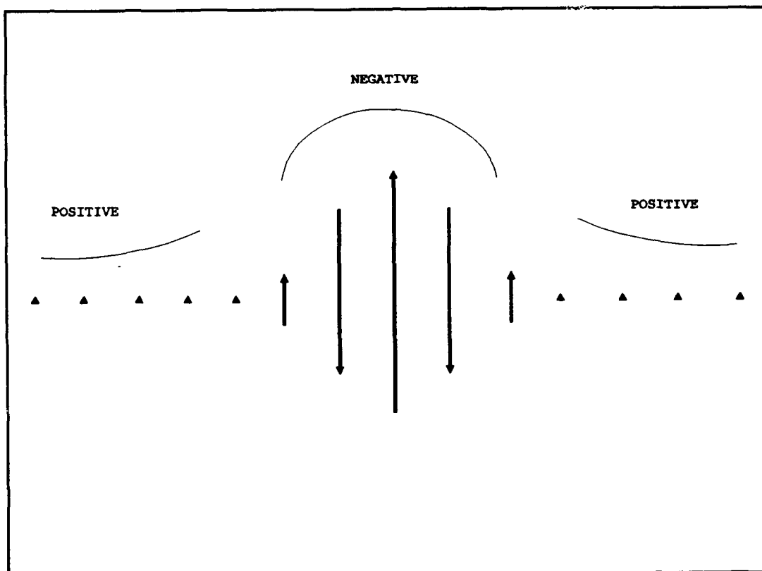
Figure II.B.1 Upper Cutoff Breather Envelope Curvatures
