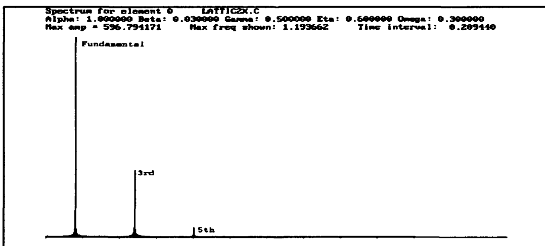
Figure III.D.4 Lower Cutoff FFT Spectrum \omega=.3
