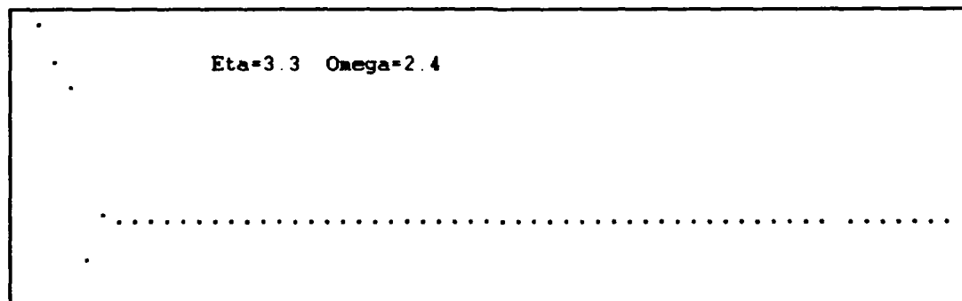
Figure III.D.15 Time Snapshot \omega=2.4
