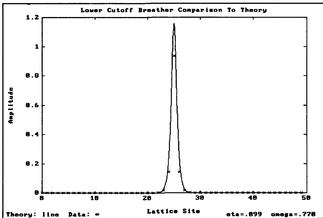
Figure III.B.7 Lower Cutoff Breather Theory Comparison
