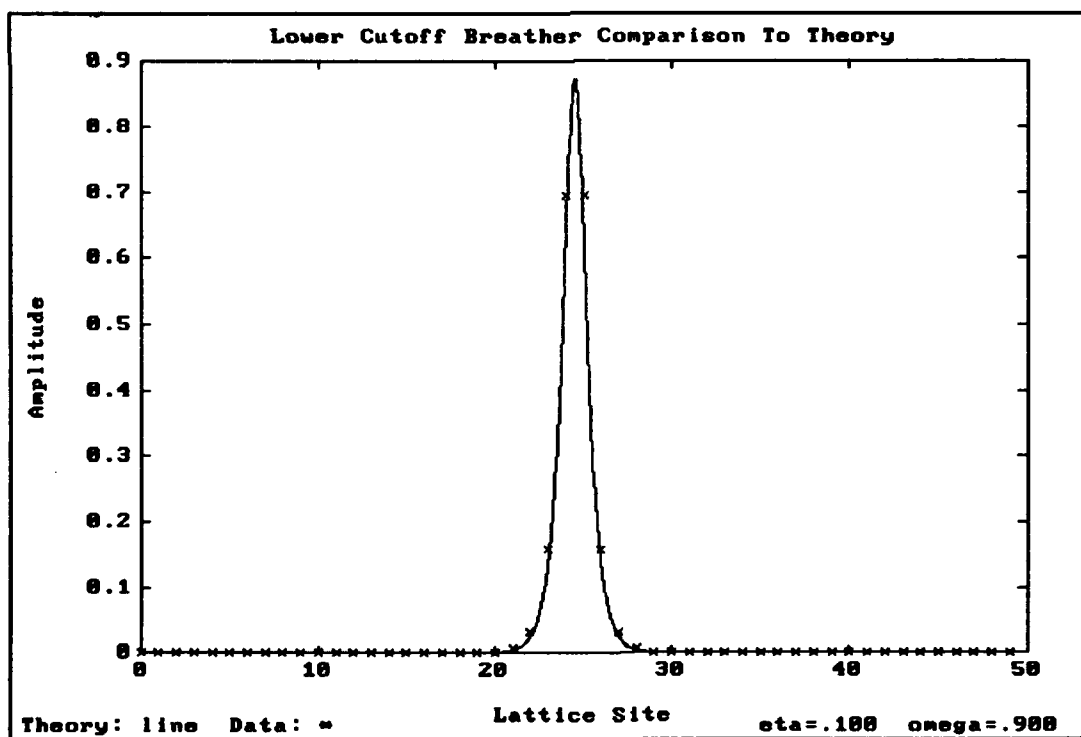
Figure III.B.8 Lower Cutoff Breather Theory Comparison
