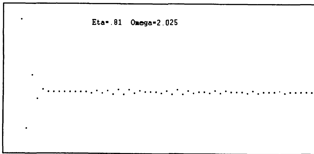
Figure III.D.11 Time Snapshot \omega = 2.025
