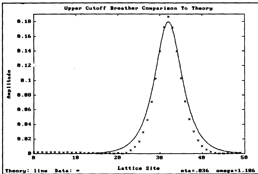
Figure III.C.7 Upper Cutoff Breather Theory Comparison
