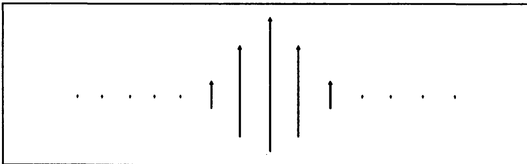
Figure I.B.3 Lower Cutoff Breather
