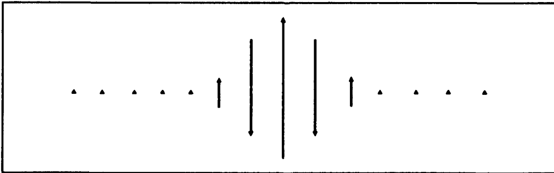
Figure I.B.4 Upper Cutoff Breather
