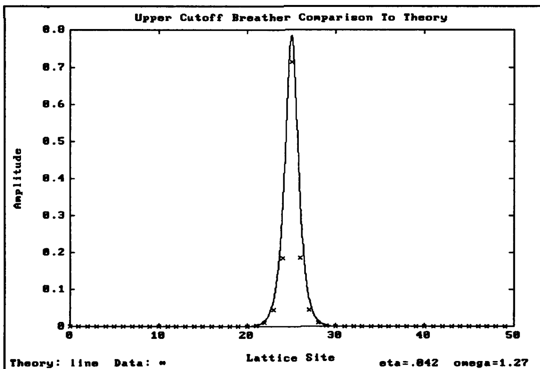
Figure III.C.6 Upper Cutoff Breather Theory Comparison
