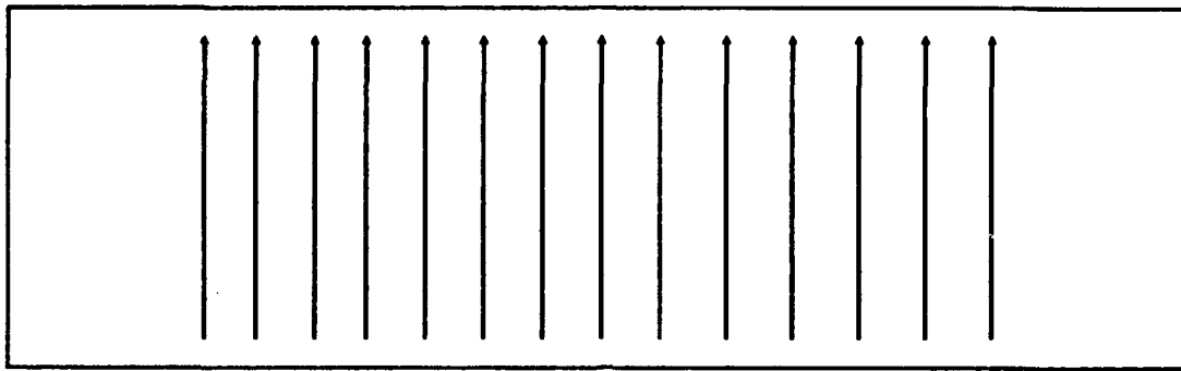
Figure I.B.1 Lower Cutoff Mode
