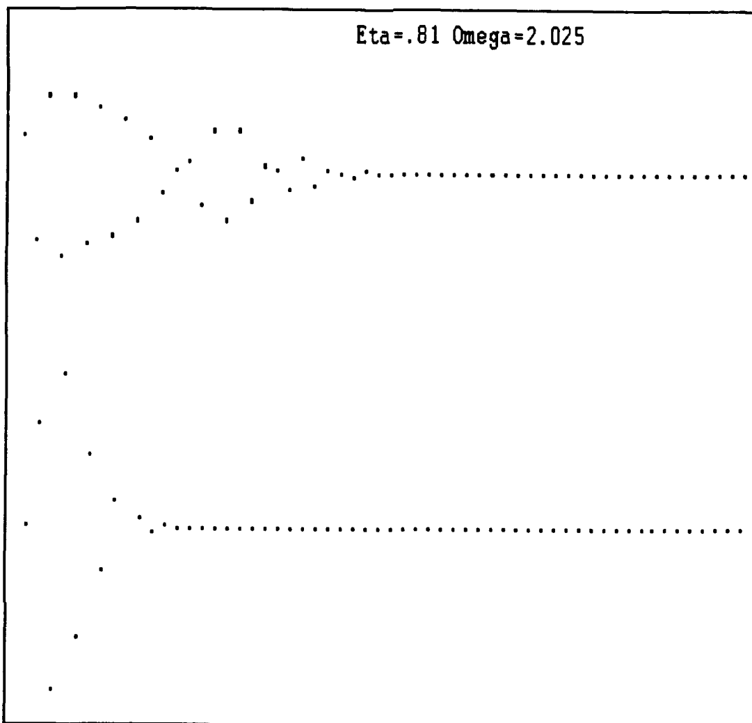
Figure III.D.10 Time Snapshots \omega = 2.025
