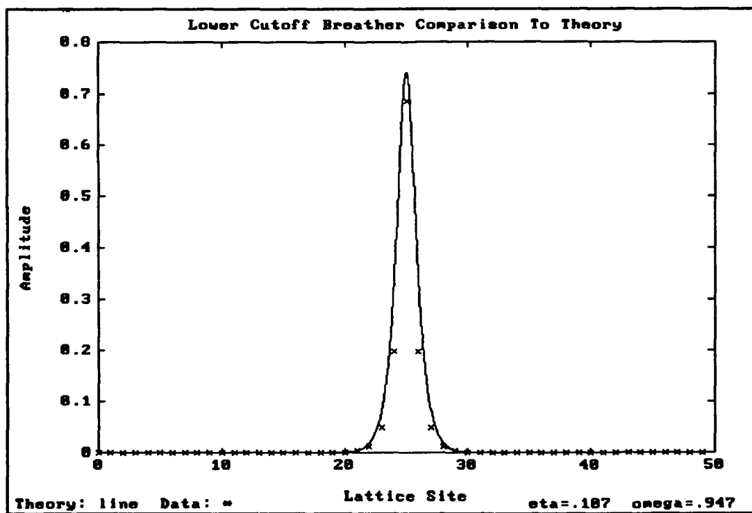
Figure III.B.6 Lower Cutoff Breather Theory Comparison
