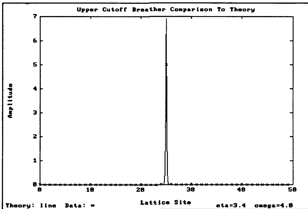
Figure III.C.5 Upper Cutoff Breather Theory Comparison
