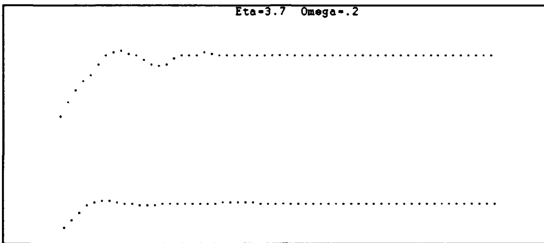
Figure III.D.6 Time Snapshots \omega=.2
