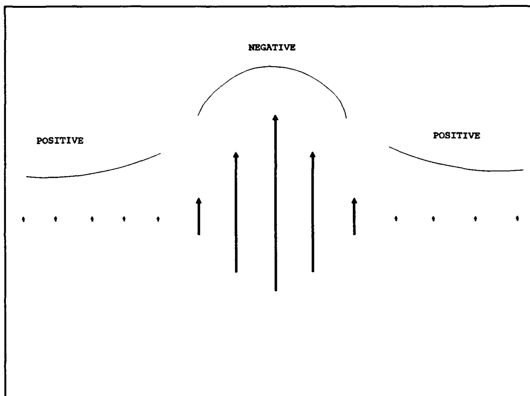
Figure II.A.1 Lower Cutoff Breather Envelope Curvatures
