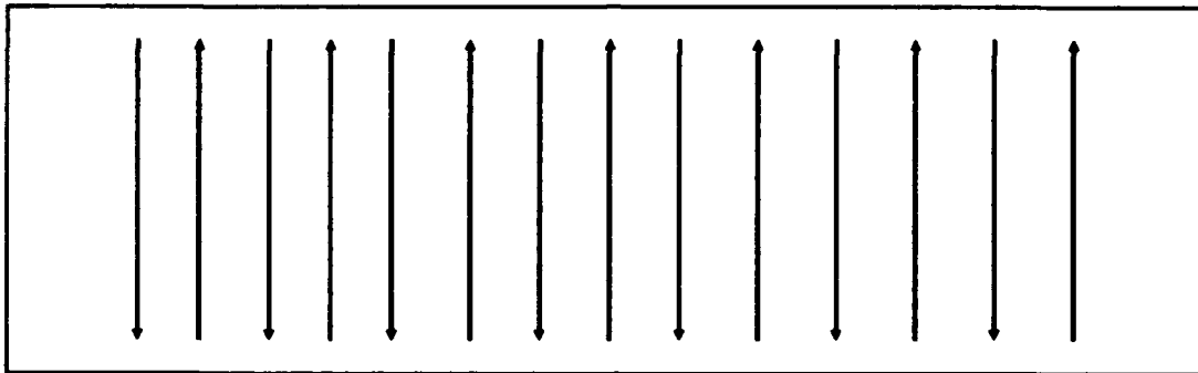
Figure I.B.2 Upper Cutoff Mode
