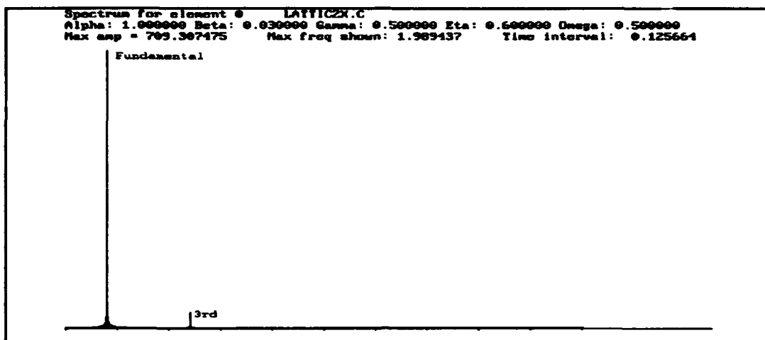
Figure III.D.2 Lower Cutoff FFT Spectrum \omega=.5
