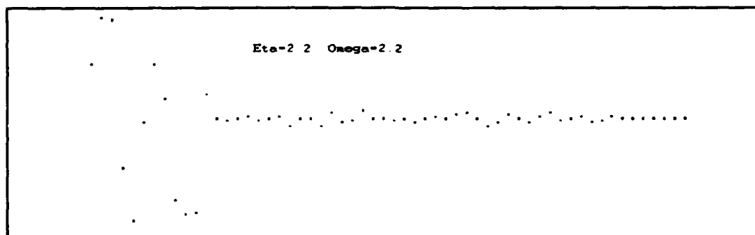
Figure III.D.13 Time Snapshot \omega=2.2
