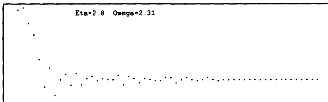
Figure III.D.14 Time Snapshot \omega=2.31
