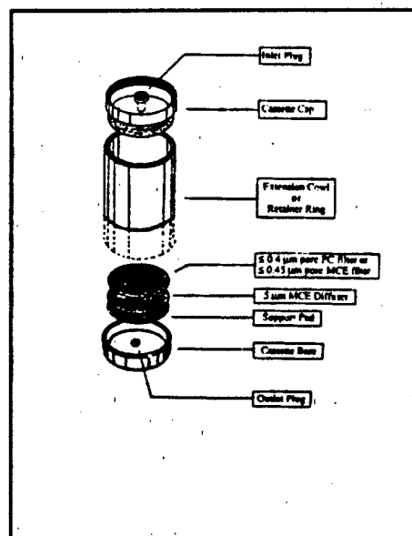
OSHA Reference Method Filter Figure 1
