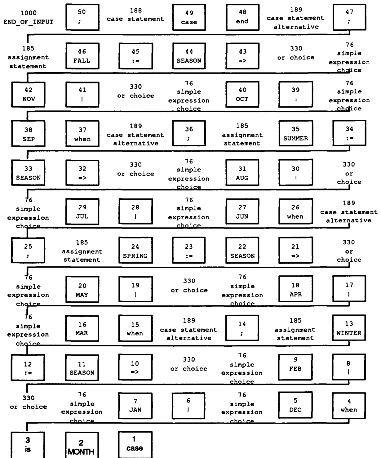
Figure 14 Expert's Meaning List
