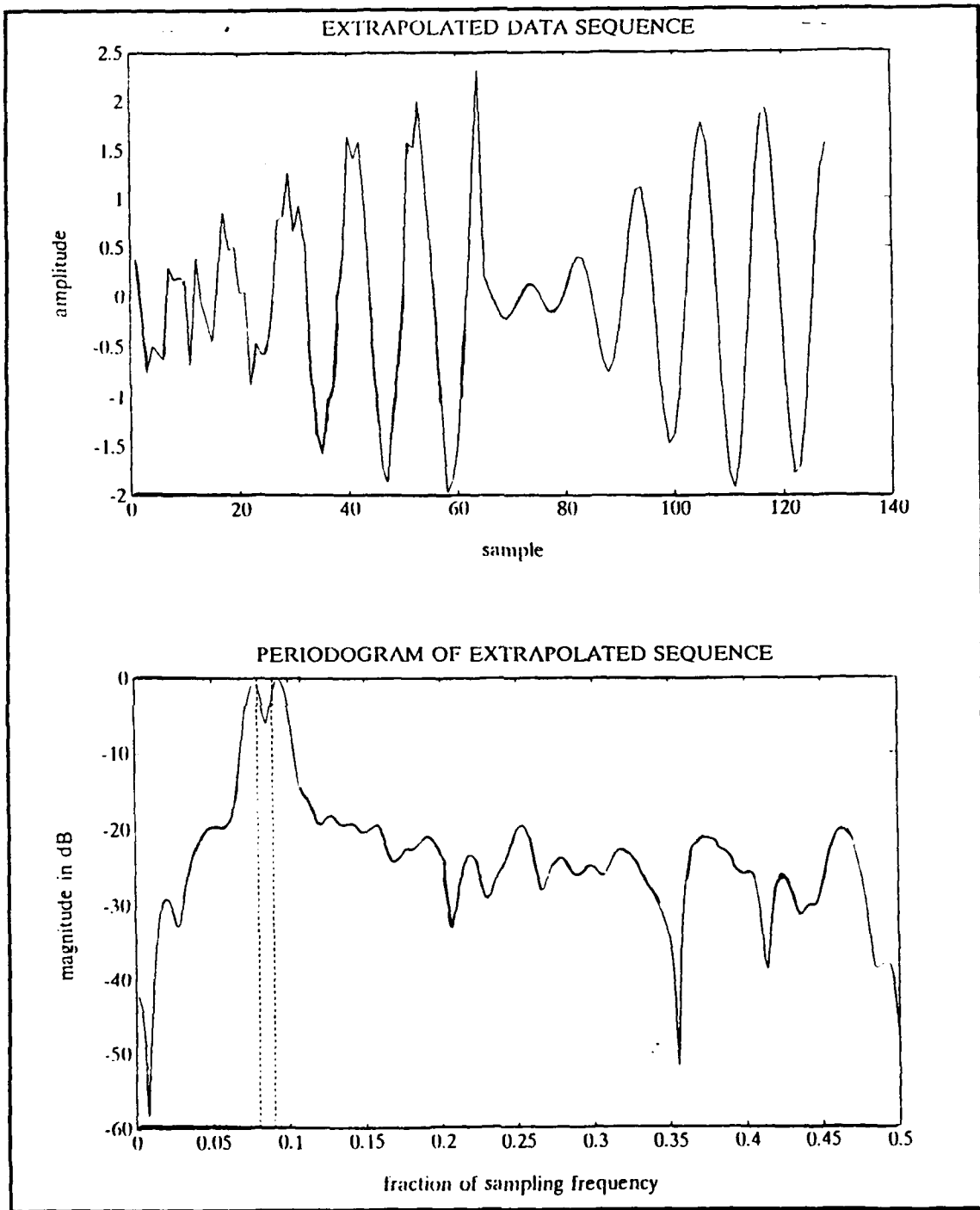
Figure 38. Eigenvector Extrapolation of Two Sine Waves, 10Hz Apart, 45° Initial Phase Angle, SNR = 15 dB, 2 Eigenvectors Used; and Resulting Periodogram
