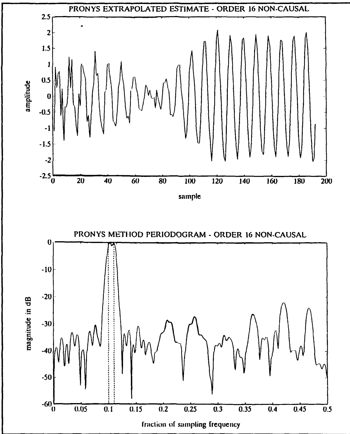
Figure 32. Extrapolated Sequence of two Sine Waves, 10 Hz Apart, 45° Initial Phase Angle, SNR = 15 dB, and Resulting Periodogram
