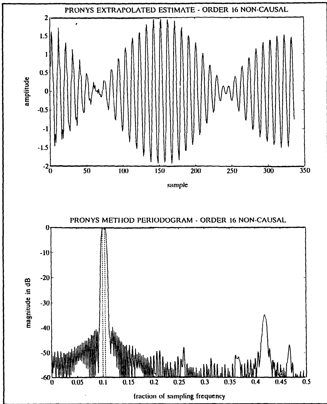
Figure 35. Extrapolated Sequence of two Sine Waves, 5 Hz Apart, 45° Initial Phase Angle, SNR = 30 dB, and Resulting Periodogram
