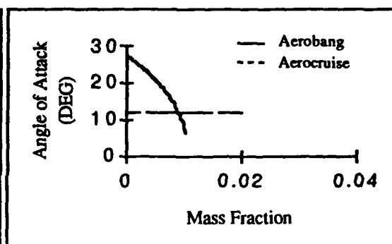
Figure 18. Angle of Attack vs Mass Fraction ERV k=.94
