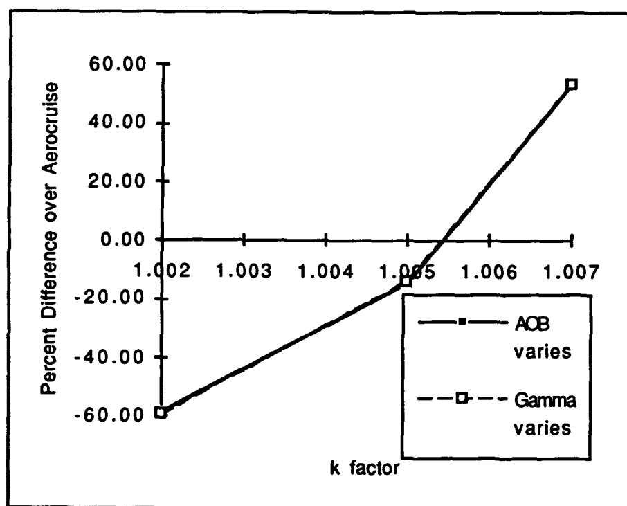
Figure 29. Fuel Percentage Difference over Aerocruise vs k Factor for MRRV (Low Heating Rate)
