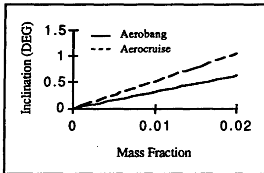
Figure 21. Inclination Change for MRRV k=.99
