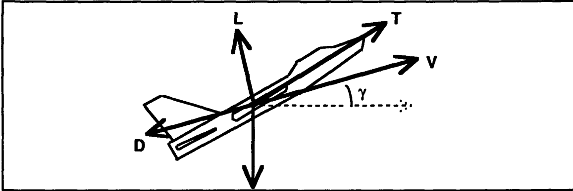
Figure 13. Spacecraft Forces During Atmospheric Interaction
