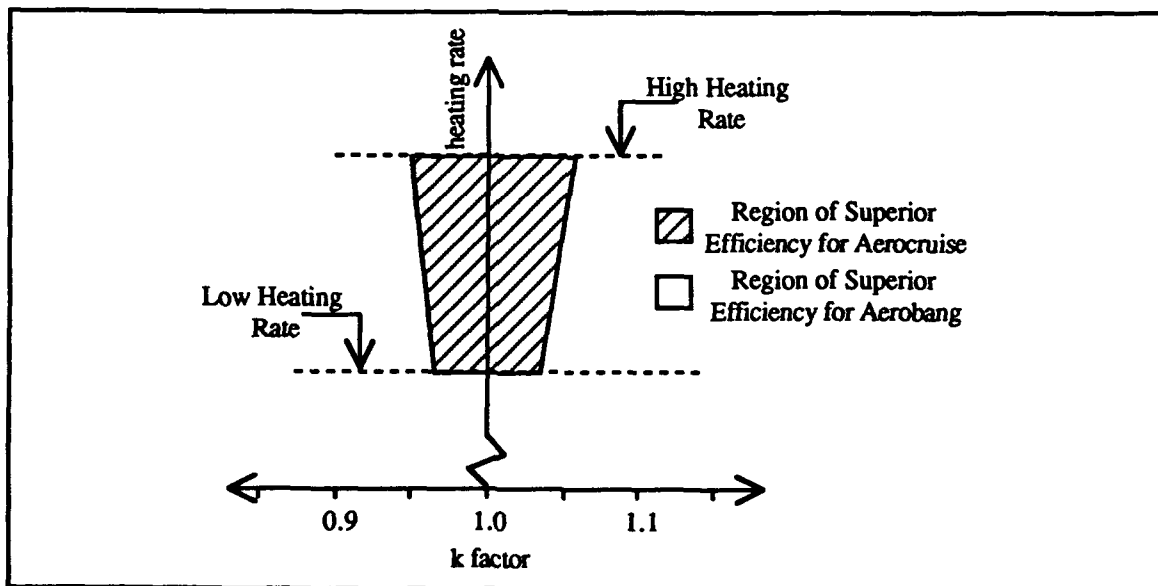
Figure 31. Efficiency Regions for the ERV
