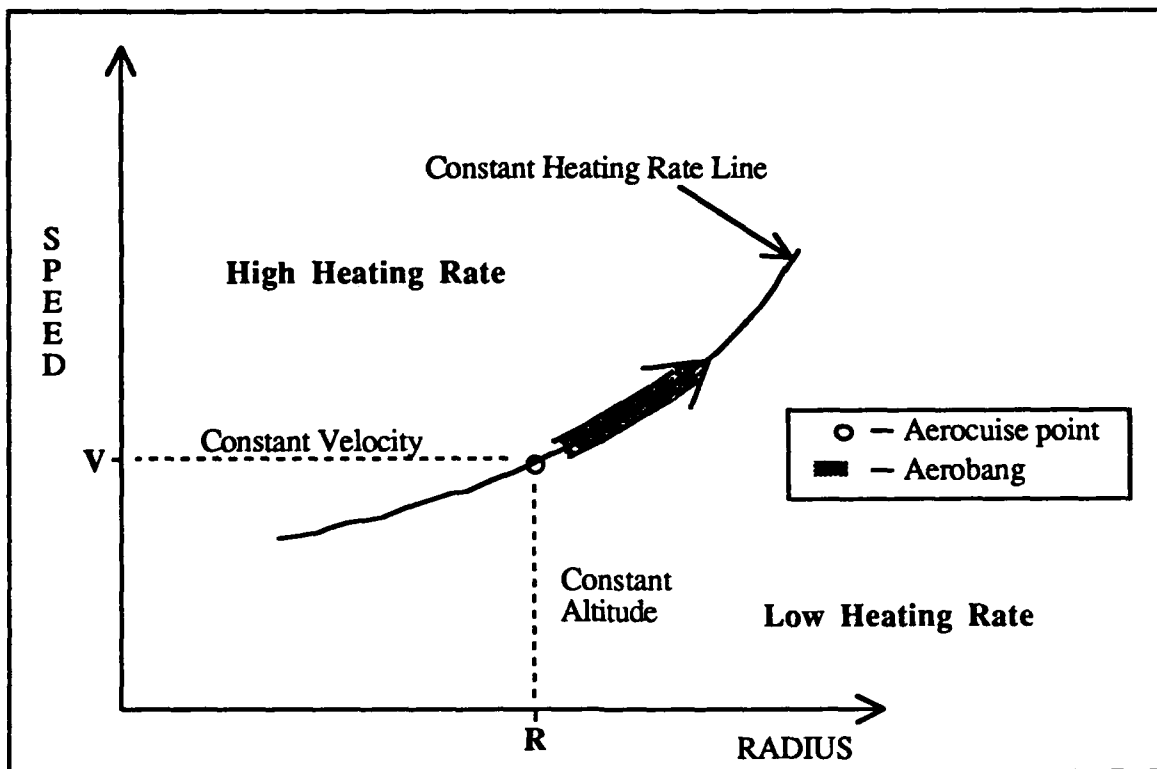
Figure 2. Heating Rate Curve
