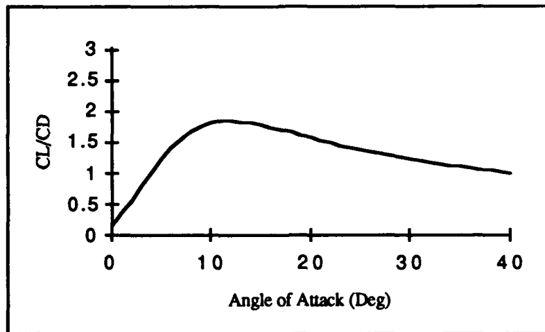
Figure 7. CL/CD vs Angle of Attack for ERV
