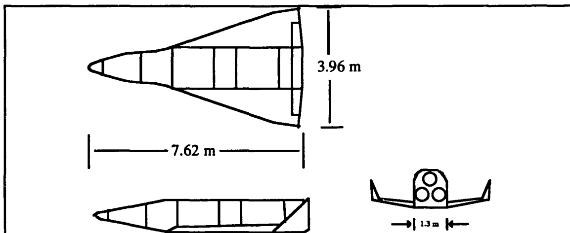
Figure 4. Three-view Diagram of ERV
