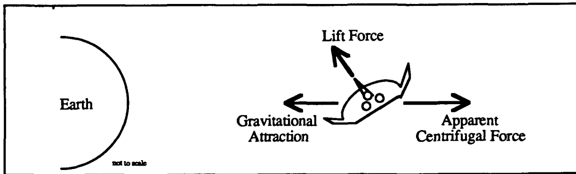
Figure 3. Graphical Representation of Aerocruise Maneuver
