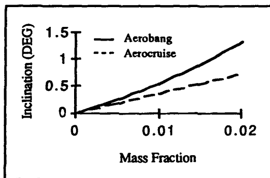
Figure 25. ERV k=1.1 Angle of Attack Profile unaugmented
