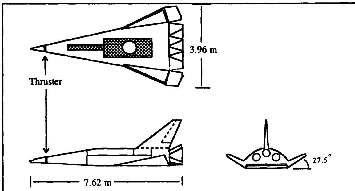
Figure 8. Three-view Diagram of MRRV
