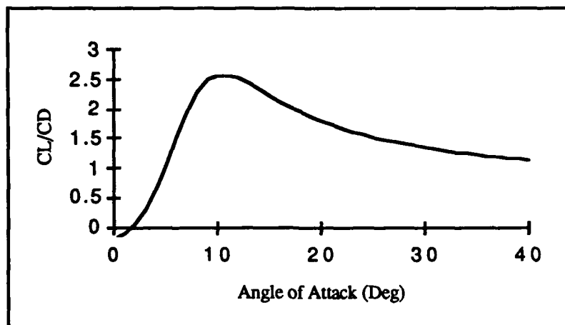
Figure 11. C_L/C_D vs Angle of Attack for MRRV
