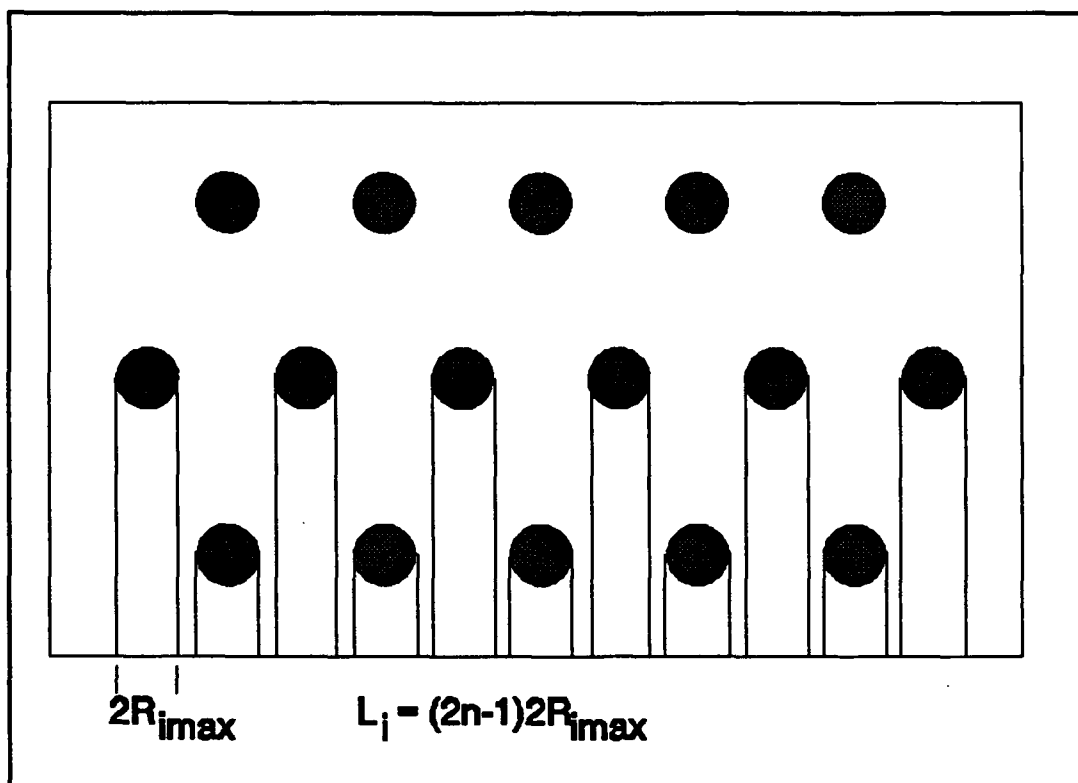
Figure 8. Equivalent Pattern Sweep Width When R_{imax} \leq 1/4 Buoy Spacing
