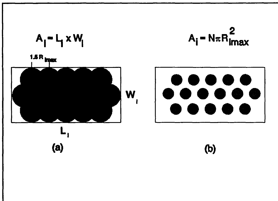
Figure 7. Initial Areas Covered by Pattern When Buoy Coverage Areas (a) Overlap and (b) Don't Overlap
