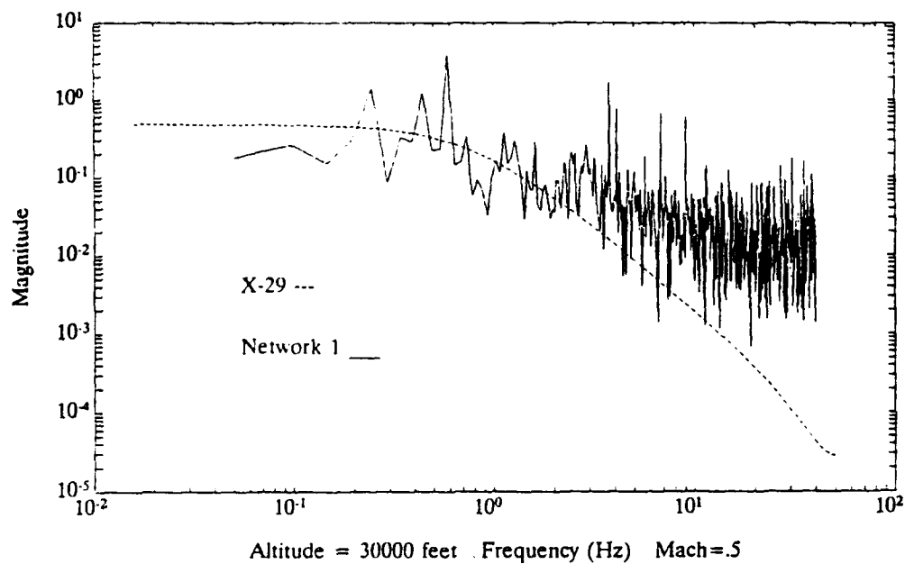
Figure 77 X-29 Plant Model and Network 1 \alpha Frequency Responses to Input 1
