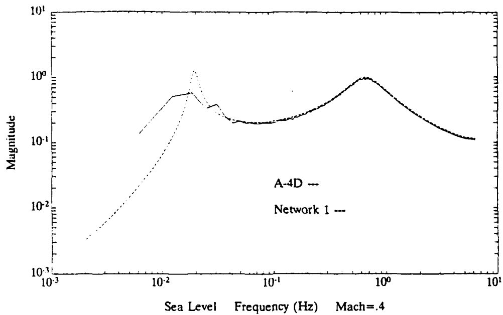
Figure 69 A-4D Plant Model and Network 1 q Frequency Responses
