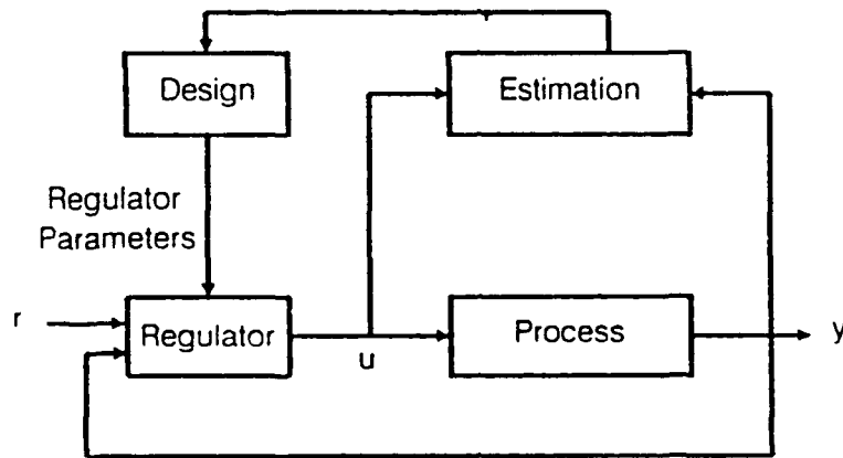
Figure 7 Self-Tuning Regulator Control Block Diagram
