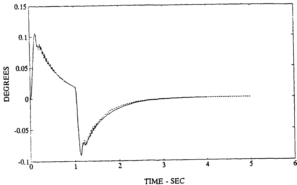
Figure 43 X-29 Model and Network \alpha Time Responses to Input 2 (Optimal case)
