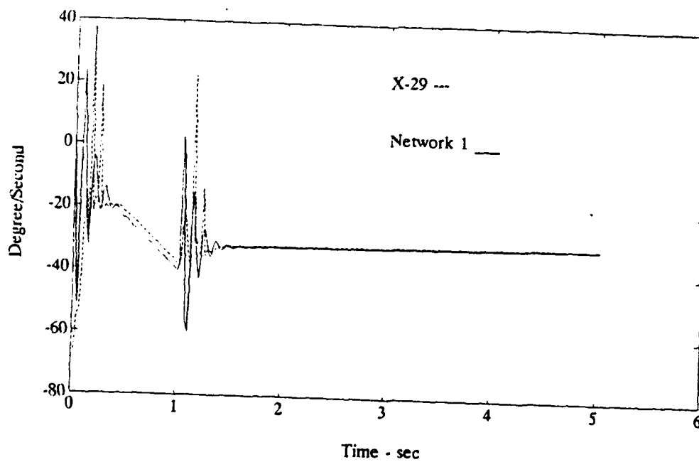
Figure 87 X-29 Optimal Controller Model and Network 1 \dot{q} Time Responses to Input 2 ( 1 Hidden layer )
