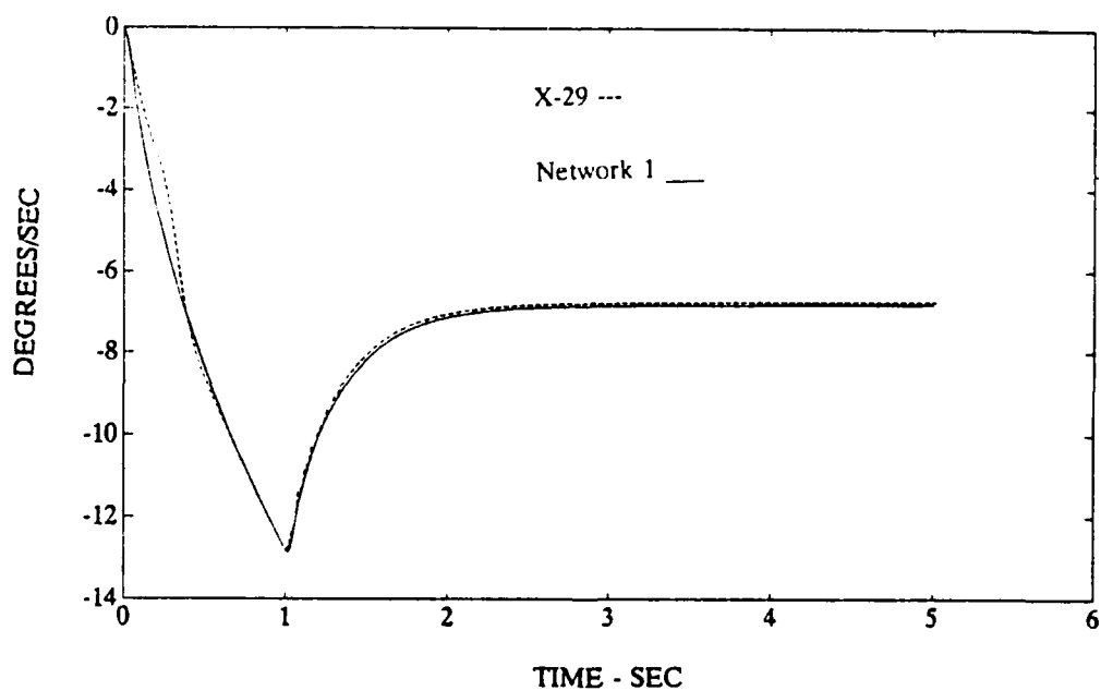
Figure 99 X-29 Limited Controller Model and Network 1 \dot{\alpha} Time Responses to Input 1
