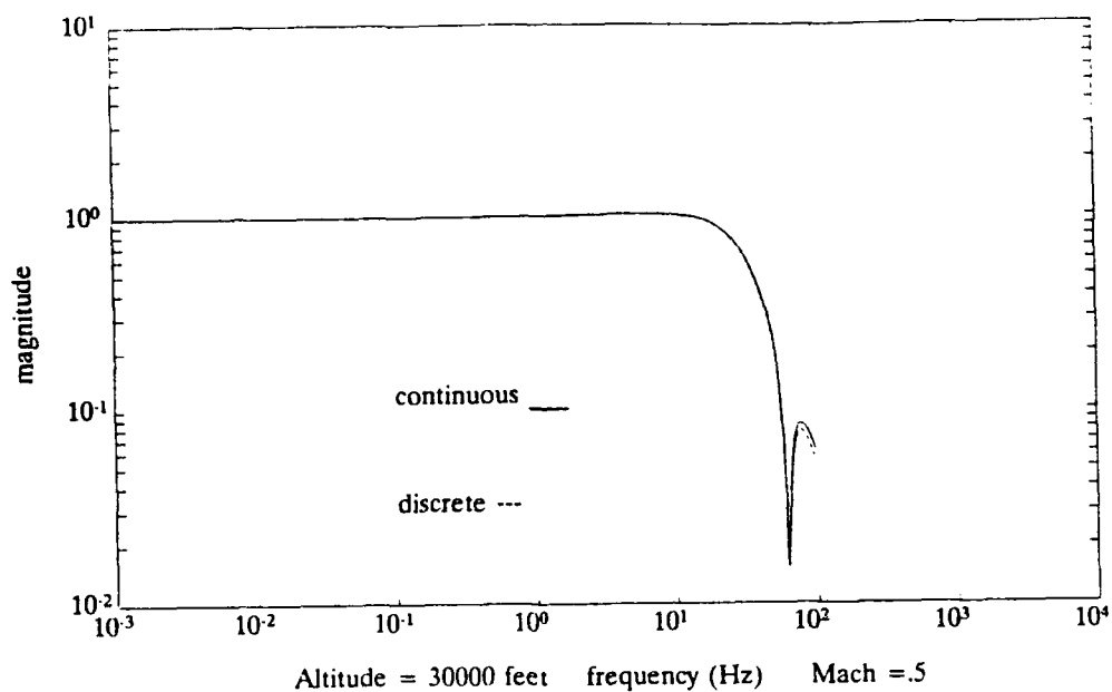
Figure 15 Continuous and Discrete \alpha Frequency Responses to Input 1 (Optimal case)
