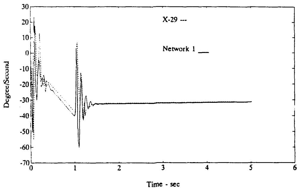
Figure 95 X-29 Optimal Controller Model and Network 1 q Time Responses to Input 2 ( 2 Hidden layer )
