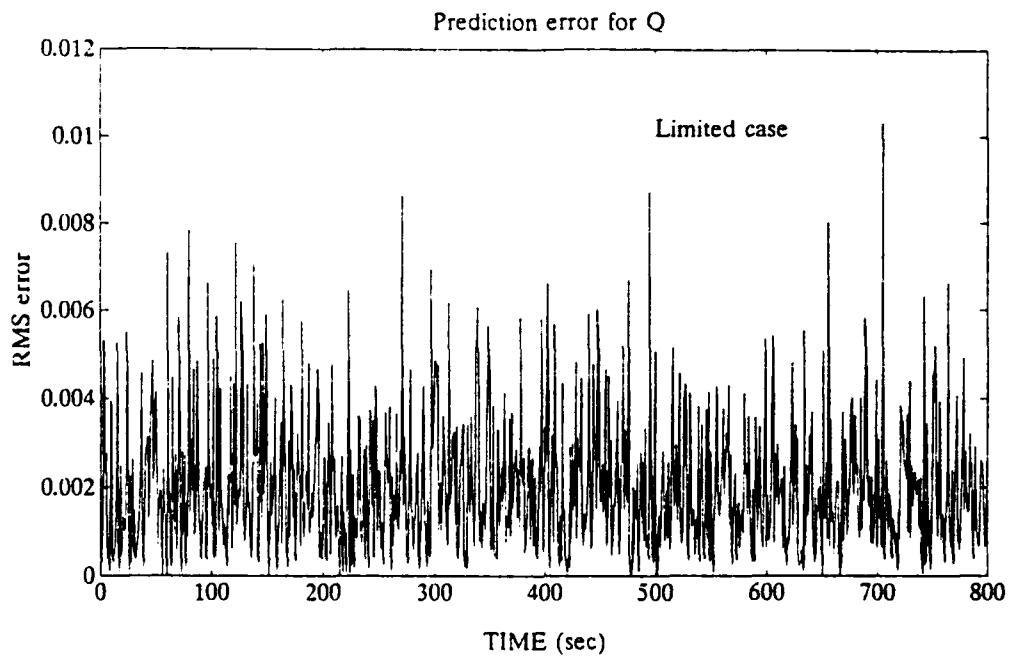
Figure 50 RMS Prediction Errors for q
