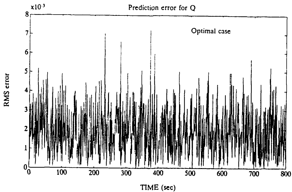
Figure 40 RMS Prediction Errors for q
