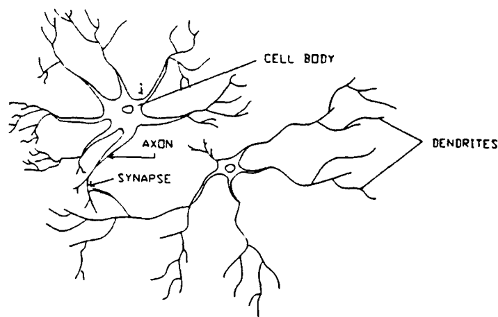
Figure 1 Biological Neuron
