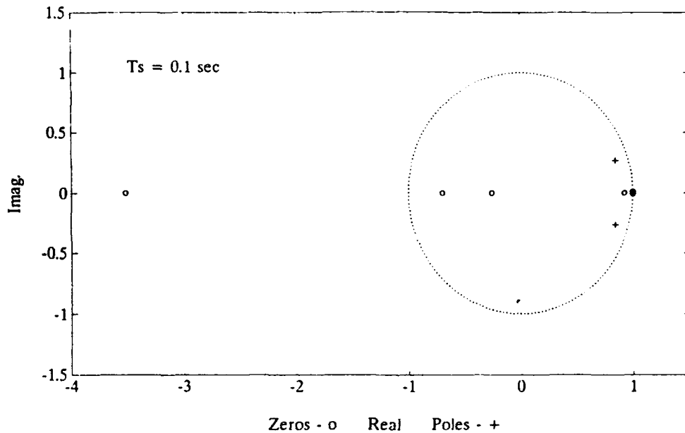
Figure 30 Poles and Zeros of the A-4D Plant
