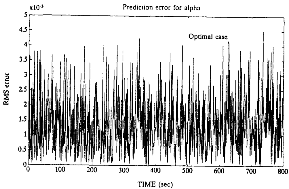
Figure 39 RMS Prediction Errors for \alpha
