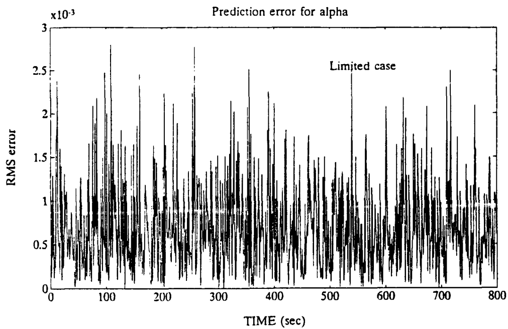
Figure 49 RMS Prediction Errors for \alpha
