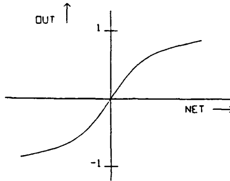
Figure 6 Hyperbolic Tangent Function
