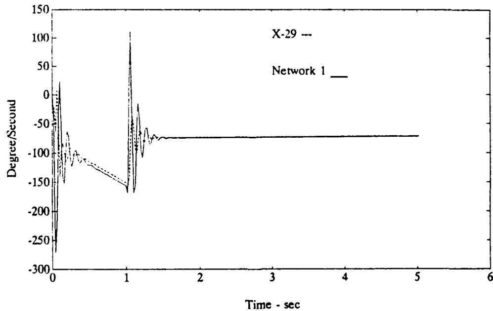
Figure 93 X-29 Optimal Controller Model and Network 1 \dot{\alpha} Time Responses to Input 1 ( 2 Hidden layer )
