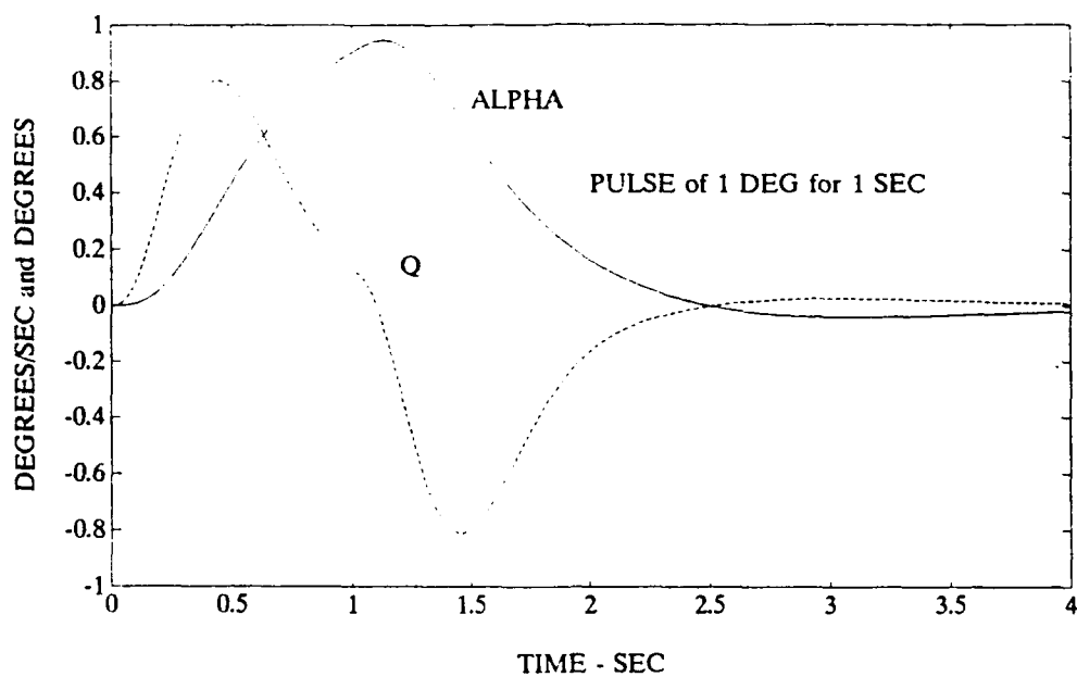
Figure 19 Q and \alpha Time Responses to Input 1 (Limited case)
