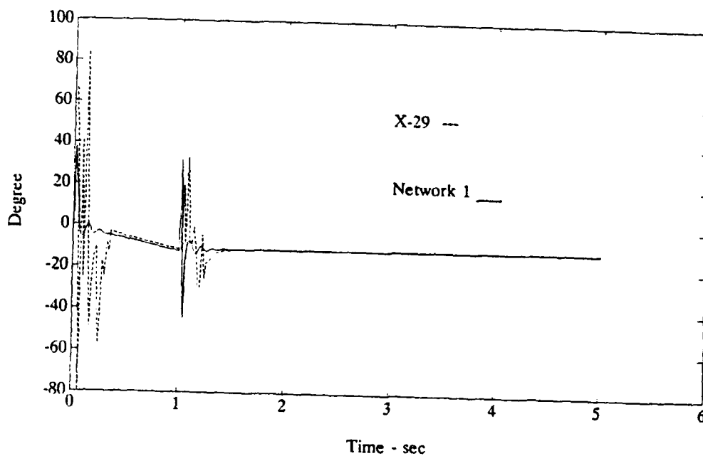
Figure 86 X-29 Optimal Controller Model and Network 1 \alpha Time Responses to Input 2 ( 1 Hidden layer )
