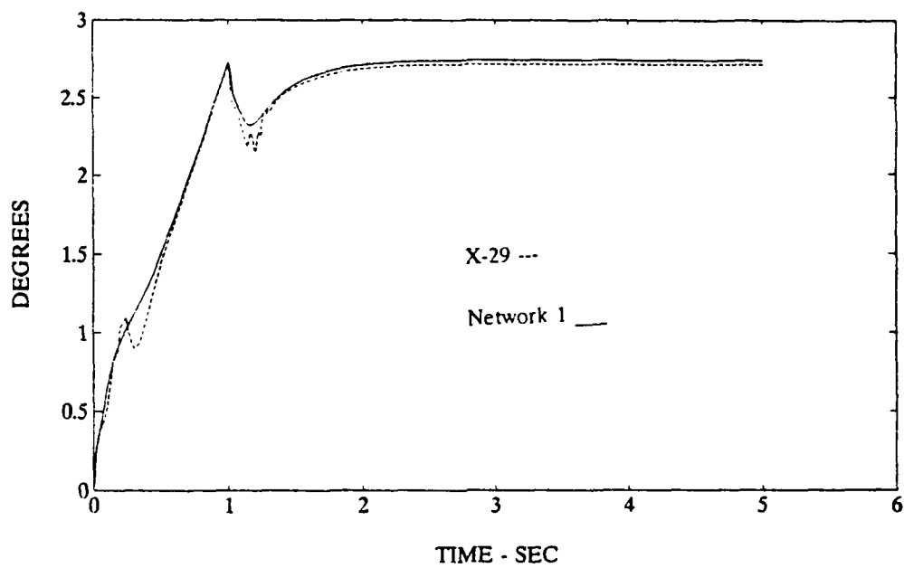
Figure 100 X-29 Limited Controller Model and Network 1 \alpha Time Responses to Input 2
