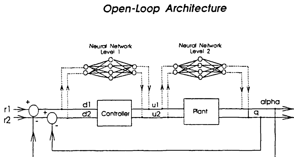
Figure 33 Open-Loop Architecture
