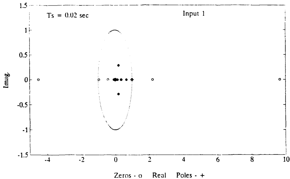
Figure 31 Poles and Zeros of the X-29 Plant
