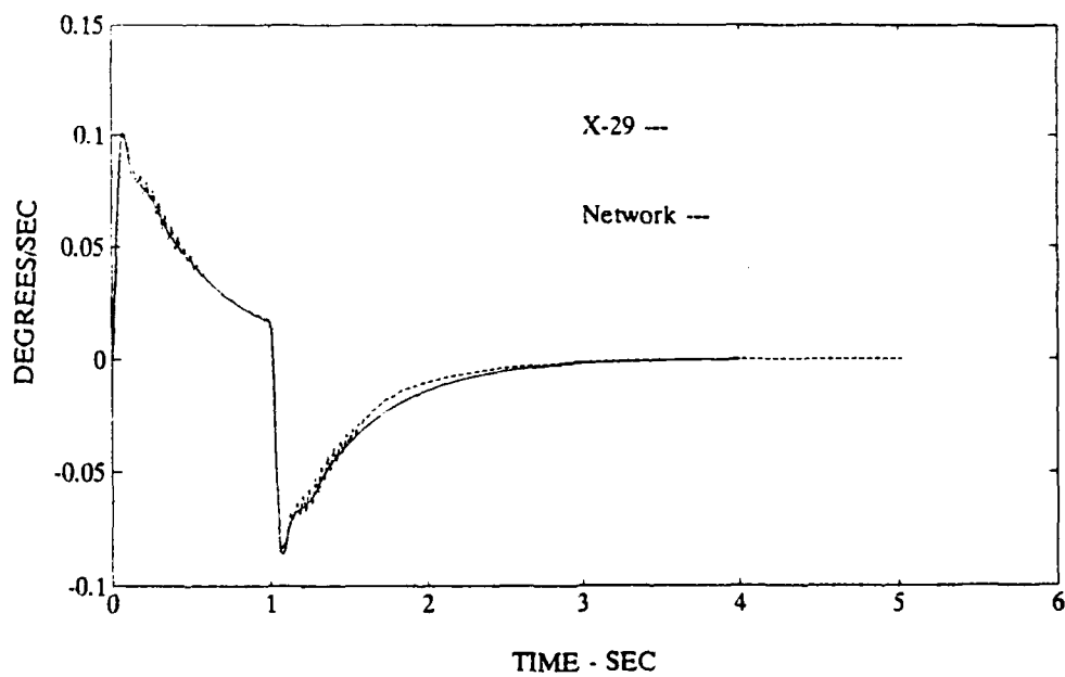
Figure 42 X-29 Model and Network q Time Responses to Input 1 (Optimal case)
