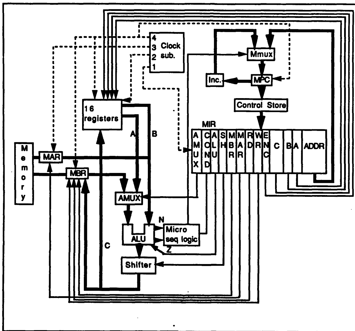
Figure 3.2 Tanenbaum's Microarchitecture (Tanenbaum, 1984, p. 132)
