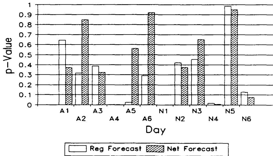
Figure 4.10 Paired Difference p-Values
