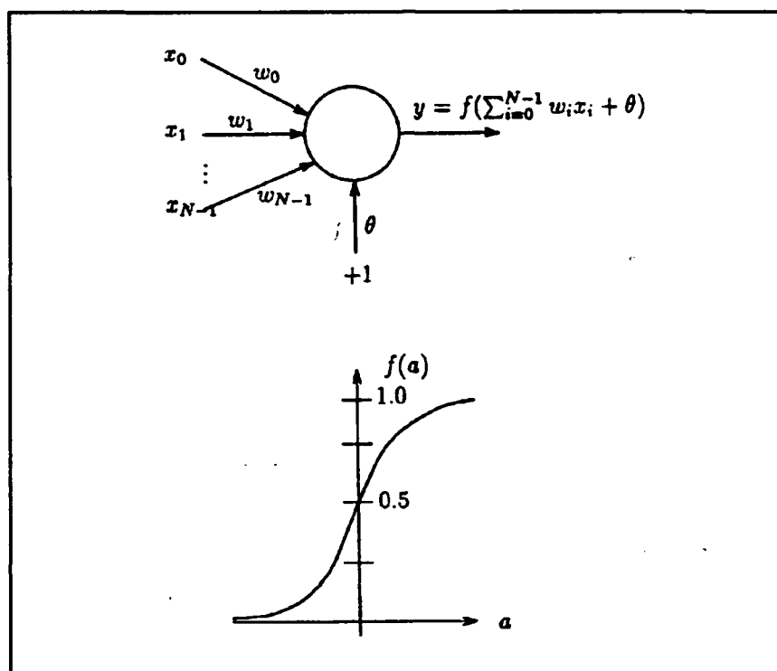
Figure 2.3 The Perceptron (Rogers et al., 1990:49)
