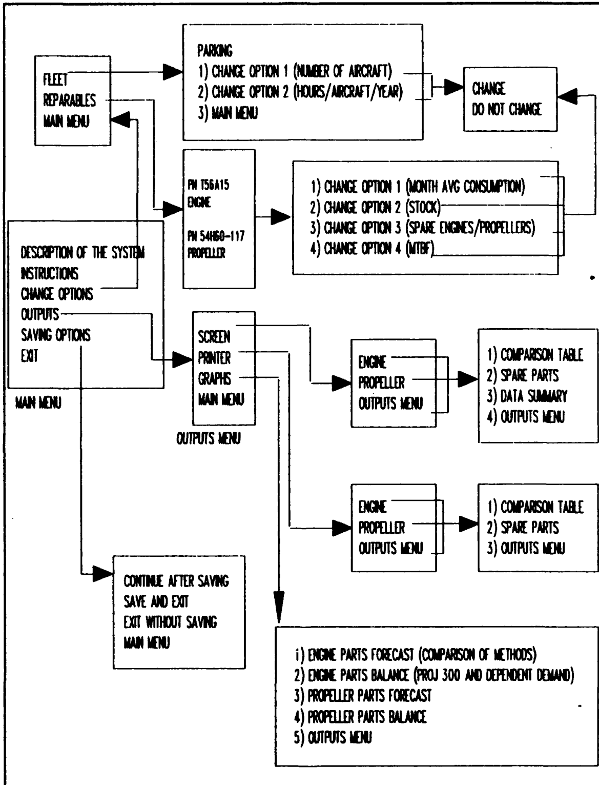
Figure 3. Menu Structure
