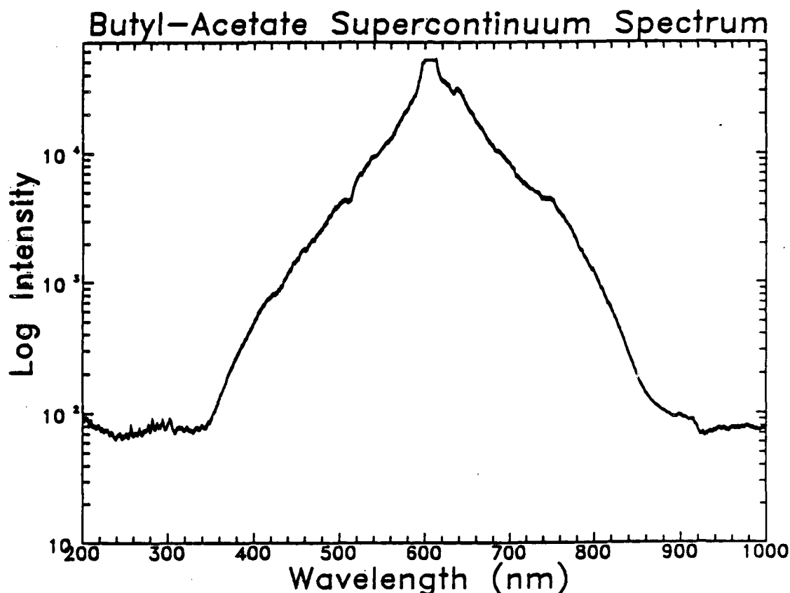
Fig. 2. Spectrum of the supercontinuum produced by focusing \sim 1/3 mJ, 50 fs pulses ( \gamma \approx 620\text{nm} ) into butyl acetate.
