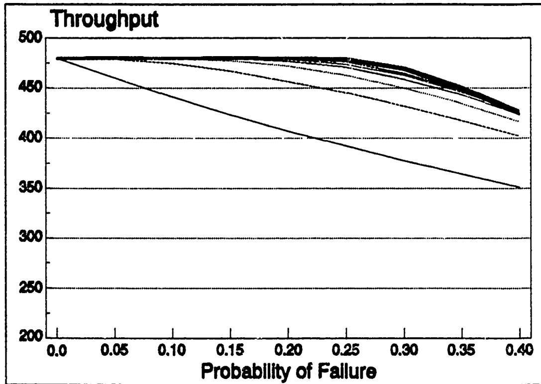
Figure 4-6. System 1 - JIT - Station Failure
