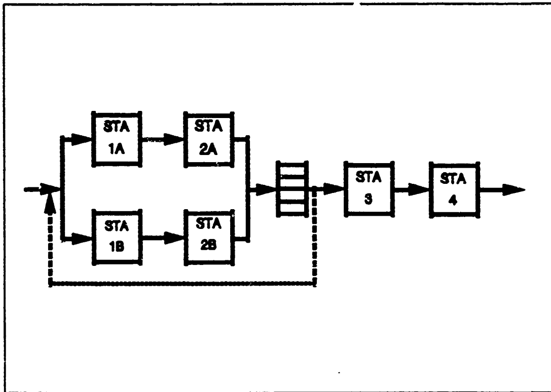
Figure 3-8. System 2 - Drum-Buffer-Rope
