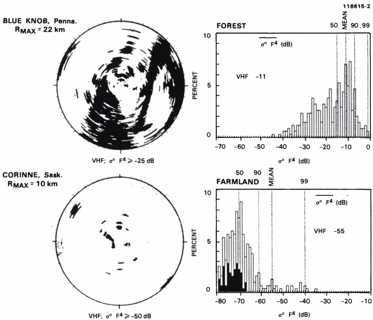
Figure 18. VHF ground clutter in steep forest and level farmland. Histograms show repeat sector data. In the PPI clutter maps, cells containing clutter stronger than the indicated threshold are shown as black.
