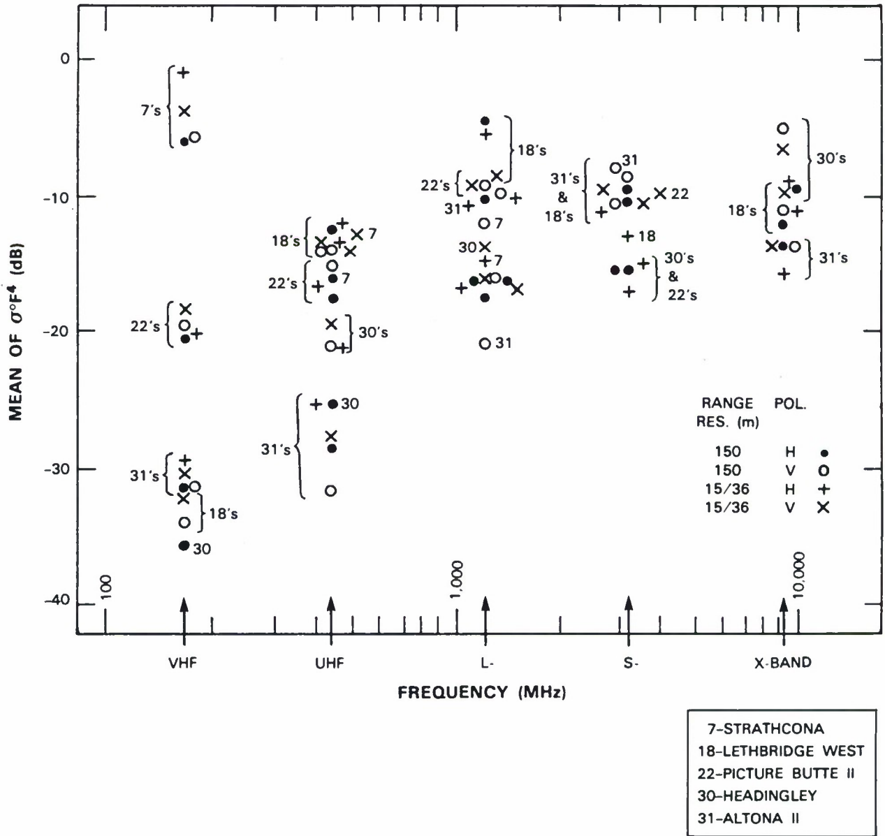
Figure 23. Mean clutter strength versus frequency for urban terrain. See Table 7.
