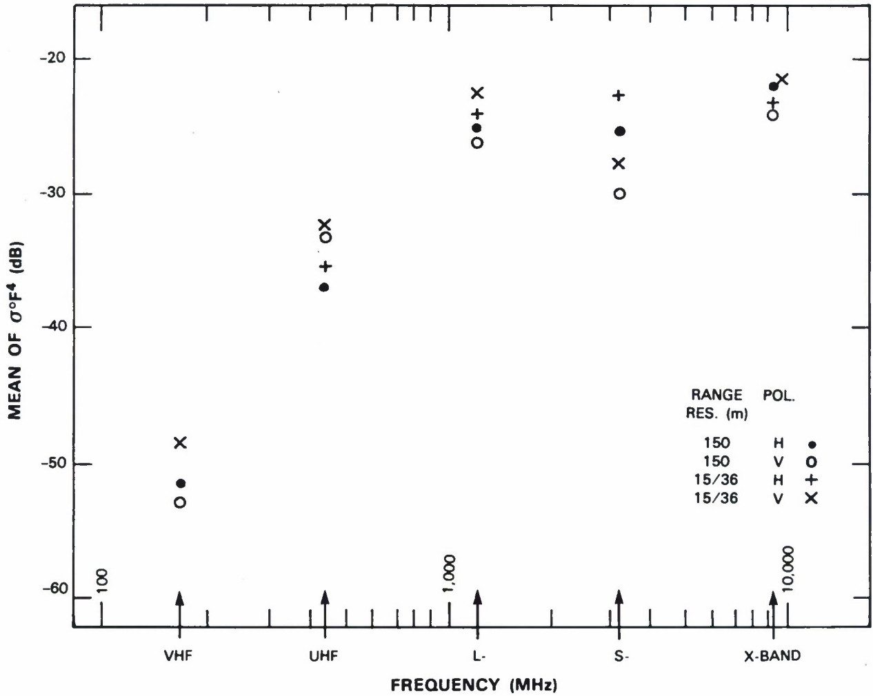
Figure 92. Mean clutter strength versus frequency at Suffield.
