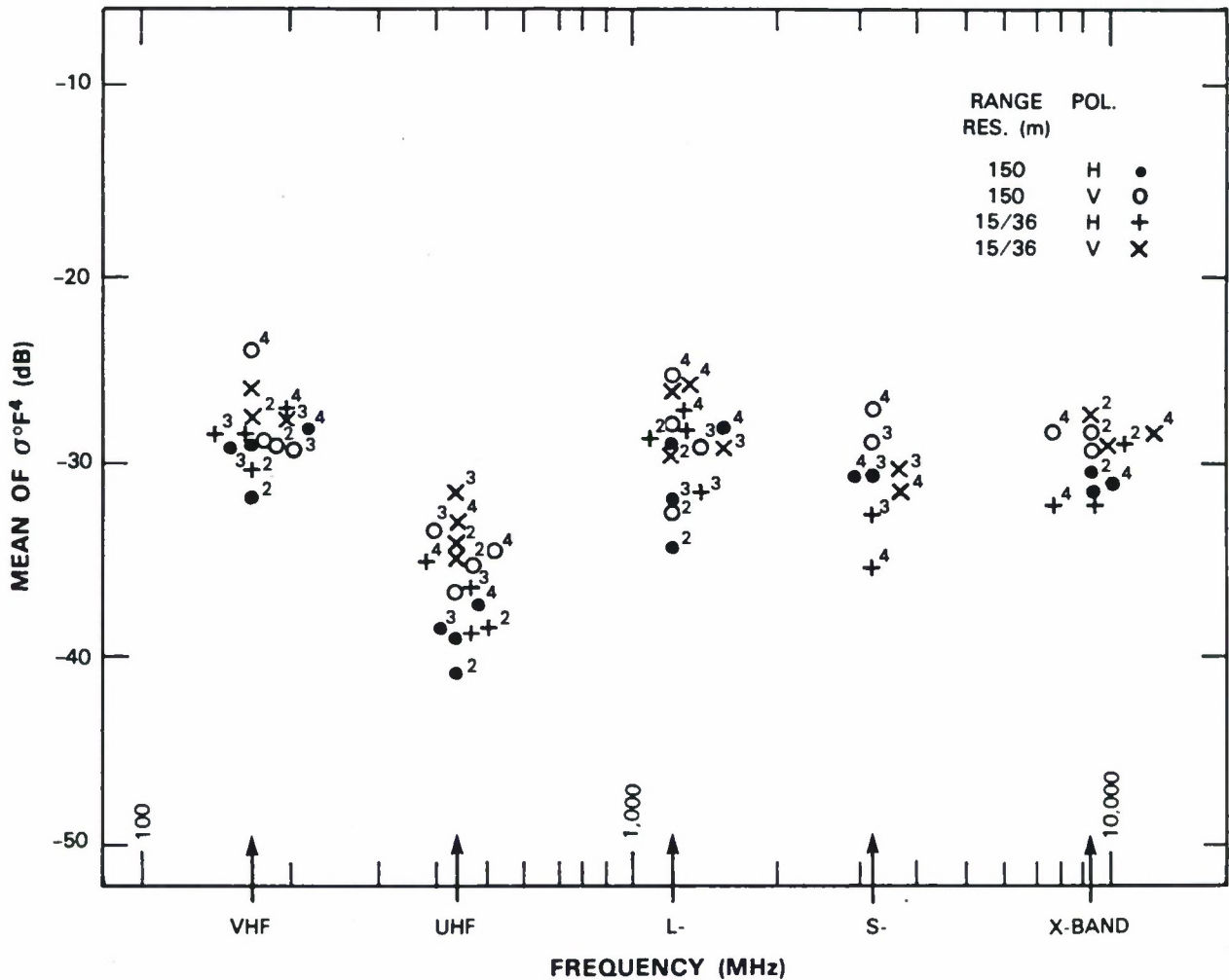
Figure 67. Seasonal variations in mean clutter strength at Beiseker. Repeat sector data. First visit, fall (18 October to 13 November 1982). Second visit, winter (12 February to 24 February 1983). Third visit, summer (6 August to 24 August 1983). Fourth visit, late fall (16 November to 26 November 1983). Second, third, and fourth visit results indicated by superscripts to the upper right.
