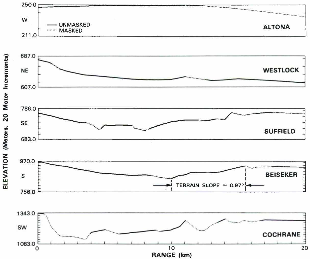
Figure 10. Terrain elevations and masking in five Phase One repeat sectors. (a) Antenna mast height = 50 ft; adaptive ordinate. Data from 1:50,000 scale topographic maps.
