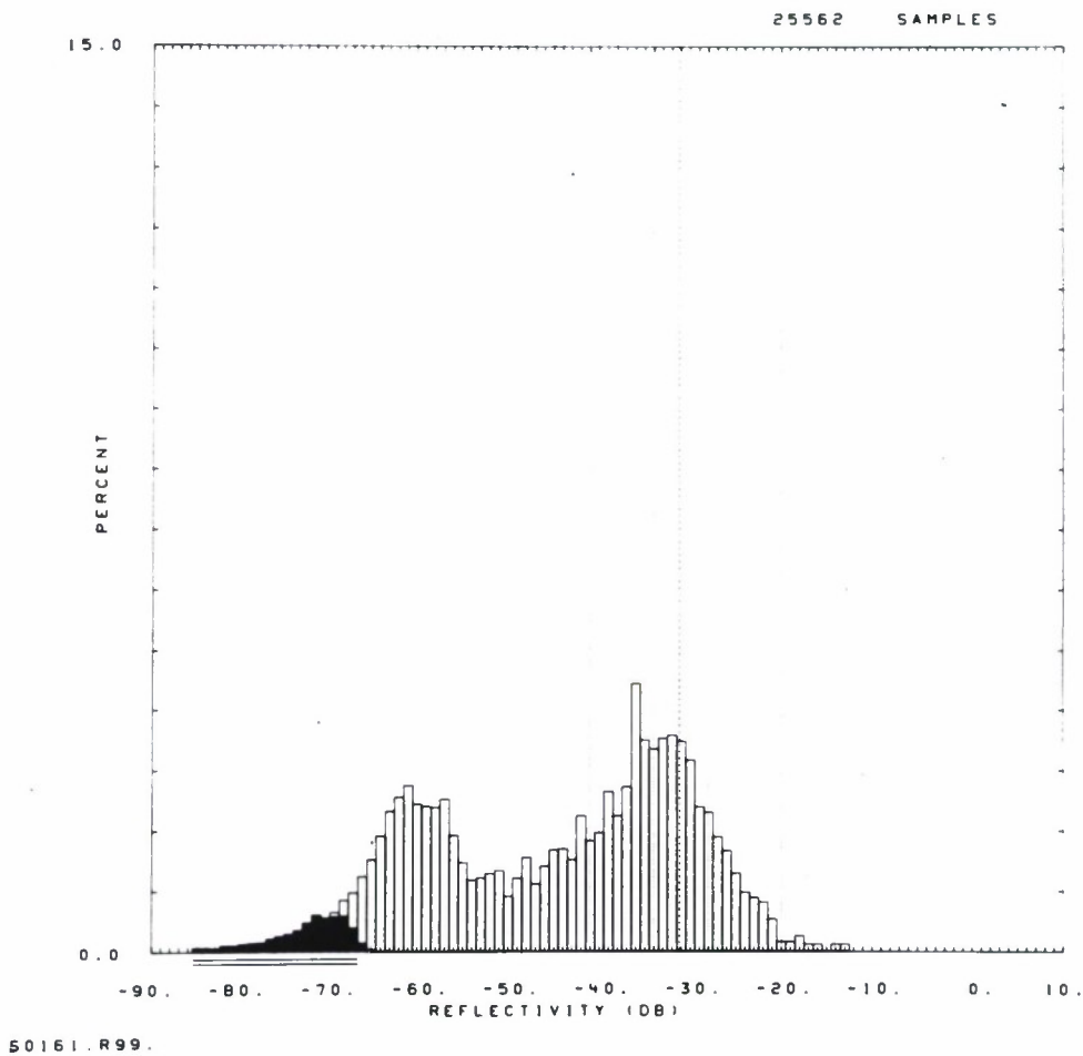
Figure 8. Histograms of clutter amplitude statistics at X-band over the Gull Lake West repeat sector. (b) 150-m range resolution, horizontal polarization, measured 20 February 1984.
