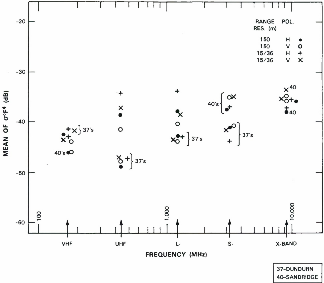
Figure 50. Mean clutter strength versus frequency for forest/low-relief terrain at low depression angle. See Table 7.
