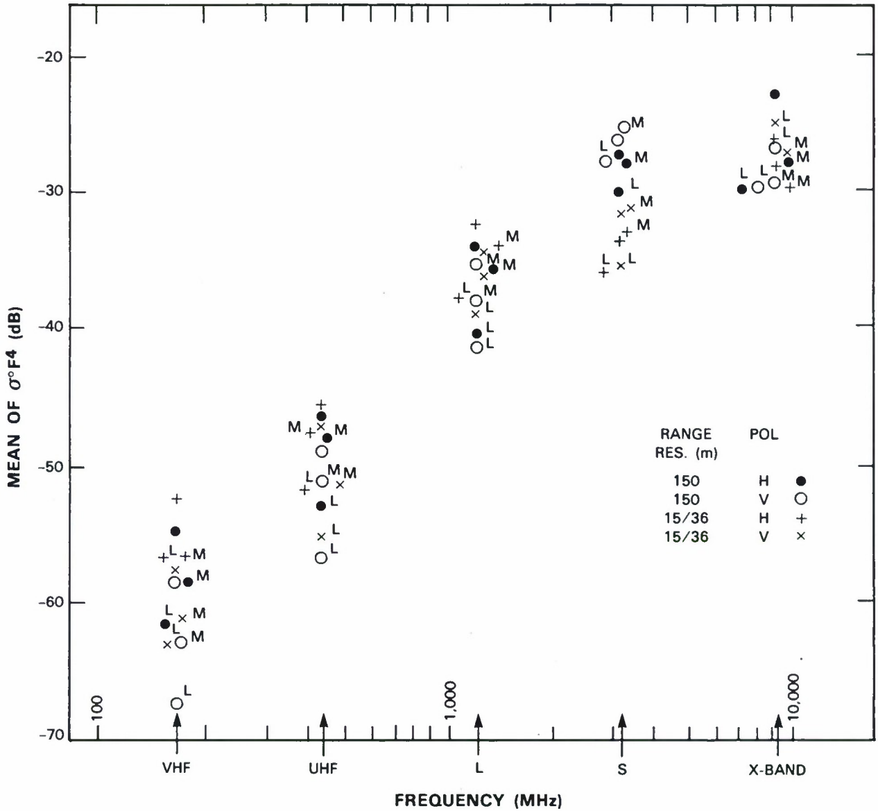
Figure 78. Mean clutter strength versus frequency at Corinne for three antenna heights. Repeat sector data; level farmland; antenna heights = 54 – 59 ft (3 tower sections, no superscript), = 41 – 46 ft (2 tower sections, superscript "M"), and = 27 – 32 ft (1 tower section, superscript "L"), see Table A-5; at S-band, the high resolution range interval (4.0 – 8.9 km) is shorter than that for the other 18 frequency band/waveform combinations (1.0 – 8.9 km).
