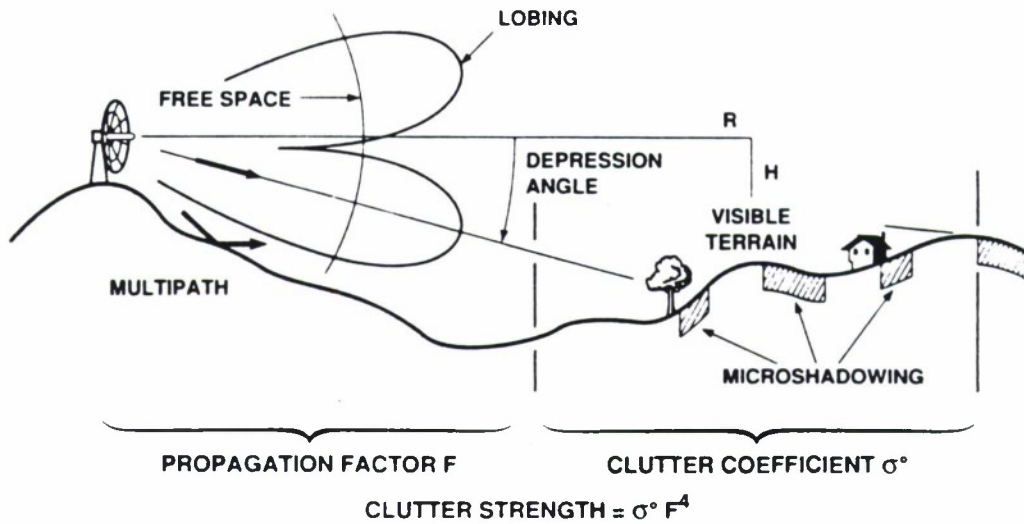
Figure 15. Clutter physics.
