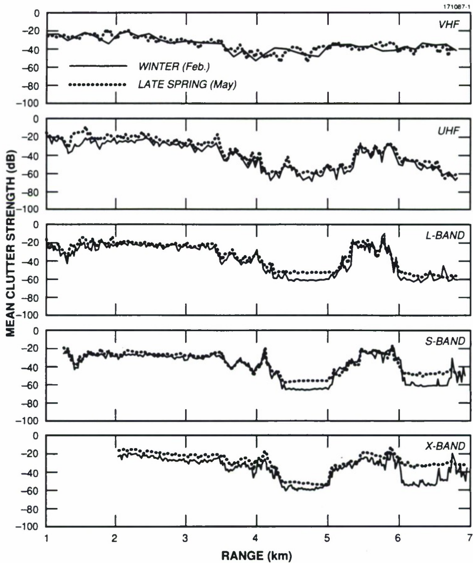
Figure 7. Seasonal variation in mean clutter strength versus range for five frequency bands at Gull Lake West, Manitoba. Repeat sector data; level forest and forested wetland with lake edges; winter visit in February 1984 (solid lines), spring visit in May 1984 (dotted lines); vertical polarization, high range resolution data, except VHF winter visit where low range resolution data are shown.
