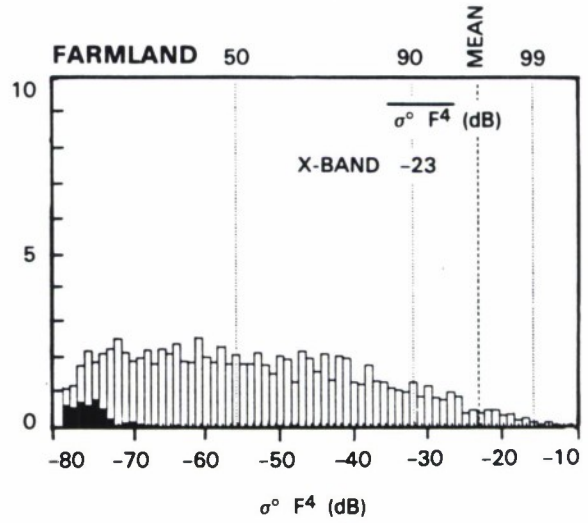
Figure 17. X-band ground clutter in steep forest and level farmland. Histograms show repeat sector data. In the PPI clutter maps, cells with \sigma^{\circ} F^4 \geq -50 dB are shown as black.
