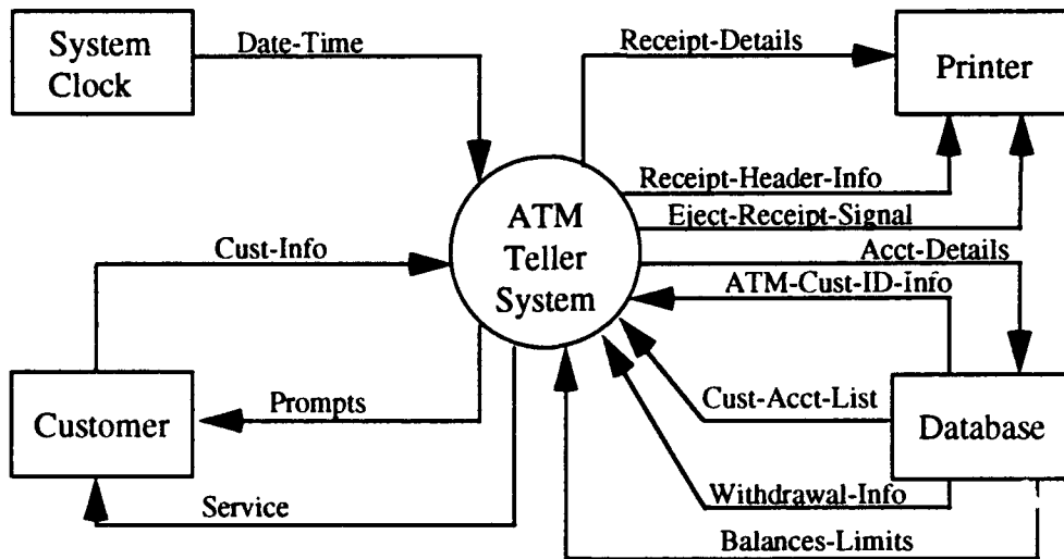
Figure 2: Context Diagram
