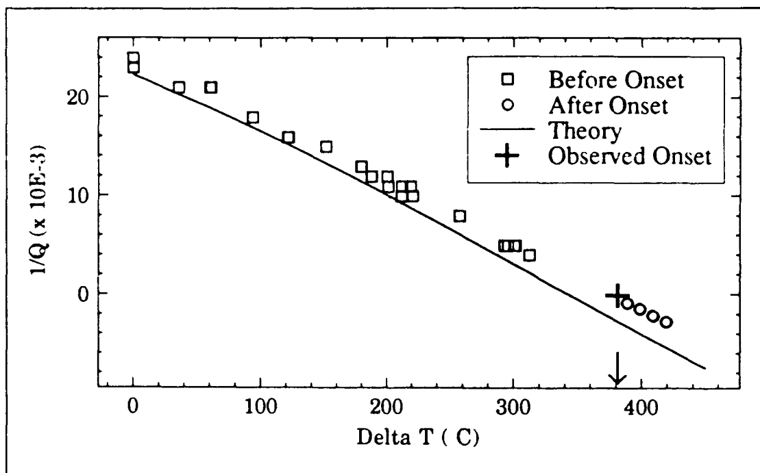
Figure 12. Plot of combined 1/Q vs \Delta T_m data obtained below and immediately after onset. P = 205\text{ kPa} .
