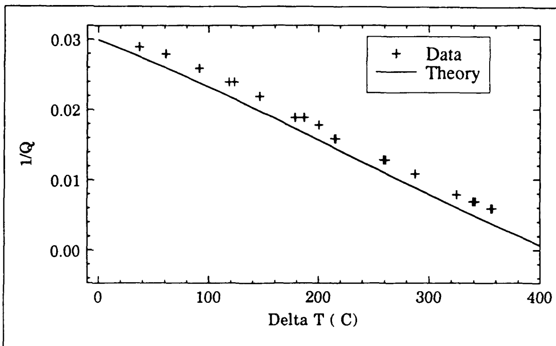
Figure 14. Plot of 1/Q vs \Delta T_m for data obtained below onset in the second mode. P = 80 \text{ kPa} .
