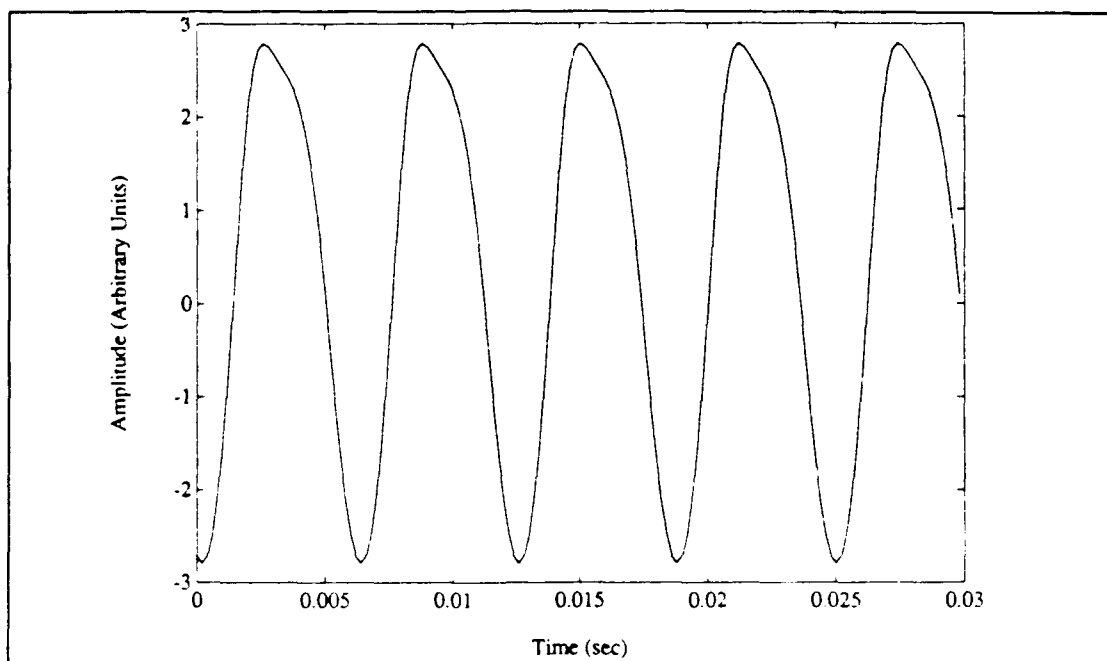
Figure 35. Plot of waveform obtained at steady state. P = 207.7 \text{ kPa} . \Delta T_m = 416.5 \text{ }^{\circ}\text{C} .
