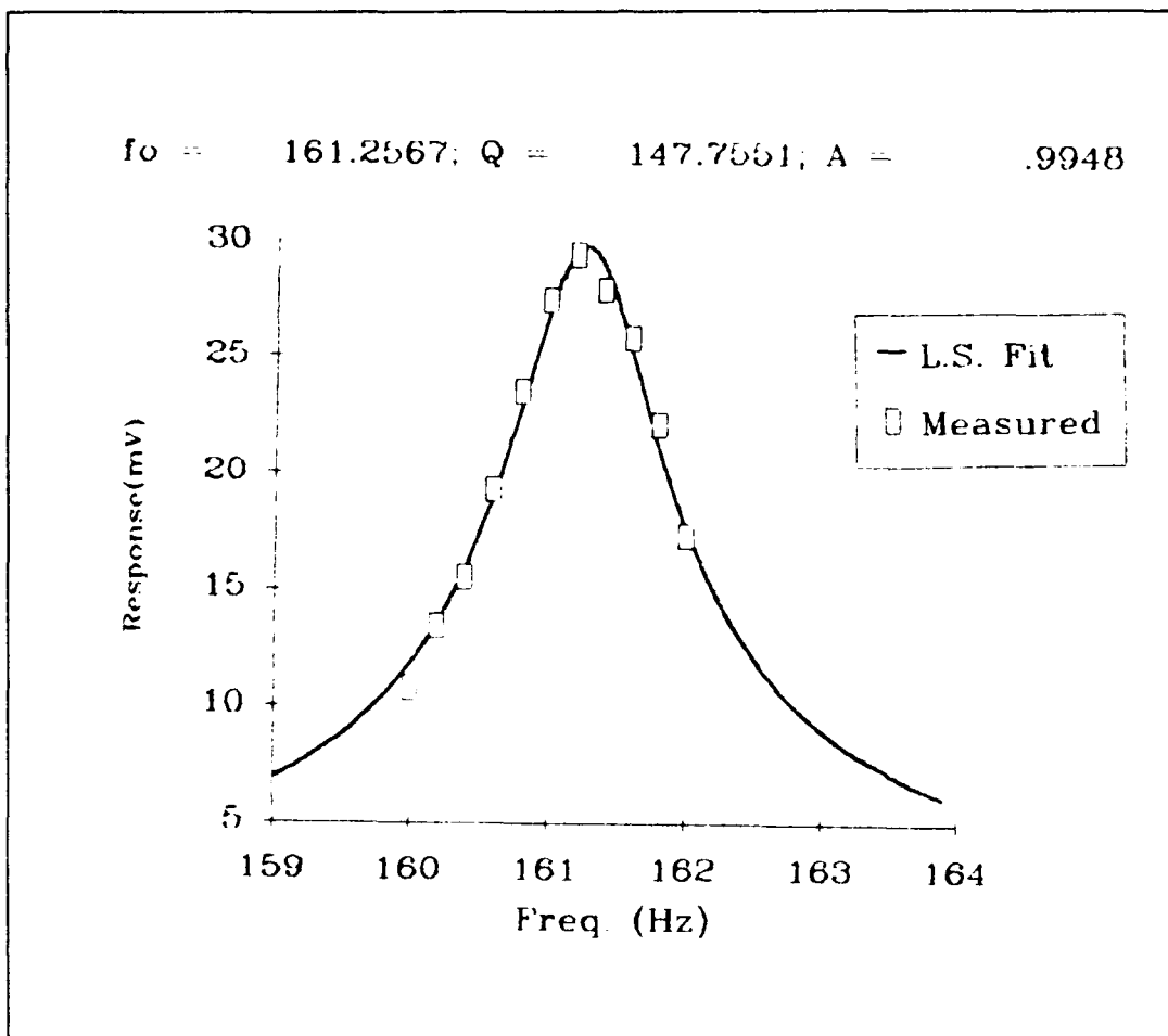
Figure 4. Sample plot of data obtained prior to onset.
