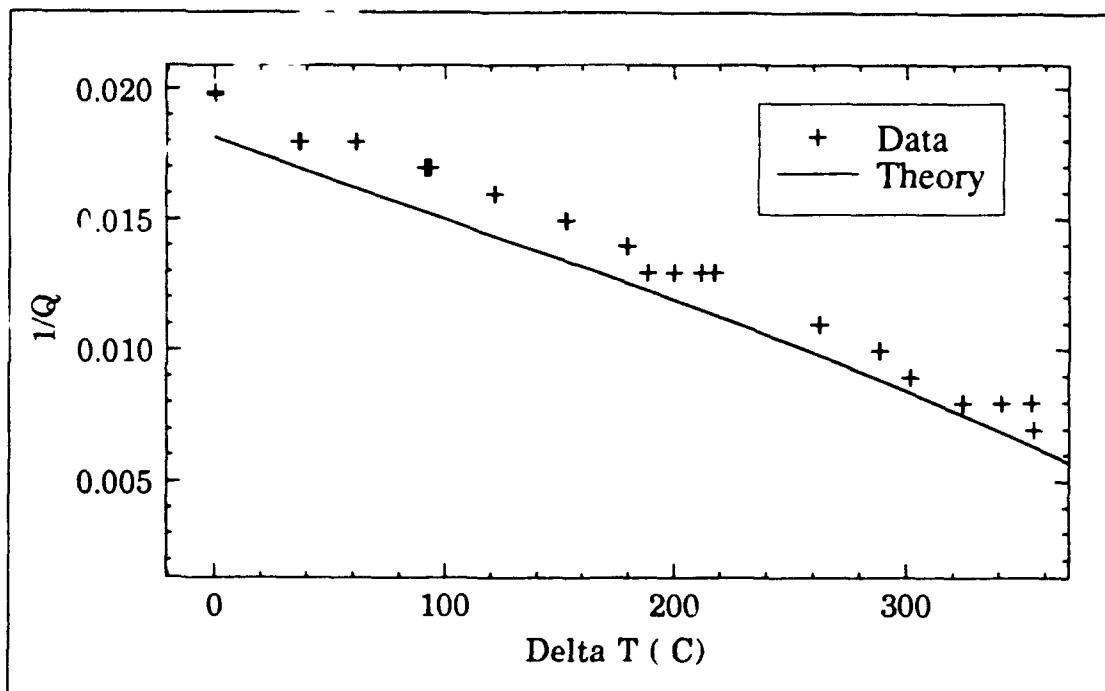
Figure 15. Plot of 1/Q vs \Delta T_m for data obtained below onset in the second mode. P = 205 \text{ kPa} .
