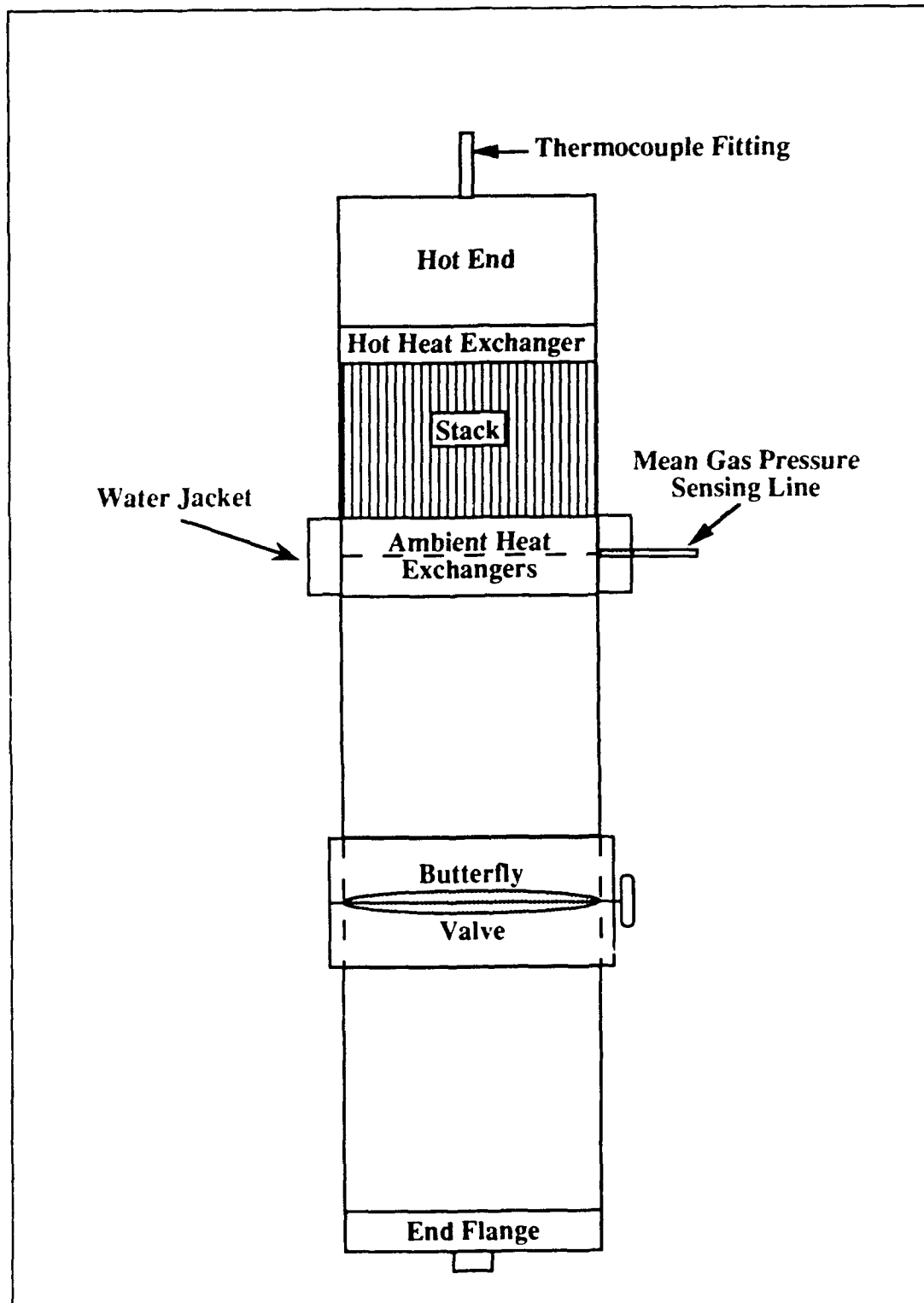
Figure 1. Major components of a prime mover. (Not to scale)
