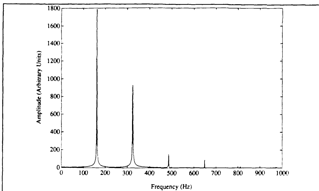
Figure 20. Plot of DFT of data obtained at steady state. P = 80.3 \text{ kPa} . \nabla T_m = 419.8 \text{ }^\circ\text{C} .
