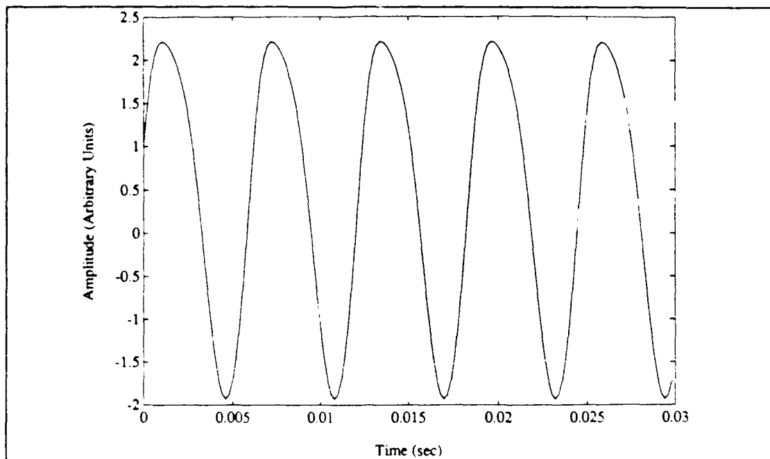
Figure 33. Plot of waveform obtained at steady state. P = 204.8 \text{ kPa} . \Delta T_m = 411.5 \text{ }^\circ\text{C} .
