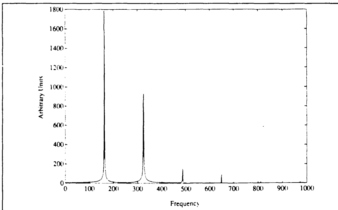
Figure 10. Sample plot of DFT of data collected during steady state.
