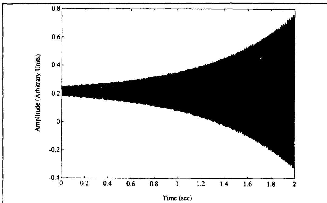
Figure 6. Sample plot of data collected during onset.
