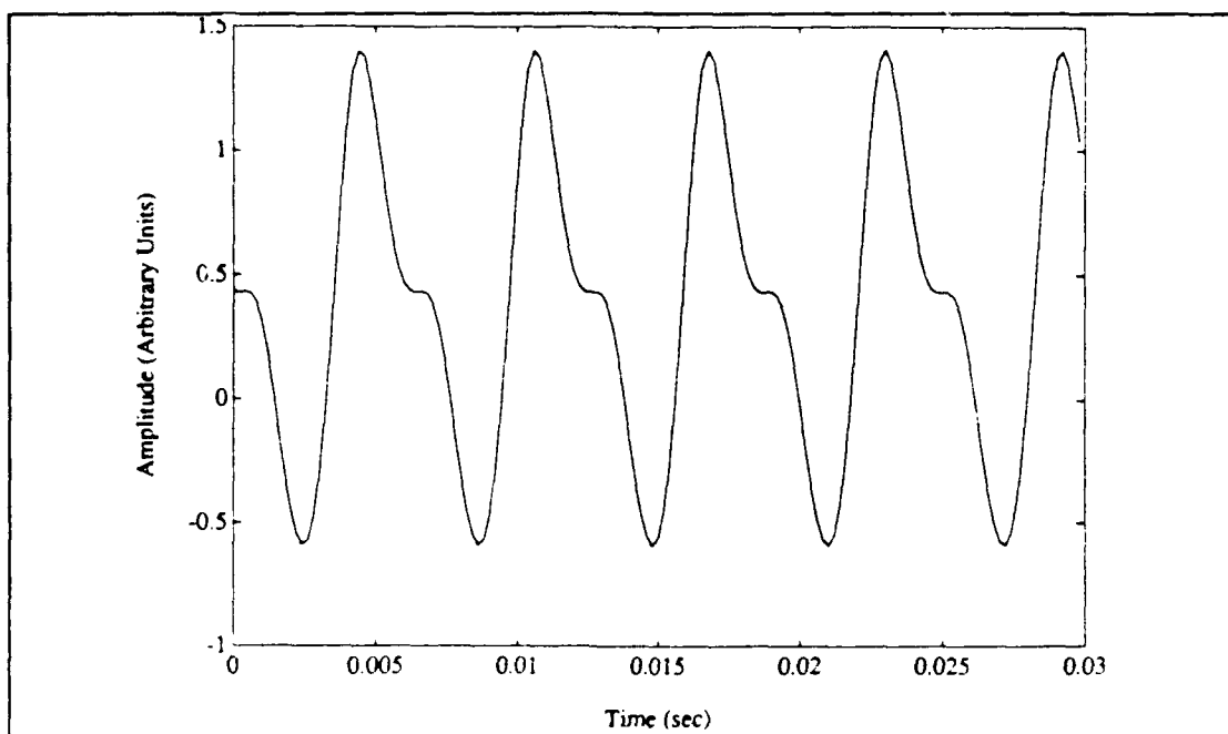
Figure 21. Plot of waveform obtained at steady state. P = 81.1 \text{ kPa} . \Delta T_m = 398.3 \text{ }^\circ\text{C} .
