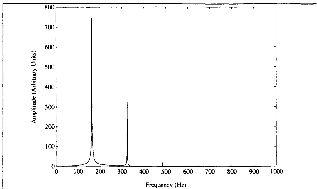
Figure 18. Plot of DFT of data obtained at steady state. P = 80.1 \text{ kPa} . \Delta T_m = 382.8 \text{ }^\circ\text{C} .
