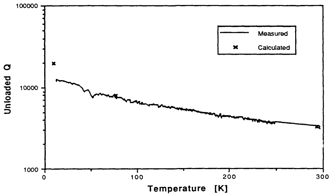
Fig.7 Total unloaded Q of resonator structure using a sample gold-plated OFHC plate.
