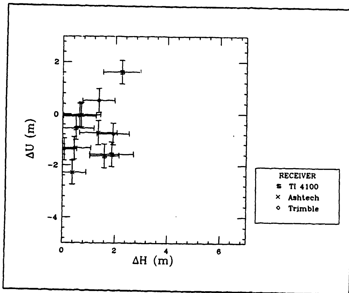
Figure 22. \Delta H_{\text{or}} versus \Delta U_{\text{p}} for Beach Lab, Precise Ephemeris Data
