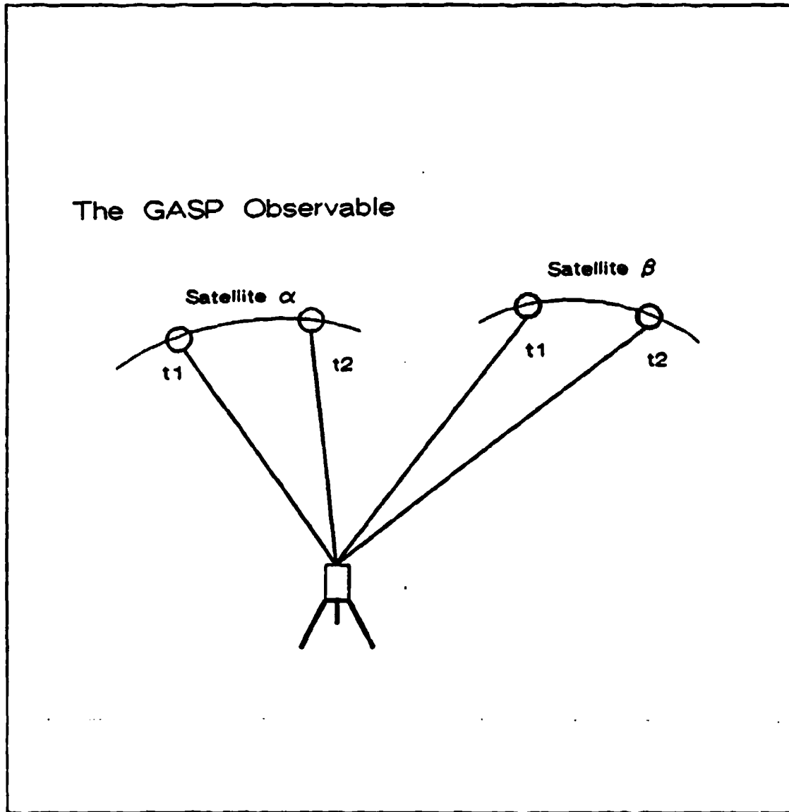
Figure 17. The GASP Observable: Differencing Over Satellites Over Two Consecutive Measurement Epochs
