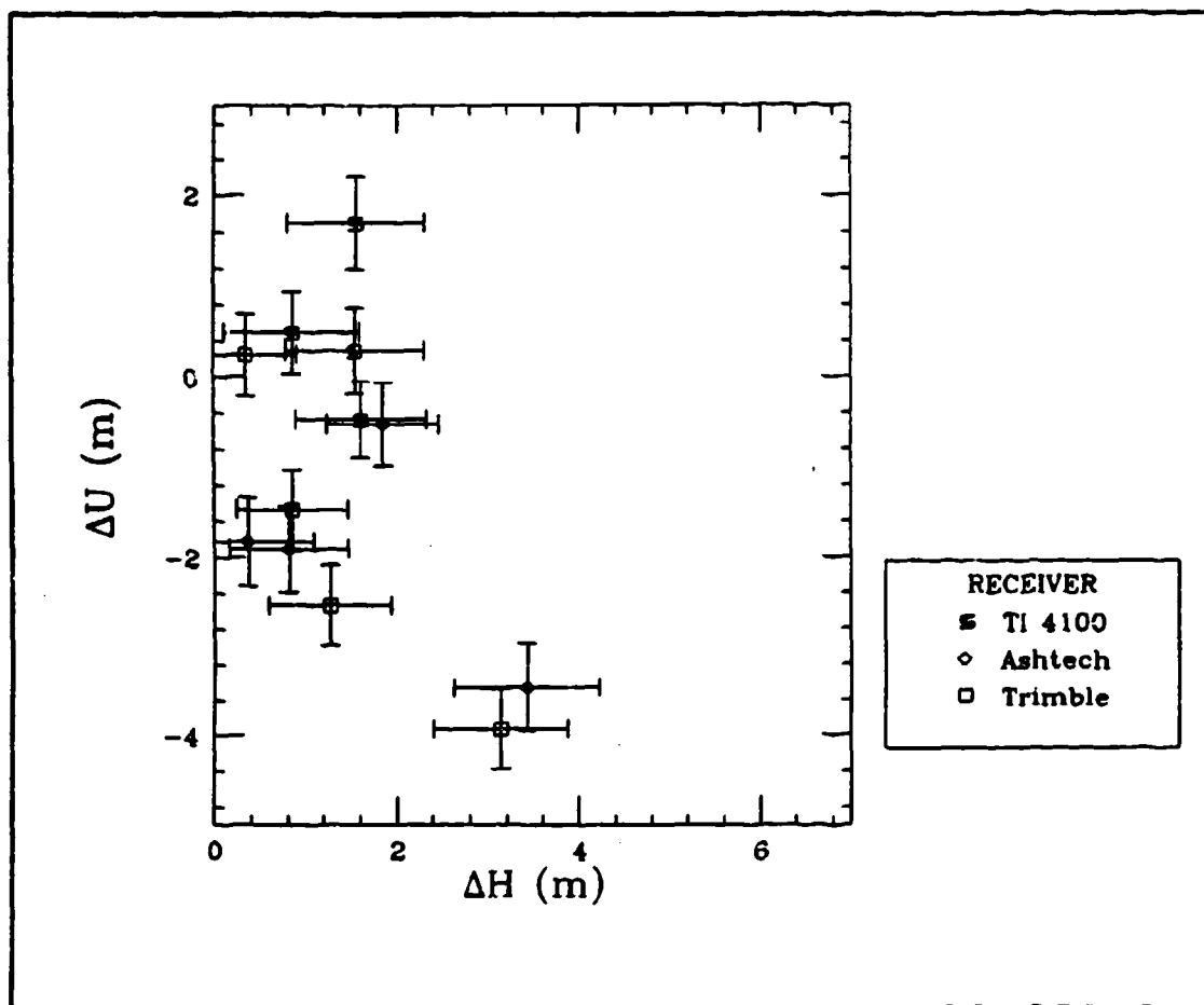
Figure 20. \Delta H versus \Delta U for Beach Lab, Broadcast Ephemeris Data
