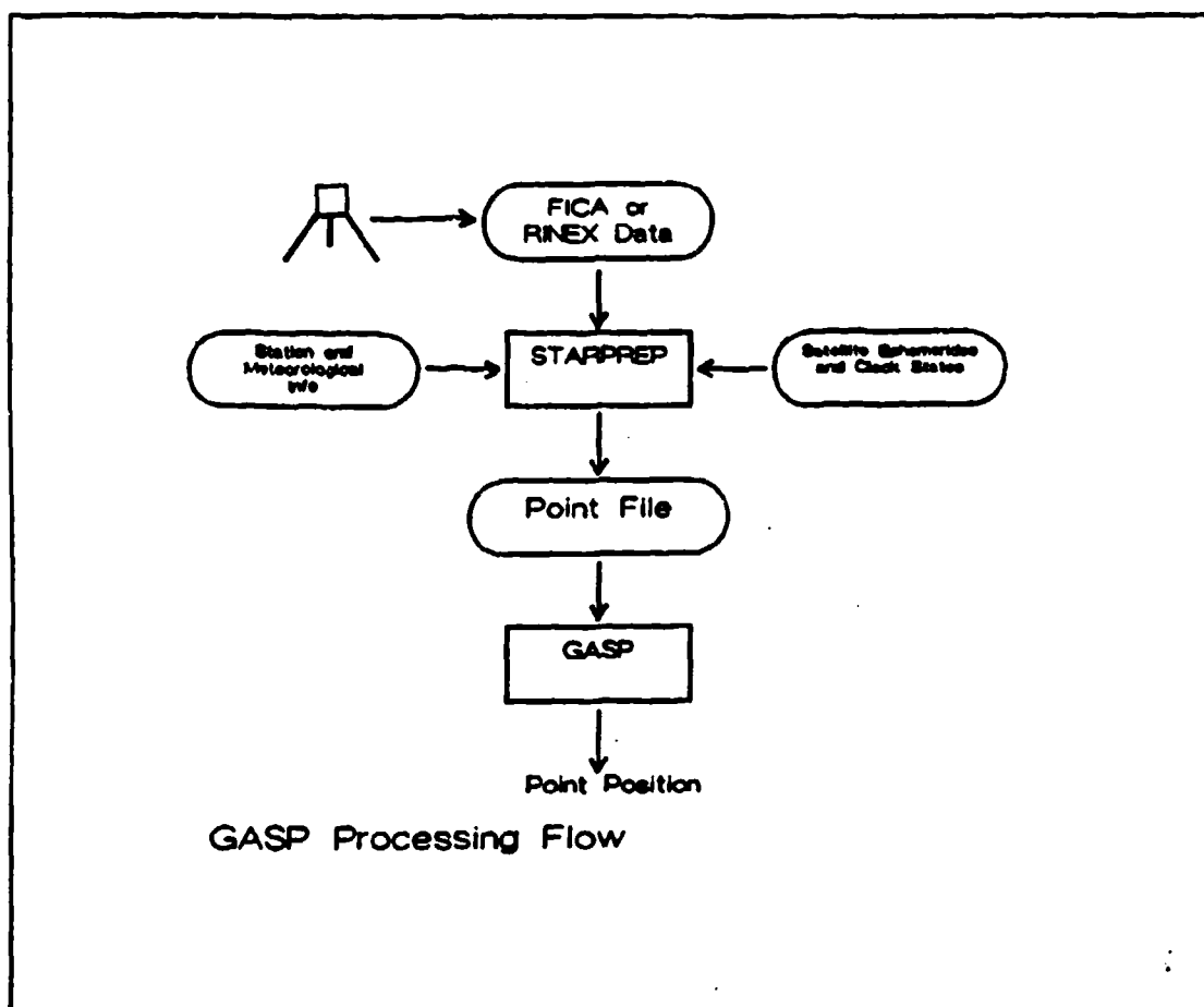
Figure 12. GASP Processing Flow
