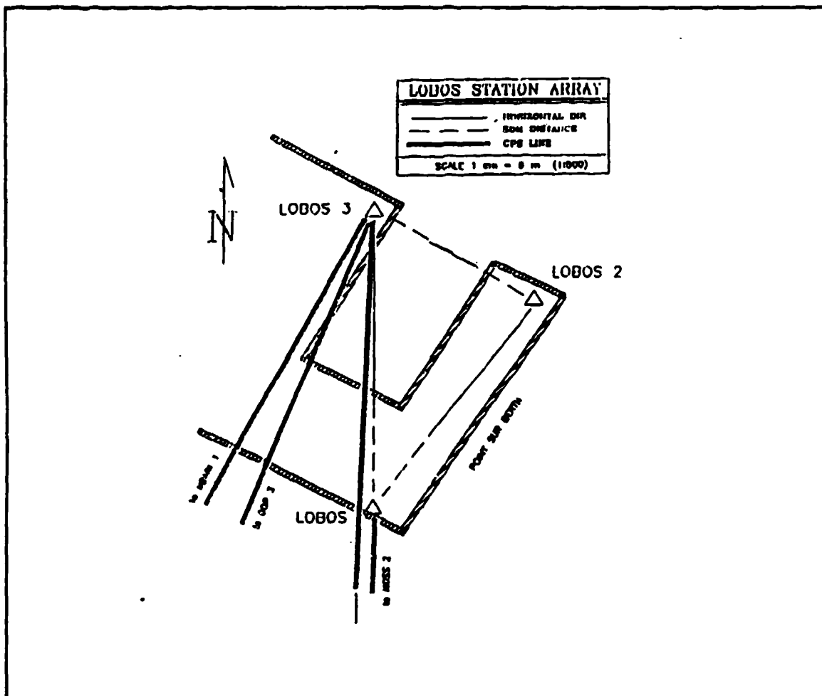
Figure 11. The Lobos Array: The Moss Landing Monument Sites, TI 4100 Receiver Set-up Over LOBOS3
