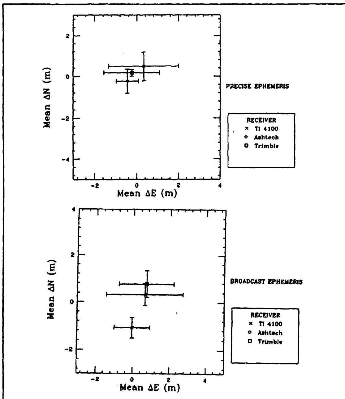
Figure 23. Mean \Delta East versus Mean \Delta North for Beach Lai: Repeatability: Average Over Days by Receiver
