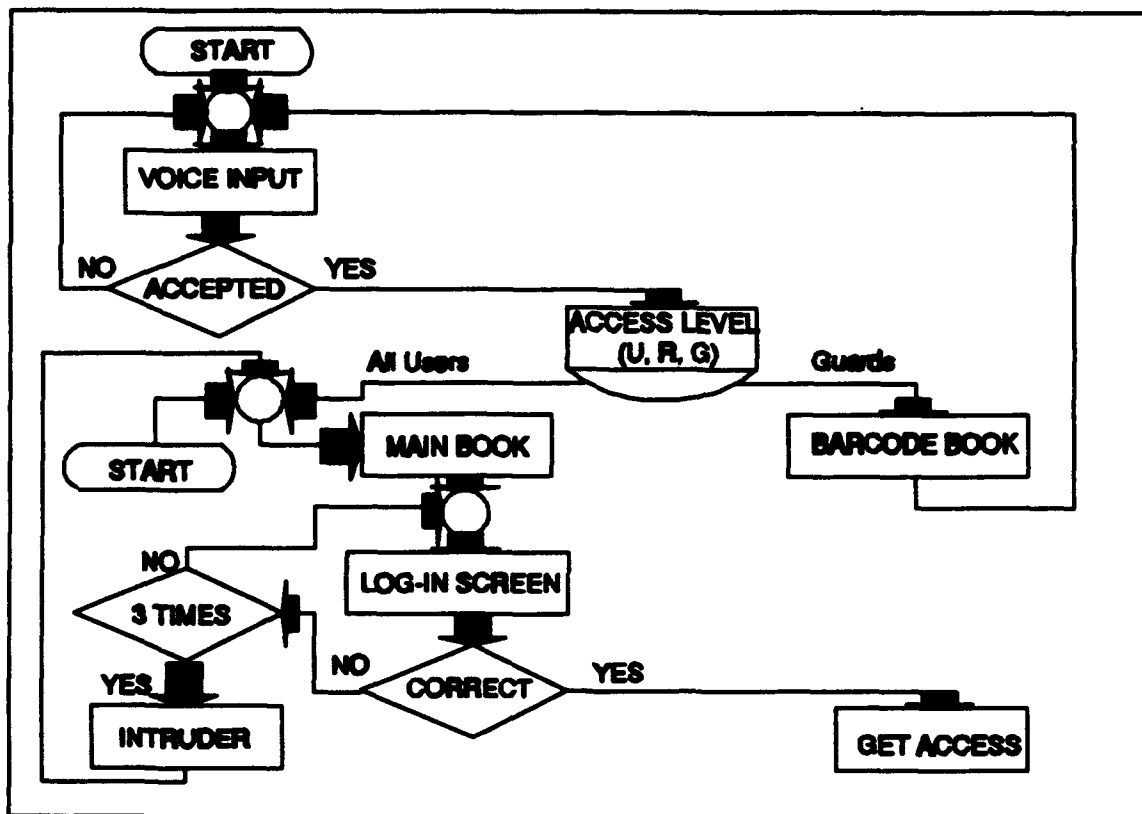
Figure 3.1 Logic Sequence Accessing CCCS Prototype
