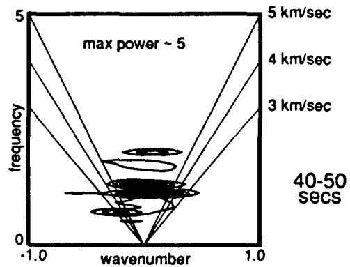
Figure 5: Wavenumber spectra for randomly selected windows of the vertical component for the 2/10/87 event.
