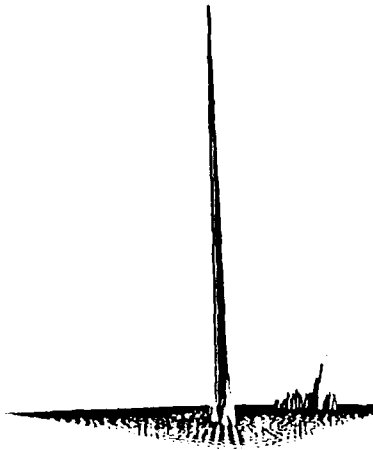
Lorenz equations
