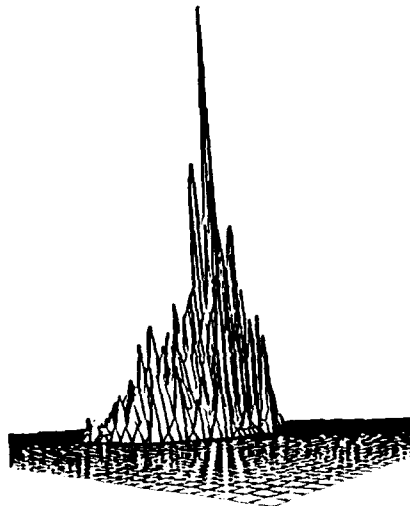
Duffing's equation
