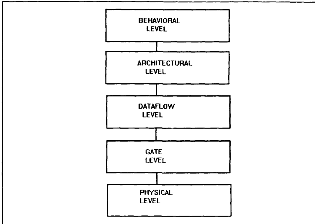
Figure 1 Digital hardware hierarchy
