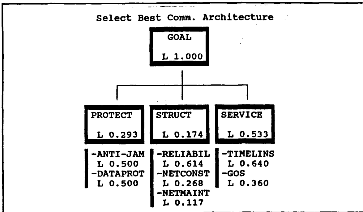
Figure 17. Problem Hierarchy
