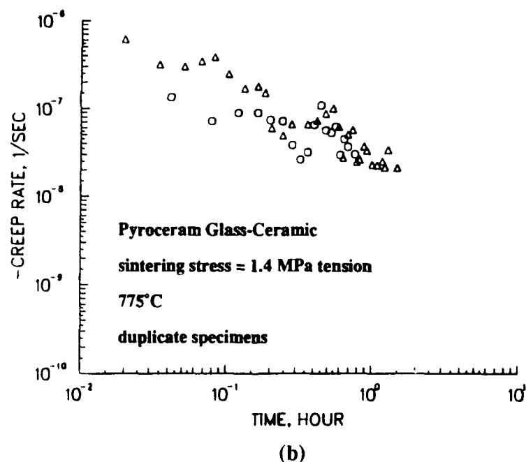
Figure 20. Creep and sintering rates as a function of time: (a) creep rates for MAS glass-ceramic tested at 41 MPa at 775°C, and (b) negative creep rate (contraction rate) as a function of time of sintering at a tensile stress of 1.4 MPa. The pyroceram glass-ceramic specimens were pre-crept at 41 MPa for \approx 16 hours at 775°C.
