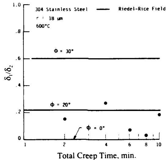
Fig. 9. Comparison of measured and calculated ratios of mode II, \delta_I , to mode I \delta_{II} , crack opening displacement rates as a function of creep time for 304 stainless steel.
