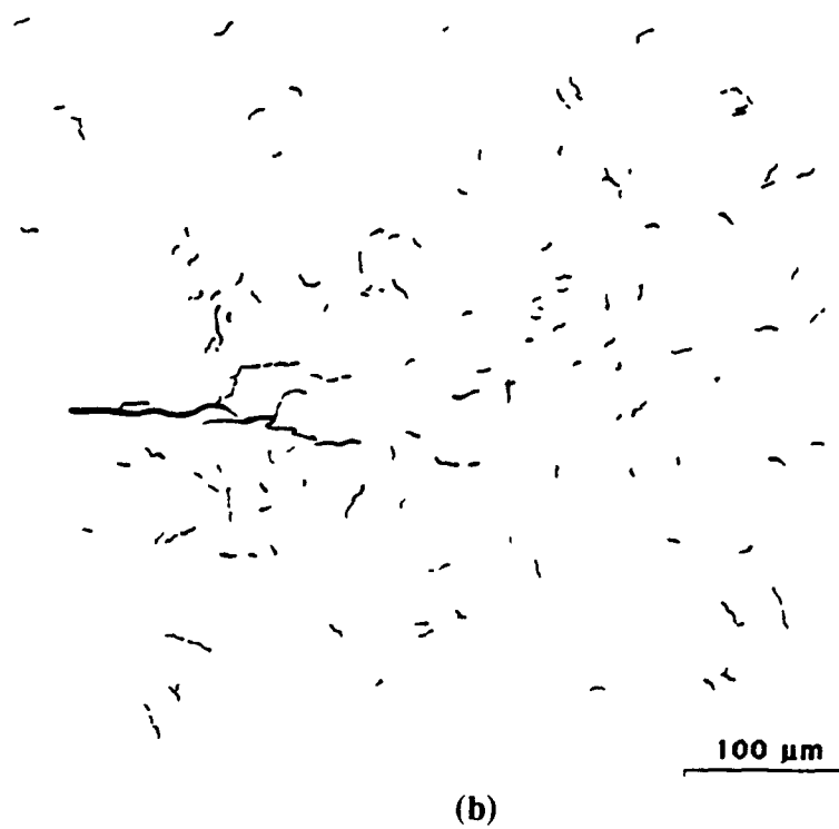
Figure 6. Traces of microcracks located near the tip of dominant creep crack: (a) K = 0.95\sqrt{\text{m}} at 750^{\circ}\text{C} , and (b) K = 0.7\sqrt{\text{m}} at 775^{\circ}\text{C} .
